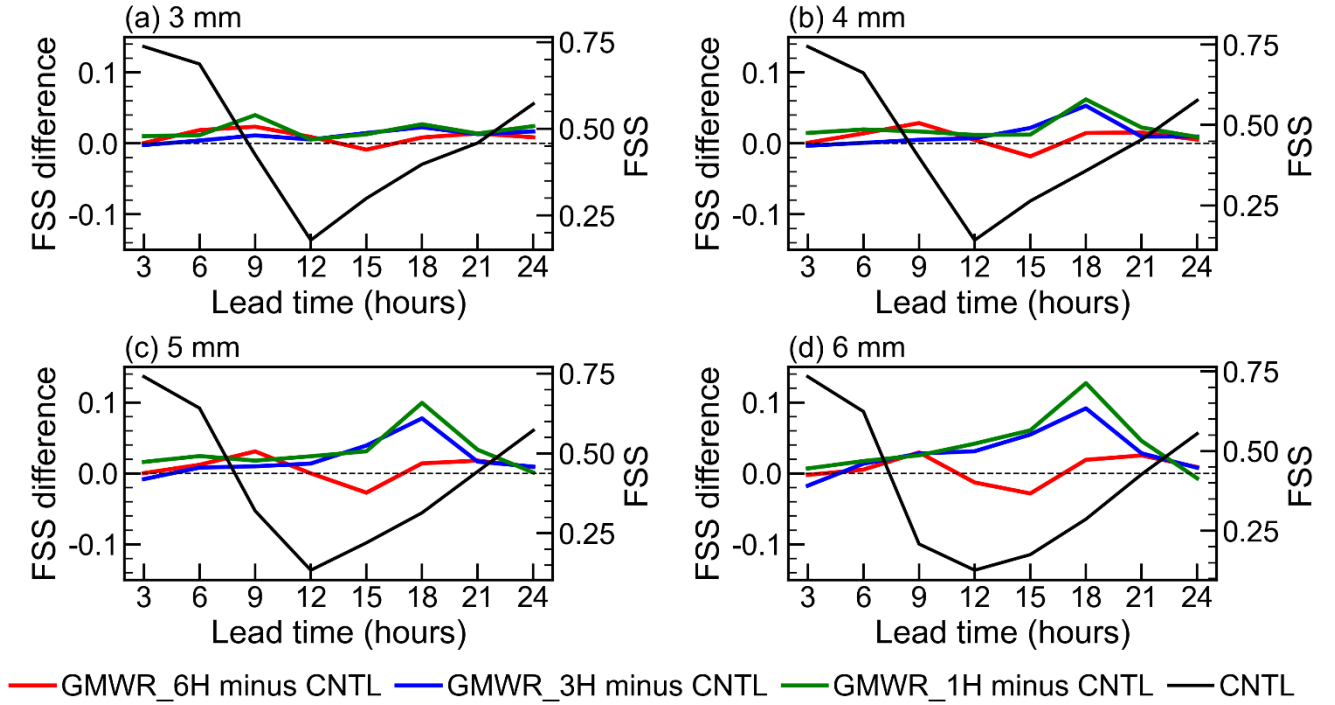
Figure 13. The time series of FSS (black line) for the CNTL experiment and FSS differences (colored lines) between the assimilation experiments and the CNTL experiment. These experiments were conducted from 13 to 22 October 2023. The FSS was calculated for 3 h accumulated precipitation with thresholds of (a) 3 mm, (b) 4 mm, (c) 5 mm, and (d) 6 mm.
