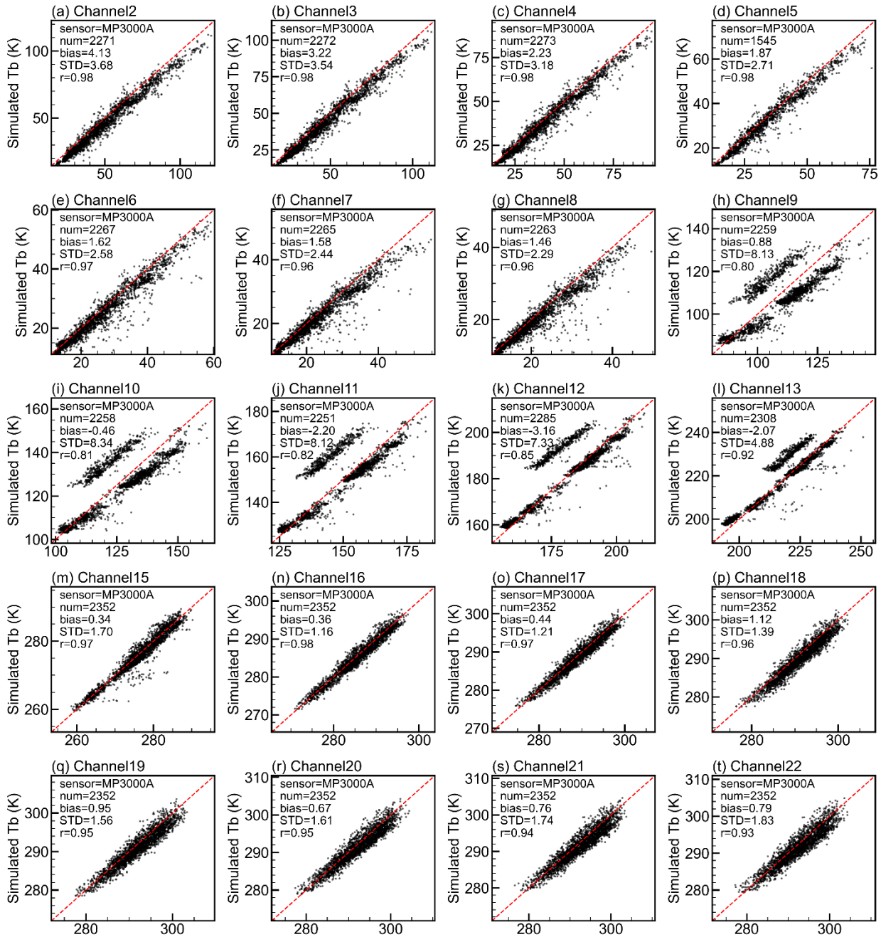
570 Figure A2. Scatterplots of observed brightness temperature (Tb) versus simulated Tb for MP3000A. Same as Fig. 3 but for additional channels.
