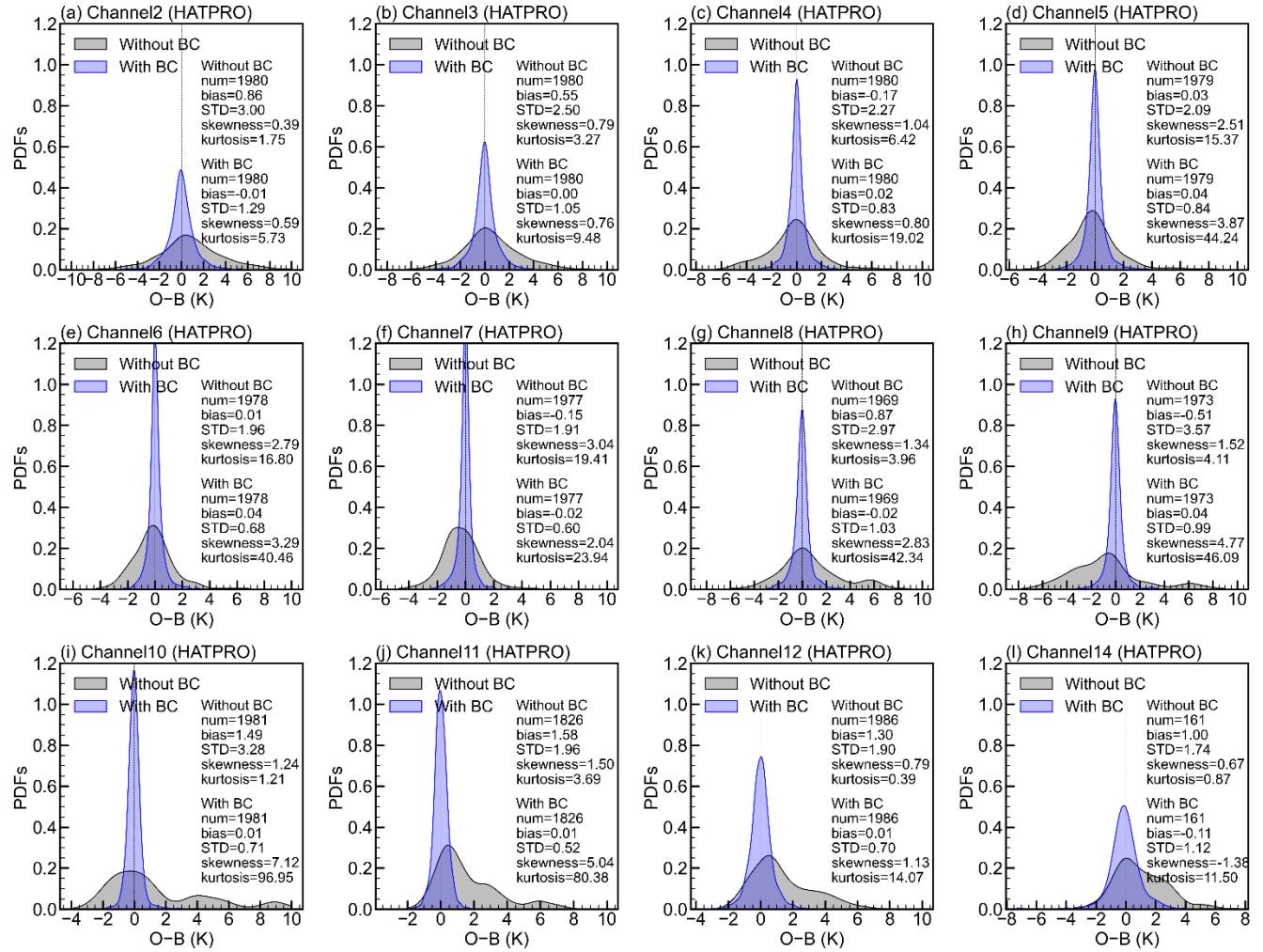
Figure B1. Probability density functions (PDFs) of the O-B distributions for HATPRO. Same as Fig. 6 but for additional
