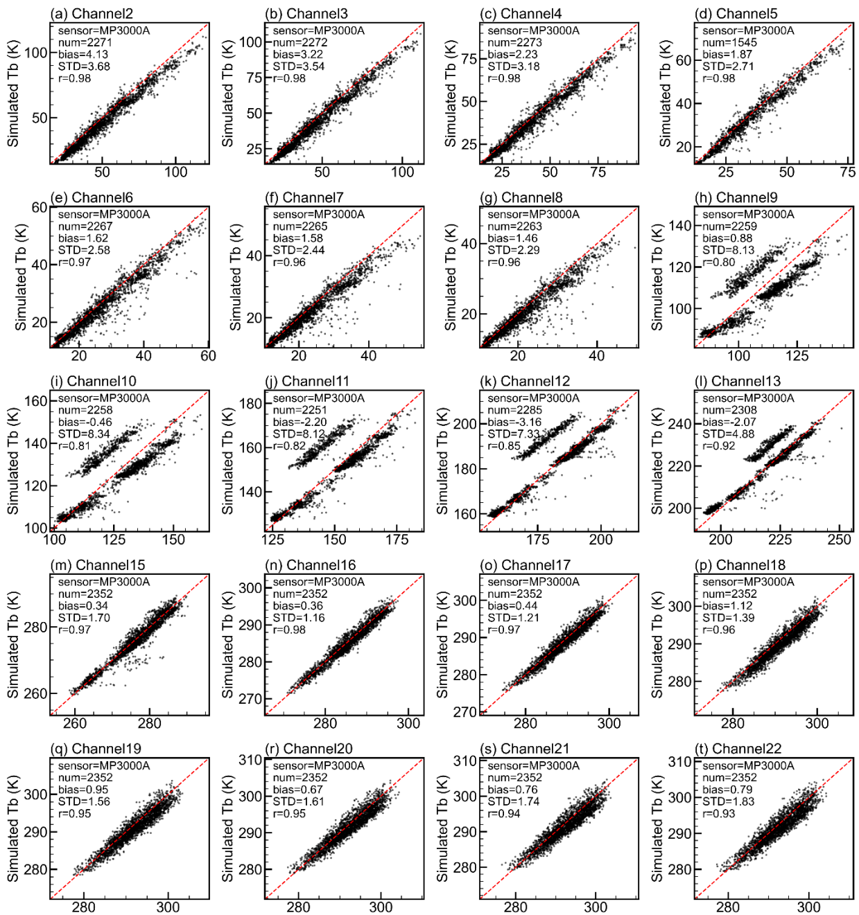
565 Figure A2: Scatter plot of observed brightness temperature (Tb) versus simulated Tb for MP3000A. Same as Fig. 3 but for additional channels.
