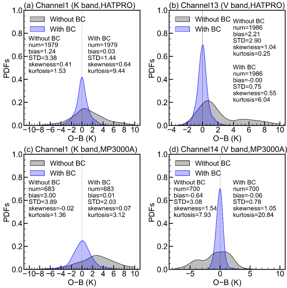
Figure 6: Probability density function (PDF) of the O-B distributions, based on a test set randomly selected from 30% of the three-month sample dataset collected from August to October 2023. The top and bottom rows correspond to the HATPRO and MP3000A sensors, respectively, while the left and right columns represent the K-band and V-band. Each panel displays the number of samples (num), the mean (bias), standard deviation (STD), skewness, and kurtosis of the distributions.
