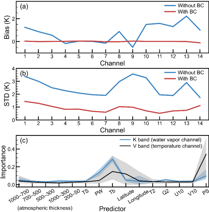
320 Figure 7: (a) Bias and (b) standard deviation (STD) of O–B, based on a test set randomly selected from 30% of the three-month sample dataset collected from August to October 2023. (c) Feature importance of the predictors used in the bias correction (BC) model. The shaded regions and solid lines represent the range and mean feature importance for the K-band and V-band, respectively.
