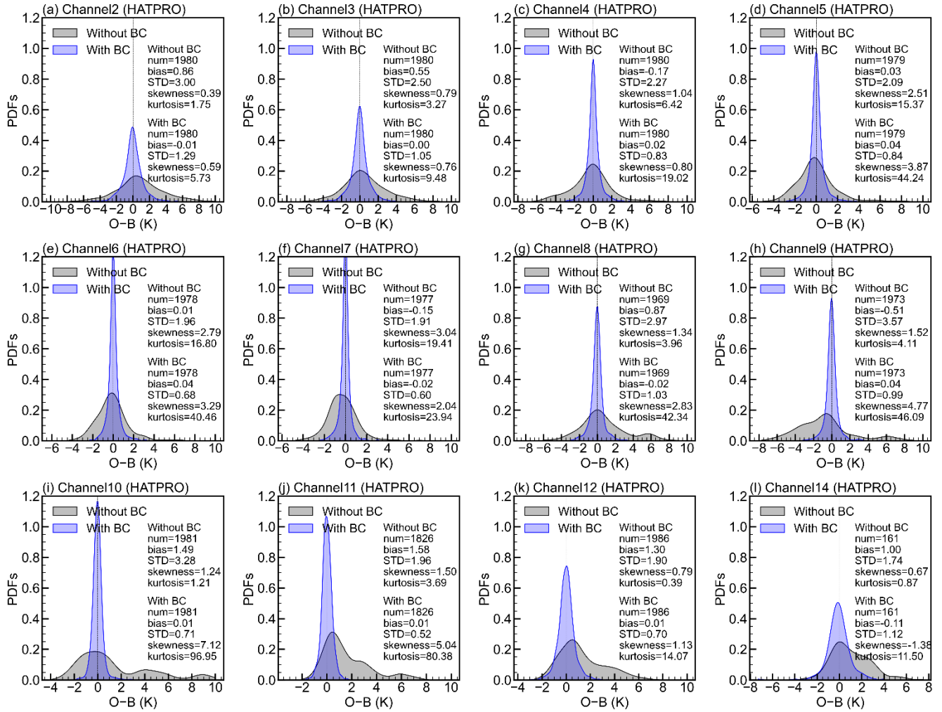
Figure B1: Probability density function (PDF) of the O-B distributions for HATPRO. Same as Fig. 6 but for additional
