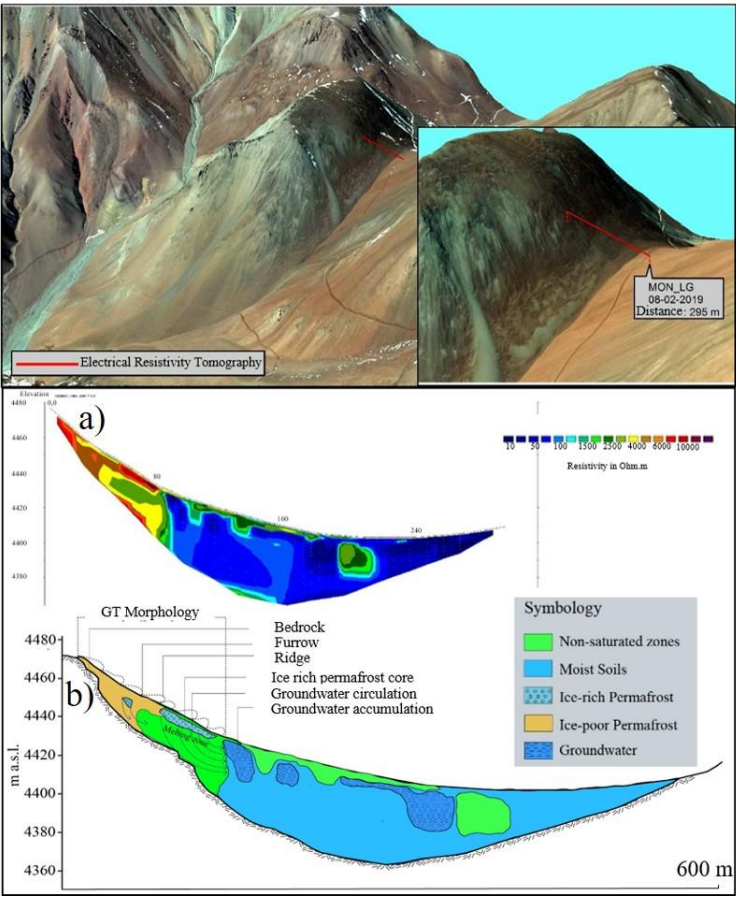
686 687 Figure 13. Results of the electrical resistivity tomography (ERT) over the gelifluction taluses cryospheric landforms in the Montosa 688 Sub-watershed. a) Electrical resistivity tomography, b) Subsurface interpretation of resistivity test. Basemap: Esri, Maxar, 689 Earthstar Geographics, and the GIS User Community.
