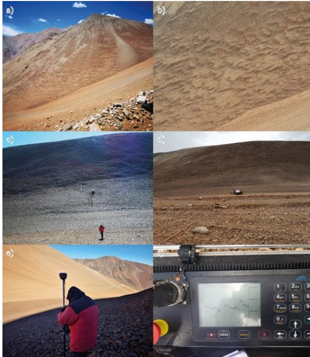
Figure 5. Photography of the fieldwork. a) And b) the Lobulated morphology of studied gelifluction taluses, which are not covered in snow; c) and d) the geoelectric line cable; e) and f) the used equipment, differential GPS and resistivity meter ARES II measuring a resistivity point diagram distribution.
