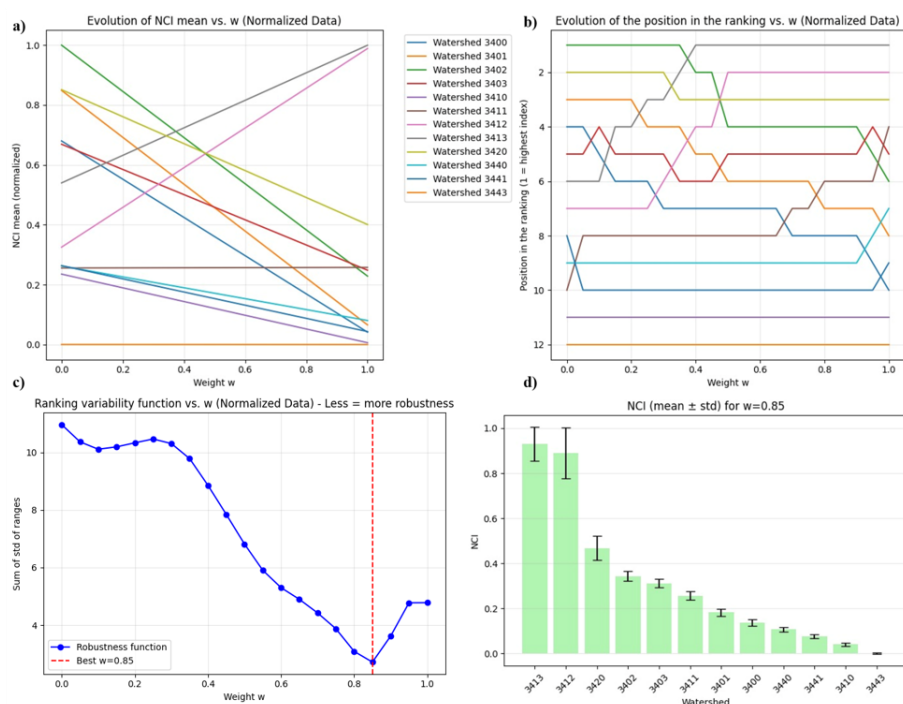
816 817 Figure 19. Analysis of NCI and robustness of the ranking as a function of w weighting (a) Evolution of the mean NCI for each sub- 818 watershed as w varies between 0 and 1 (b) Position in the ranking of each sub-watershed as a function of w (c) Ranking variability 819 function (sum of the standard deviations of the positions), where the minimum at w \approx 0.85 indicates the maximum stability of the 820 ranking (d) Mean NCI \pm standard deviation for w=0.85 , evidencing the magnitude and dispersion of the index in each sub-watershed 821 under the most robust condition.
