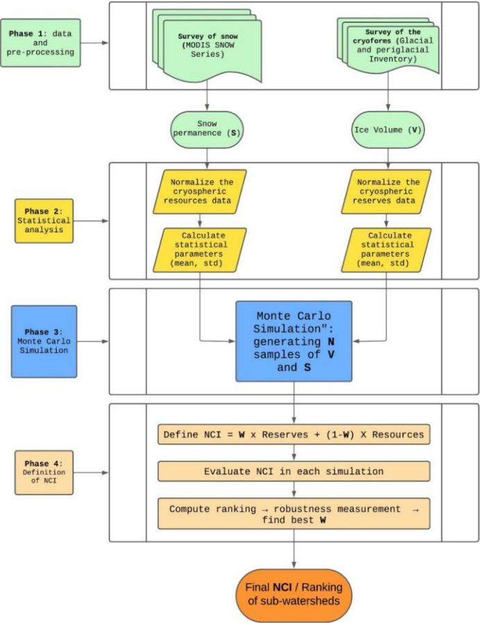
571 572 Figure 7. Flow chart of the methodology used to calculate the NCI.
