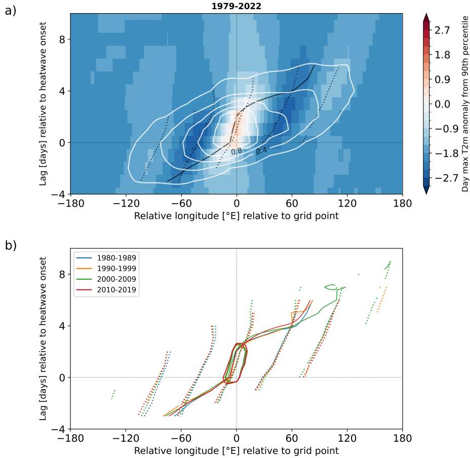
Figure 8. (a) Composite-mean daily-maximum 2 m temperature anomalies with respect to the 90th percentile as in Figure 4a for heatwaves at 50°S from the ERA5 dataset. (b) Contour lines of zero phase angle for the carrier wave (dotted lines) and the wave packet envelope (thin solid lines) with thick solid contours of 0 K composite-mean temperature anomaly as in Fig 4c for the four decades 1980-2019 in ERA5.
