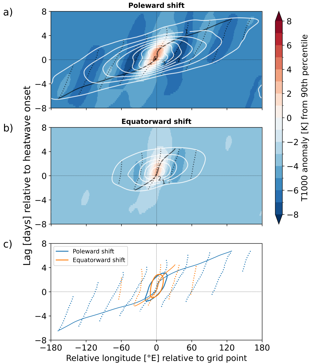
Figure 4. Composite-mean temperature anomaly at 1000 hPa with respect to the 90th percentile at 50°N for heatwaves (a) in experiment exp9 with a poleward storm track shift and (b) in experiment exp4 with an equatorward storm track shift in days relative to the heatwave onset (y-axis) and longitude relative to the grid point where the heatwave is identified (x-axis). White contours indicate the strength of the wave packet envelope in units of K. Dashed black lines indicate contours of zero phase angle for the carrier wave, while the solid black lines indicate a constant phase angle of the wave packet envelope. The lines of constant phase angle for both experiments shown in (a) and (b) are plotted for comparison in (c) with the solid contour of 0 K composite-mean temperature anomaly.
