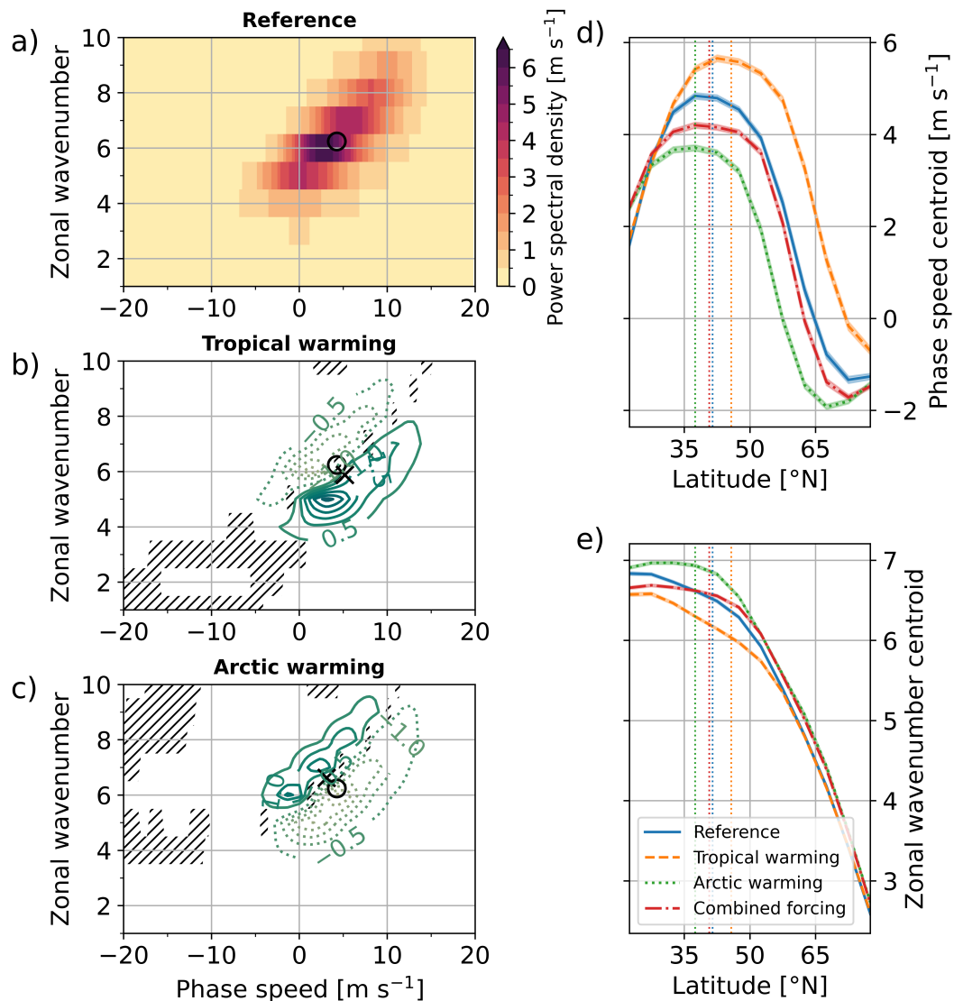
Figure 2. Climatological-mean meridional-mean (35°N to 65°N) power spectral density of meridional wind at 250 hPa for (a) the reference simulation and (b)-(c) the difference in the experiments with tropical and Arctic warming, respectively. The circle indicates the centroid of the meridional-mean spectrum for the reference simulation, the 'x' markers indicate the centroid for the respective sensitivity experiment. Hatching indicates where the spectrum of the reference simulation and the sensitivity experiment are not significantly different at the 99.9% confidence level based on a parametric bootstrap of 14-day windows. The centroid of (d) phase speed spectra and (e) zonal wavenumber spectra averaged over smaller 5°N latitude band widths is plotted as a function of central latitude with the 95% confidence interval (shading). The dotted vertical lines in (d)-(e) indicate the location of the maximum eddy kinetic energy.
