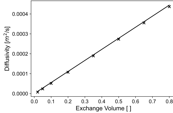
Figure A2. Correlation of the diffusivity and the exchange volume. The black crosses represent the diffusivities for the given exchange volumes and time steps (compare Table A1). The black line represents Eq. A4.
