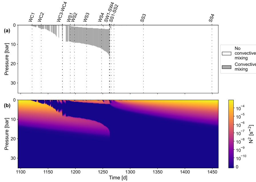
Figure A4. Similar to Fig. 5 but with an exchange volume of \nu = 0.05 and the 22nd year shown.
