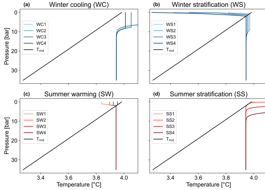
Figure A3. Similar to Fig. 4 but with an exchange volume of \nu = 0.05 and the 22nd year shown.
