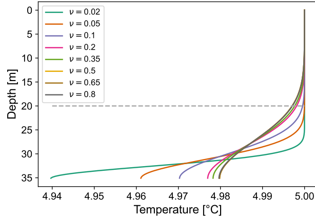
Figure A1. Temperature profiles for different applied exchange volumes at different time steps. The simulation setup is described in the text. The shown time steps for the corresponding exchange volumes are listed in Table A1. The gray dashed line indicates the depth at which the diffusivity values were evaluated.
