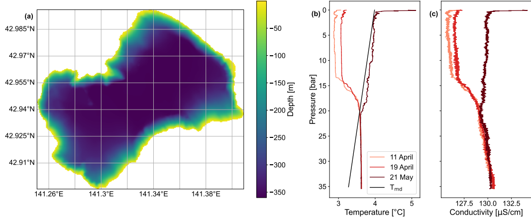
Figure 1. Bathymetry, potential temperature and conductivity profiles from 2005 of Lake Shikotsu. (a) presents the bathymetry map of Lake Shikotsu (created by editing GSI (Geospatial Information Authority of Japan) Tiles ( https://cyberjapandata.gsi.go.jp/xyz/lake1/z/x/y.png )), (b) shows potential temperature profiles and the temperature of maximum density T_{md} , and (c) conductivity profiles from 2005 (data from Boehrer et al., 2008, 2009).
