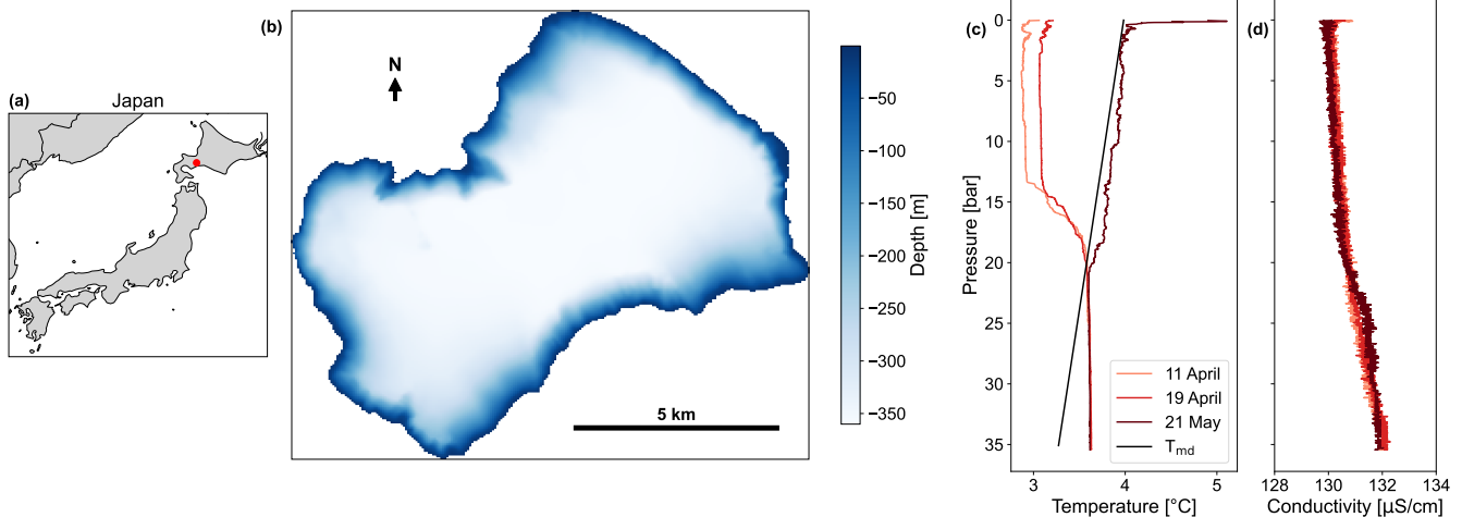
Figure 1. Bathymetry , Location , bathymetry , potential temperature , and conductivity profiles from 2005 of Lake Shikotsu. (a) shows the location of Lake Shikotsu in Japan (red dot) , (b) presents the bathymetry map of Lake Shikotsu (created by editing GSI (Geospatial Information Authority of Japan) Tiles ( https://cyberjapandata.gsi.go.jp/xyz/lake1/z/x/y.png )) , (b) (c) shows potential temperature profiles from 2005 and the temperature of maximum density T_{md} , and (e) (d) electrical conductivity profiles from 2005—normalized to 4 °C (compare Boehrer et al., 2009) for the same dates as in (c) (data from Boehrer et al., 2008, 2009).
