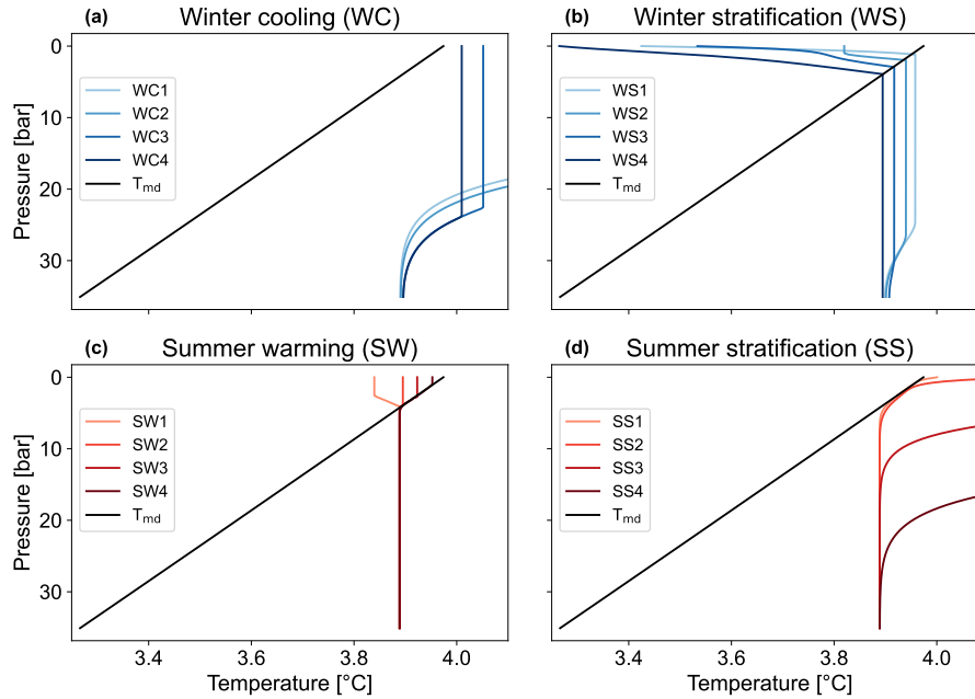
Figure B1. Similar to Fig. 4 but using the density formulation of TEOS-10.
