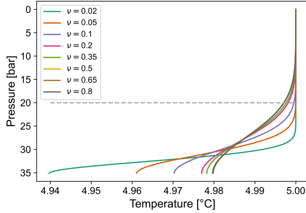
Figure A1. Temperature profiles for different applied exchange volumes-fractions at different time steps. The simulation setup is described in the text. The shown time steps for the corresponding exchange volumes-fractions are listed in Table A1. The gray dashed line indicates the depth at which the diffusivity values were evaluated.
