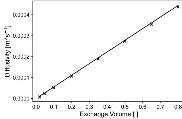
Figure A2. Correlation of the diffusivity and the exchange volume-fraction . The black crosses represent the diffusivities for the given exchange volumes-fractions and time steps (compare Table A1). The black line represents Eq. A4.
