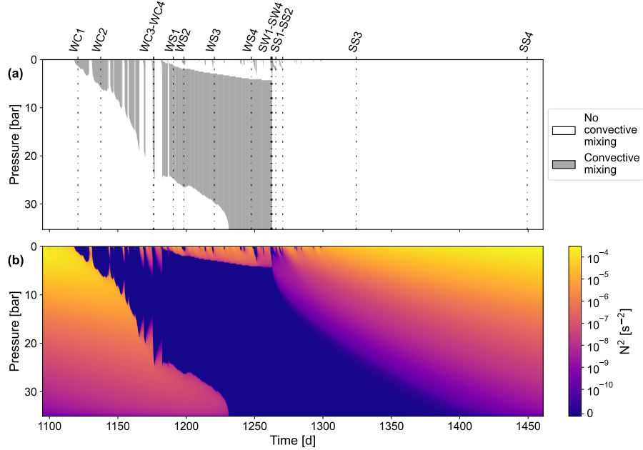
Figure 5. Convective mixing cells and stability of the fourth year of the simulation period. (a) shows the convective mixing cells and the points in time of the profiles shown in Fig. 4 are marked with dash-dotted lines. (b) depicts the corresponding Brunt-Väisälä frequency, calculated with Eq. (6).
