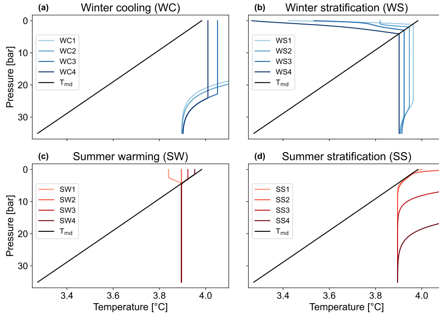
Figure 4. Temperature profiles of the fourth year of the simulation period. The selected temperature profiles are split into four plots for clarity. (a) contains profiles from the winter cooling (WC) phase, (b) from the winter stratification (WS) phase, (c) from the summer warming (SW) phase, and (d) from the summer stratification (SS) phase. Their points in time are marked in Fig. 5. Additionally, all plots include the temperature of maximum density T_{md} .
