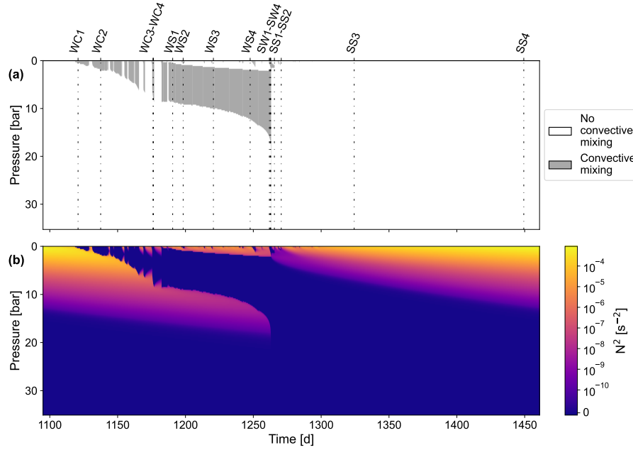
Figure A4. Similar to Fig. 5 but with an exchange volume fraction of \nu = 0.05 and the 22nd year shown.
