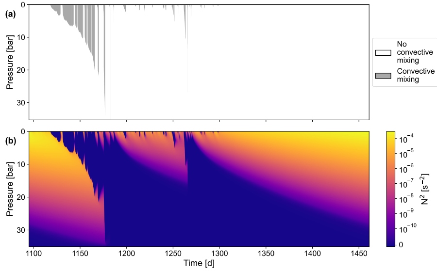
Figure 6. Convective mixing cells and stability of the fourth year of the simulation period for the simulation using potential density \rho_{\text{pot}} instead of in situ density \rho_{\text{in-situ}} (compare Fig. 5). (a) shows the convective mixing cells and (b) depicts the corresponding Brunt-Väisälä frequency, calculated with Eq. (6).
