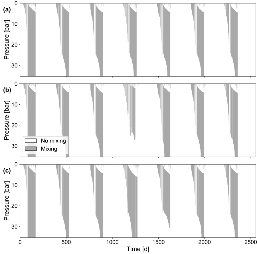
Figure 7. Mixing cells over the entire simulation period for three variants of surface temperature input. The surface temperature of the fourth year of the simulation period was (a) not modified, modified by (b) +0.4\text{ }^{\circ}\text{C} , and (c) -0.4\text{ }^{\circ}\text{C} .
