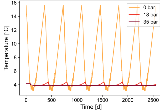
Figure 3. Temperature logs at different depths. The logs show the temperature progression of the controlled surface temperature (0 bar) and at depths of 18 and 35 bar over the entire simulation period.
