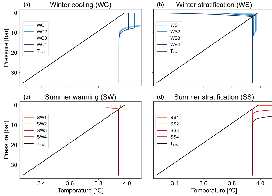
Figure A3. Similar to Fig. 4 but with an exchange volume fraction of \nu = 0.05 and the 22nd year shown.
