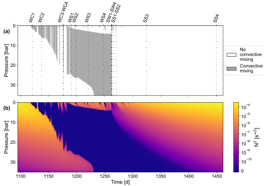
Figure B2. Similar to Fig. 5 but using the density formulation of TEOS-10.
