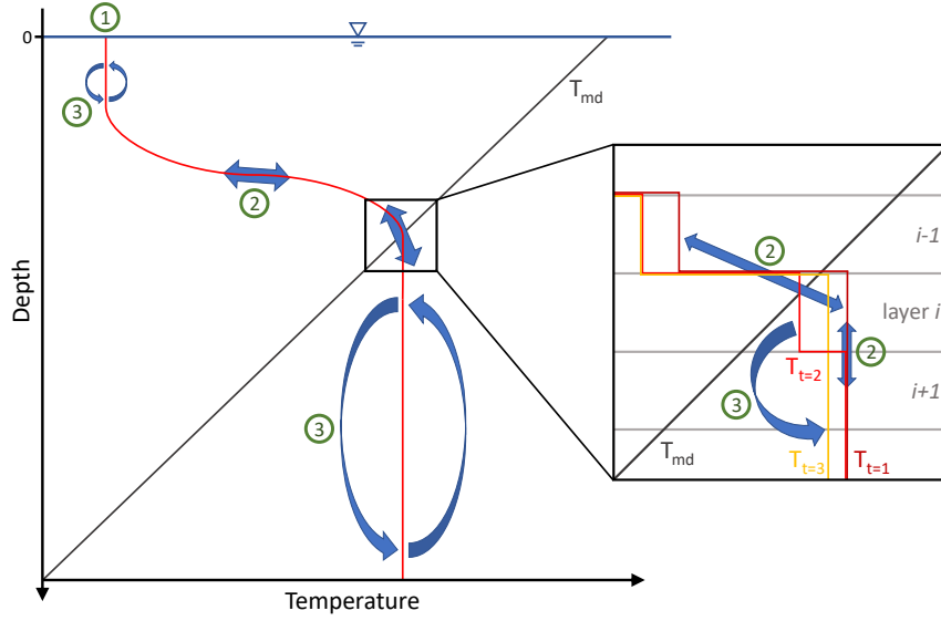
Figure 2. Model processes operating on an exemplary winter temperature profile during one time step. The processes of controlling the surface temperature (1), turbulent diffusion (2), and mixing due to instability (3) are numbered in the order they occur. The zoomed in window shows the temperature profile at the intersection with the T_{md} line between (1) and (2): T_{t=1} , (2) and (3): T_{t=2} , and after (3): T_{t=3} . For a detailed description see the text.
