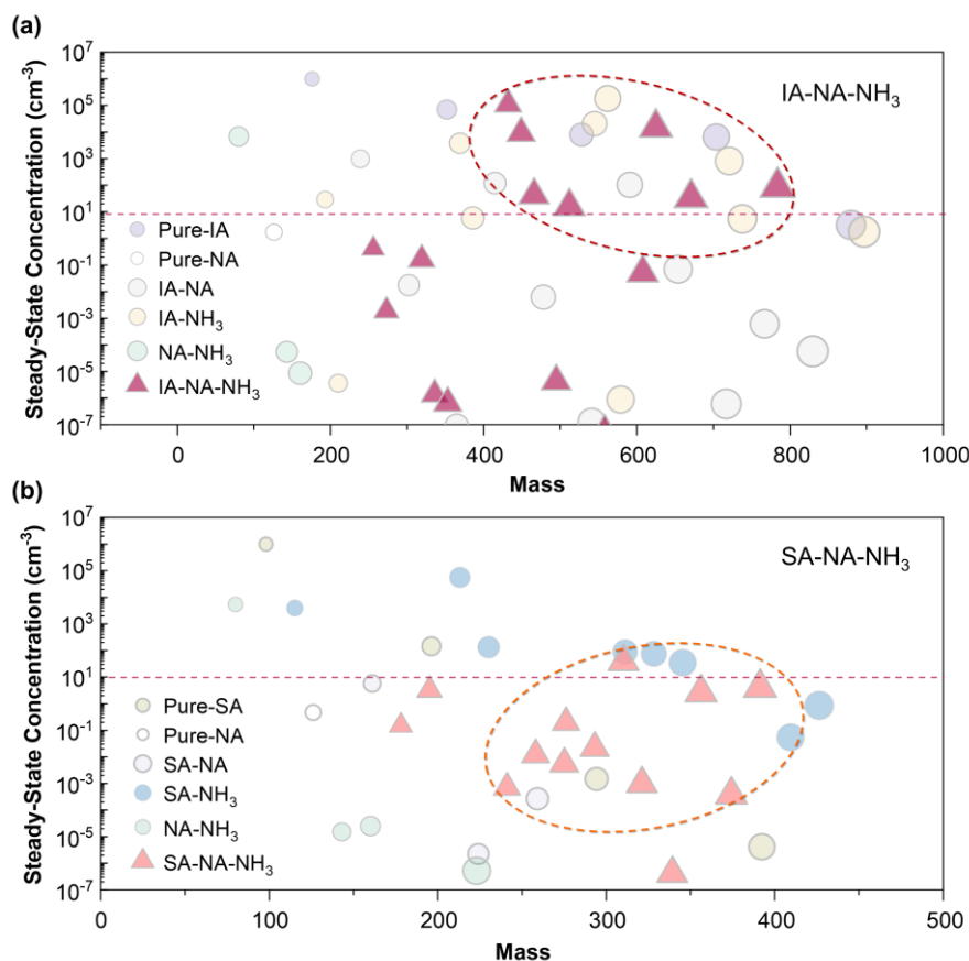
Figure 6. Simulated steady-state concentrations ( \text{cm}^{-3} ) of (a) IA-NA-NH 3 and (b) SA-NA-NH 3 clusters against cluster mass at the conditions of T = 220 K, \text{CS} = 10^{-4} \text{ s}^{-1} , [\text{IA}] = 10^6 \text{ molec. cm}^{-3} , [\text{SA}] = 10^6 \text{ molec. cm}^{-3} , [\text{NA}] = 10^9 \text{ molec. cm}^{-3} , and [\text{NH}_3] = 3 \times 10^8 \text{ molec. cm}^{-3} . For better clarify, the concentrations of ternary clusters in the IA-NA-NH 3 and SA-NA-NH 3 systems are highlighted with circles, respectively.
