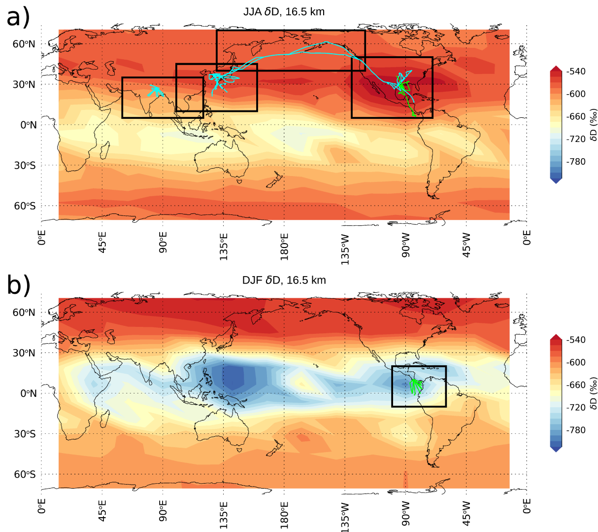
Figure 1. ACE-FTS retrievals of \delta D at 16.5 km altitude during the (a) boreal summer months (JJA) and (b) boreal winter months (DJF). Superimposed on both contour plots are the flights tracks of the ChiWIS instrument (cyan) and the Harvard ICOS/Hoxotope instruments (lime green). The black boxes show the spatial boundaries within which ACE-FTS occultations are collected for comparison to the relevant field campaign. Latitude-longitude range of each box is listed in Table 1.
