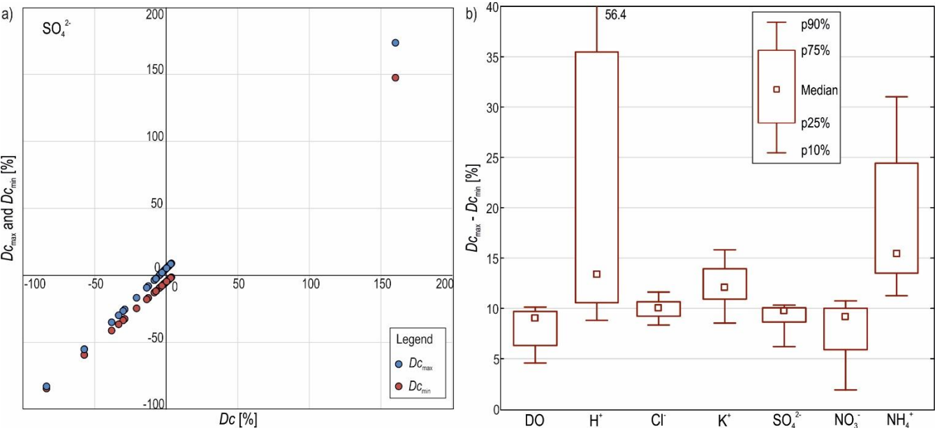
765 Figure A1. The lowest ( Dc_{min} ) and highest ( Dc_{max} ) possible Dc values, taking into account the percent relative errors of the chemical analysis, using the difference in SO_4^{2-} concentration in pond water and stream water above the ponds as an example (a). The differences between the lowest ( Dc_{min} ) and highest ( Dc_{max} ) possible Dc values for the selected chemical parameters are shown in (b).
