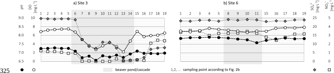
Figure 5: A longitudinal profile of the selected physico-chemical parameters at an overflowing and old site (Site 3 – a), and an in-channel and young site (Site 6 – b) on 10 September 2023.
