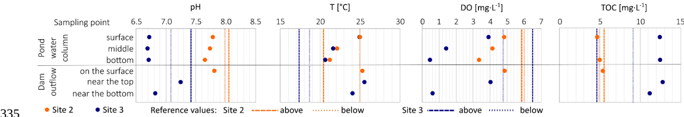
Figure 6: Average values of the selected physico-chemical parameters in the vertical profiles of study sites 2 (in-channel, moderately old) and 3 (overflowing, old) on 10 July 2024.
