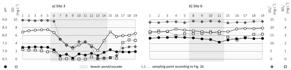
Figure 56: A longitudinal profile of the selected physico-chemical parameters at an overflowing and old site (Site 3 – a), and an in-channel and young site (Site 6 – b) on 10 September 2023.
