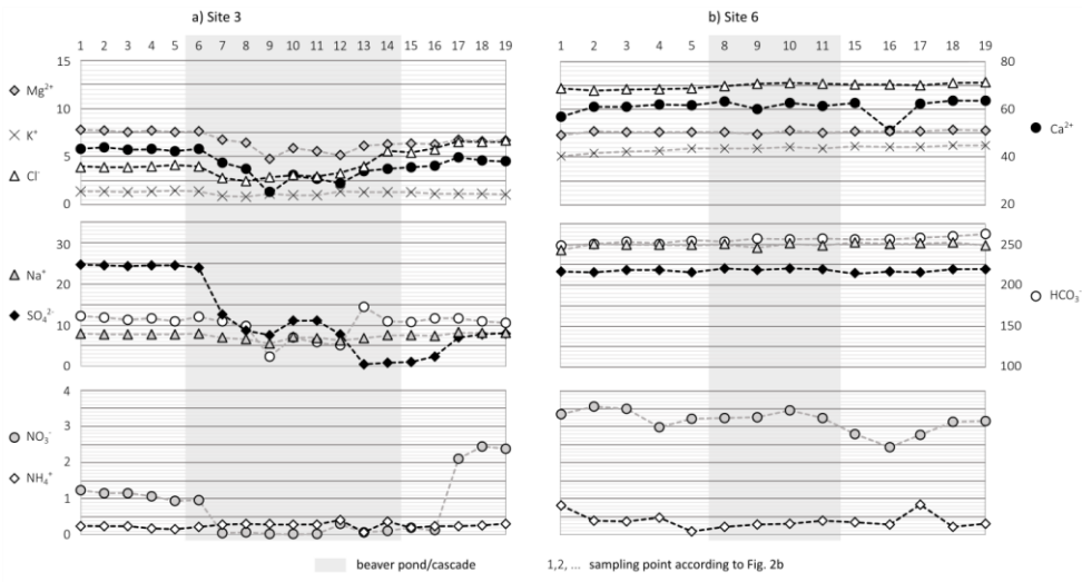
Figure B1: Concentrations of the chemical components of water [ \text{mg}\cdot\text{L}^{-1} ] in the longitudinal stream profiles at study sites 3 (a) and 6 (b) on 10 September 2023.
