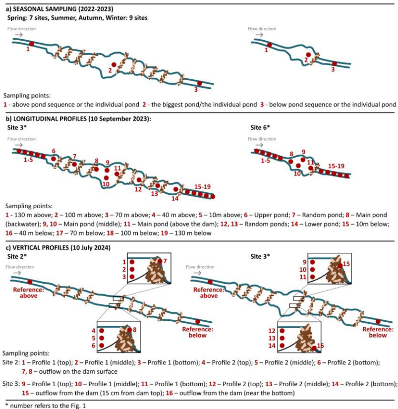
Figure 2: Study sampling schemes.
