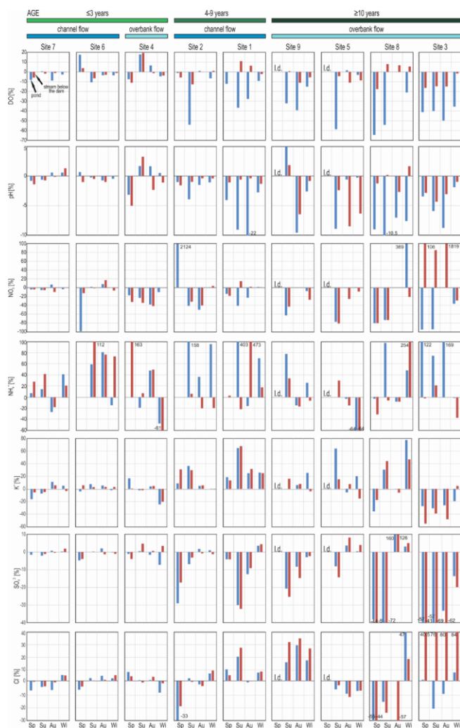
Figure A42: Percentage changes ( D_c ) in selected physico-chemical parameters main ion concentrations in and below beaver ponds compared to their upstream values (Sp – spring; Su – summer; Au – autumn; Wi – winter; l.d. – lack of data). Only the parameters for which |D_c| > 15\% are shown.
