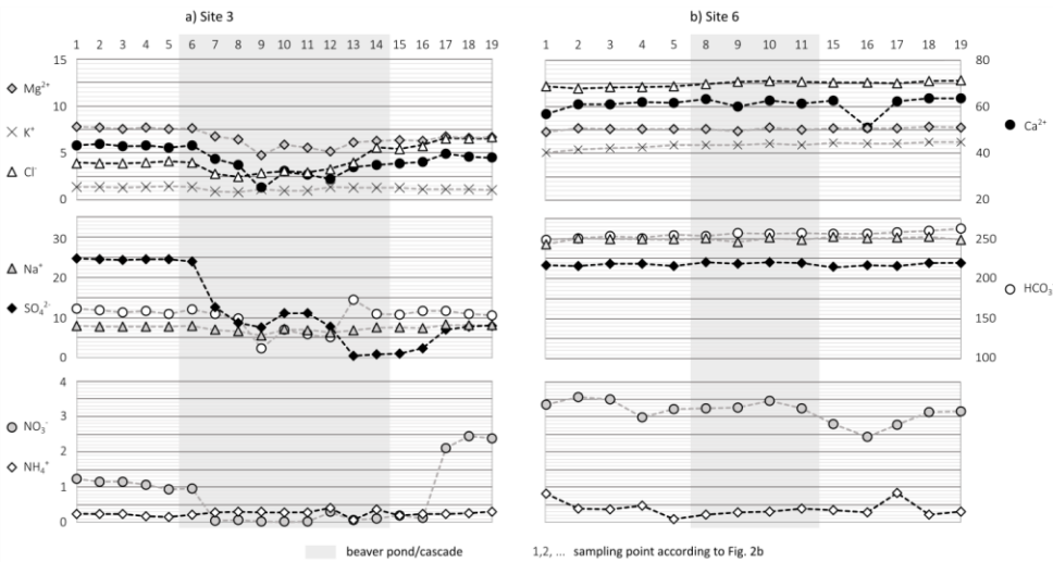
Figure B1: Concentrations of the chemical components of water [ \text{mg}\cdot\text{L}^{-1} ] in the longitudinal stream profiles at study sites 3 (a) and 6 (b) on 10 September 2023.
