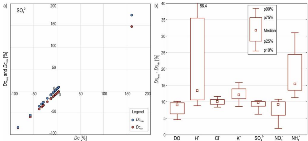
Figure A3. The lowest ( D_{c_{\min}} ) and highest ( D_{c_{\max}} ) possible D_c values, taking into account the percent relative errors of the chemical analysis, using the difference in \text{SO}_4^{2-} concentration in pond water and stream water above the ponds as an example (a). The differences between the lowest ( D_{c_{\min}} ) and highest ( D_{c_{\max}} ) possible D_c values for the selected chemical parameters are shown in (b).
