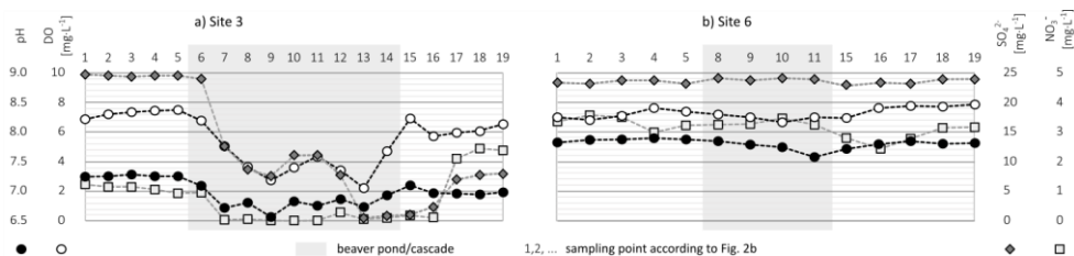
Figure 6: A longitudinal profile of the selected physico-chemical parameters at an overflowing and old study-sites (Site 3 –(a), and an in-channel and young site (Site 6 – (b) on 10 September 2023.
