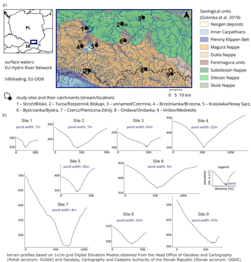
Figure 1: Study area – location (a) and valley cross-sections (b).
