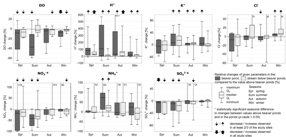
Figure 4: Percentage change (Dc) in the physico-chemical water parameters within and below beaver ponds in relation to stream water above beaver ponds. Only the parameters for which |Dc| > 15% are shown.
