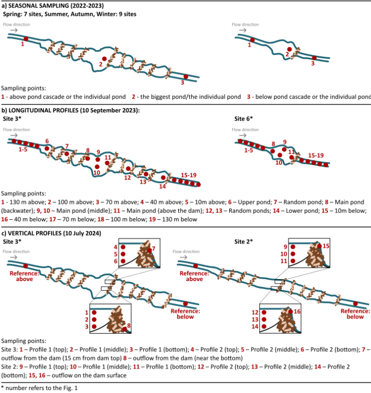
200 Figure 2: Study sampling schemes.
