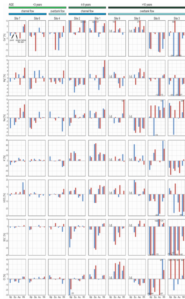
Figure A1: Percentage changes ( D_c ) in main ion concentrations in and below beaver ponds compared to their upstream values (Sp - spring, Su - summer, Au - autumn, Wi - winter, l.d. - lack of data).
