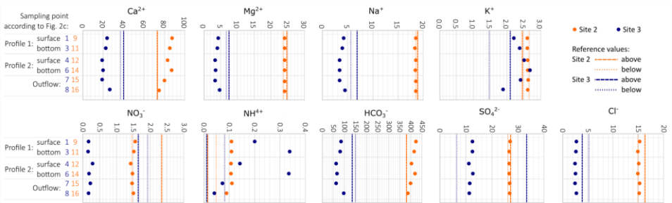
Figure B2: Concentration of the chemical components of water [ \text{mg}\cdot\text{L}^{-1} ] in the vertical profiles of study sites 2 and 3 on 10 July 2024.
