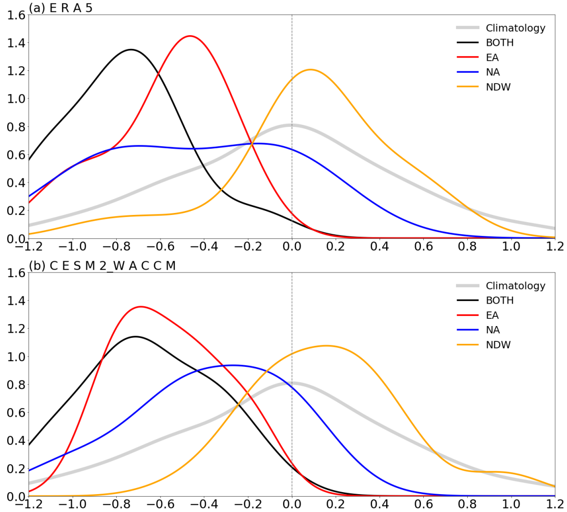
Figure 2. Probability density functions for the average NAO index during the 60 days after SSW onset date for BOTH (black curve), EA (red curve), NA (blue curve), and NDW (orange curve) events from two datasets: (a) ERA5 and (b) historical simulations by CESM2-WACCM. The climatological distribution (grey curve) is constructed from a combined sample of 2000 randomly selected 60-day winter periods drawn from both ERA5 and CESM2-WACCM. The Kernel Density Estimation is used for the 60-day mean index to smooth the PDF curve.
