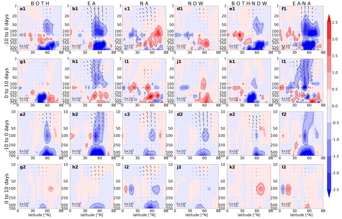
Figure 10. Same as in Figure 8, but for planetary wave 2 E-P flux.
