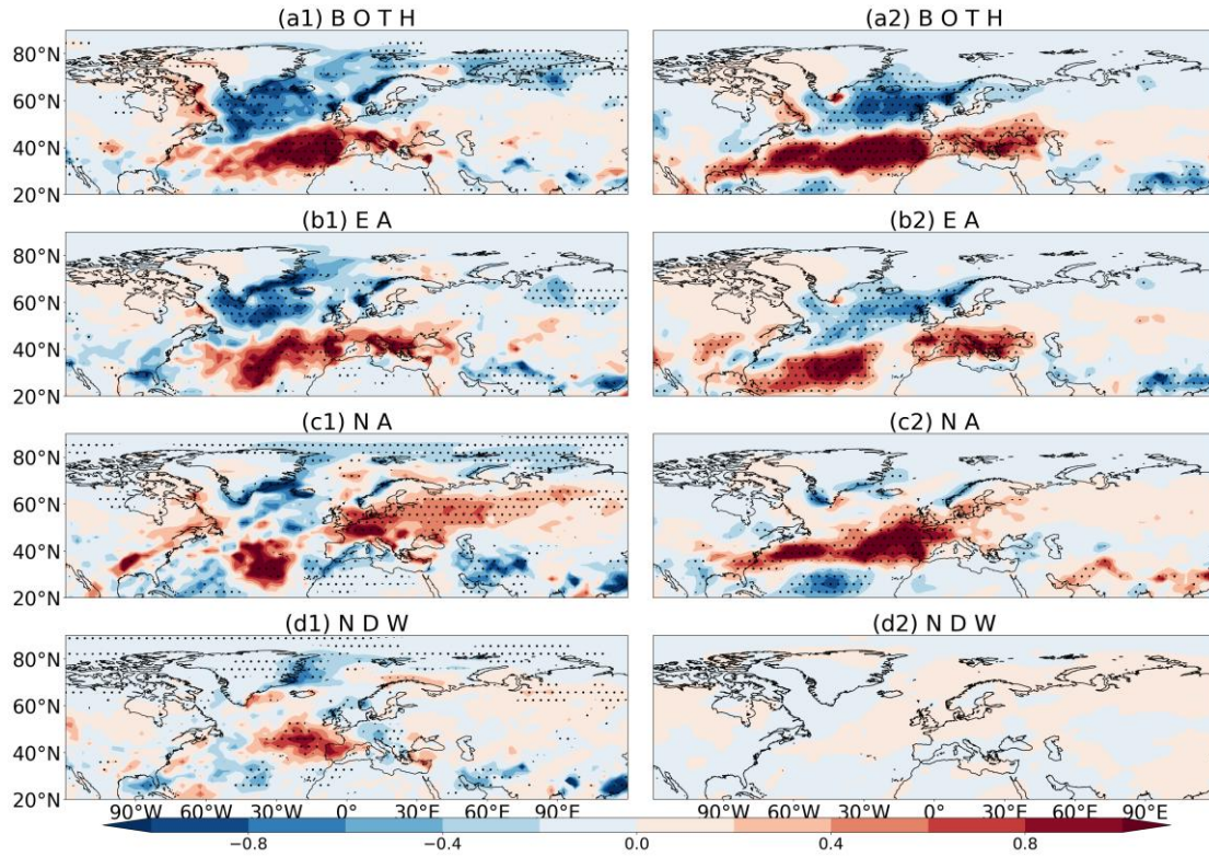
Figure 6. Composite precipitation anomalies (shadings; units: mm day -1 ) for (a) BOTH, (b) EA, (c) NA and (d) NDW events after the SSW onset from two datasets: (a1-d1) ERA5 and (a2-d2) historical simulations by CESM2-WACCM. The composite is based on the mean of day 0 to 40. The dots mark the composite anomalies at the 99% confidence level using the t -test.
