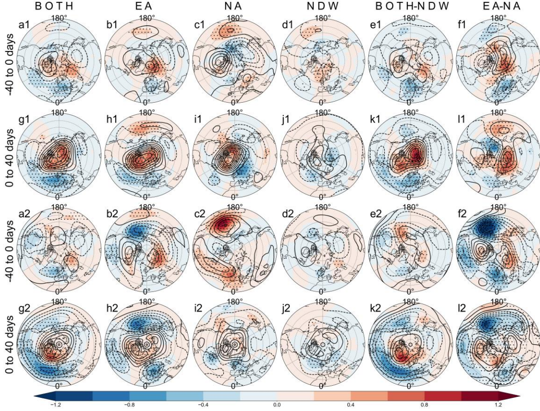
Figure 7. Composite 100-hPa geopotential height anomalies (contours; units: gpm) and sea level pressure anomalies (shadings; units: hPa) for (a, g) BOTH, (b, h) EA, (c, i) NA, (d, j) NDW, and the composite difference between (e, k) BOTH and NDW, (f, l) EA and NA before the SSW onset (top row) and afterward (bottom row) from two datasets: (a1-h1) ERA5 and (a2-h2) historical simulations by CESM2-WACCM. The composite is based on the mean of 40-day intervals. The dots mark the composite anomalies at the 95% confidence level using the t -test.
