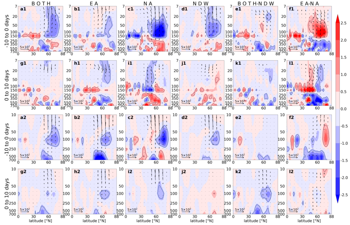
510 Figure 9. Same as in Figure 8, but for planetary wave 1 E-P flux.
