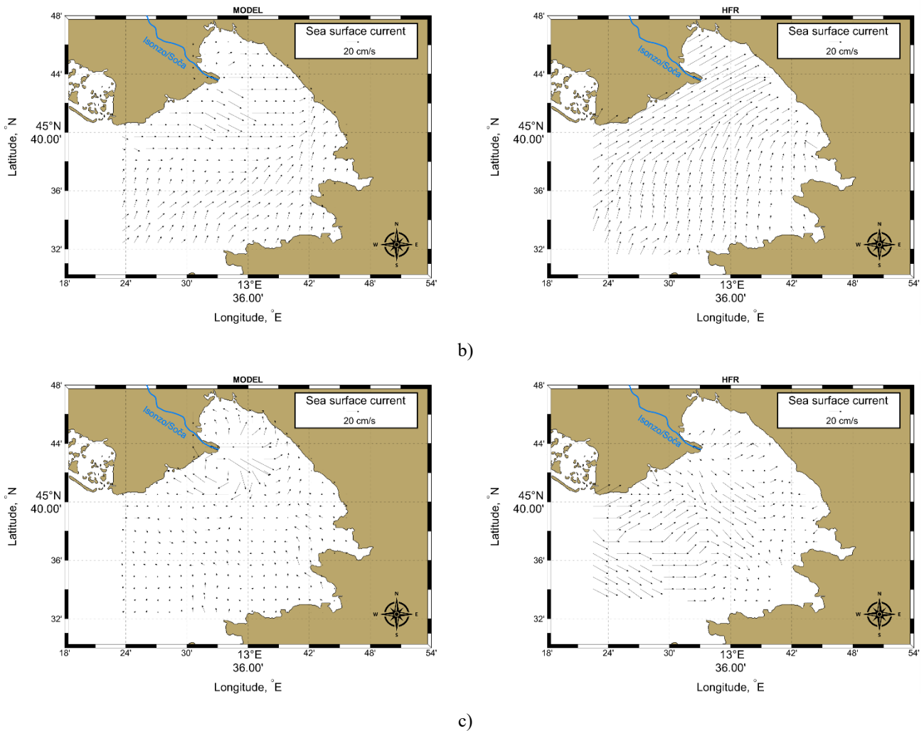
415 Figure 11: Comparison of MODEL and HFR data for the three different cases discussed in Sec. 3.3. (a) Bora wind without river outflow. (b) Southerly winds and weak outflow conditions. (c) Southerly winds and strong outflow conditions. The maps on the left and on the right show the MODEL and HFR data, respectively, with black arrows indicating the direction and speed of the currents.
