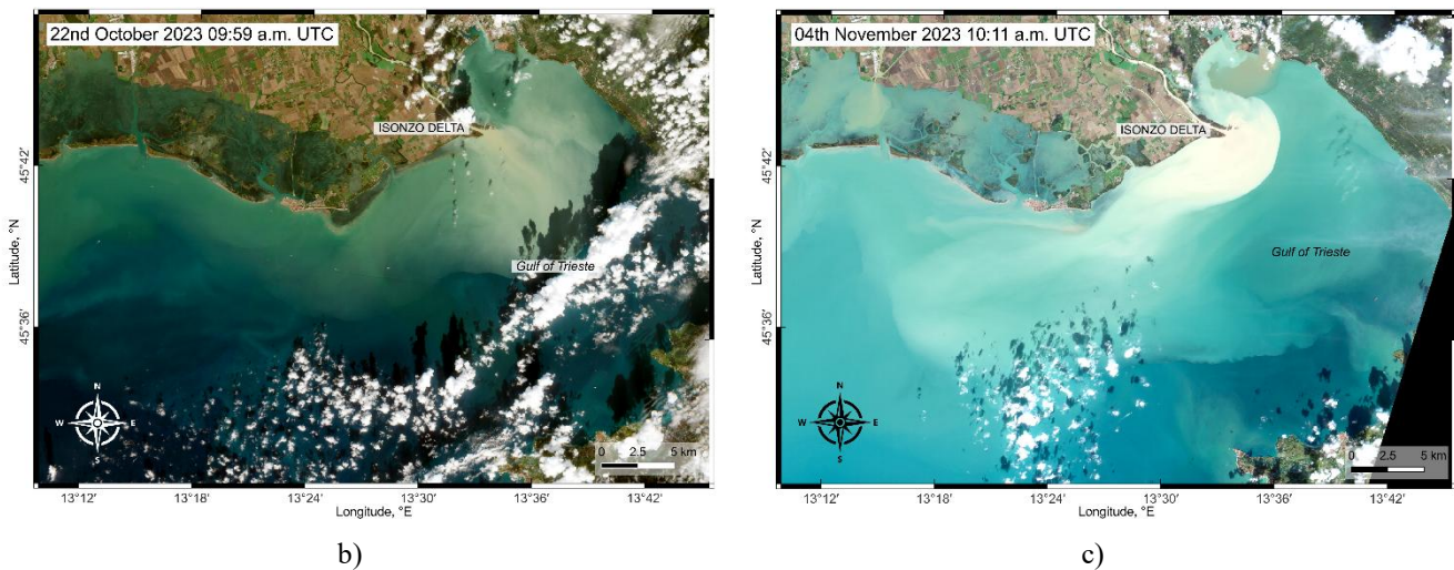
Figure 2: (a) Hydrometric data from Pieris hydrometric station in the year 2023, with the highest records highlighted in red. (b) Image Sentinel-2 22nd October 2023 09:59 a.m. UTC. (c) Image Sentinel-2 04th November 2023 10:11 a.m. UTC. Images Sentinel-2 were taken from Copernicus website: https://link.dataspace.copernicus.eu/l3n1 .
