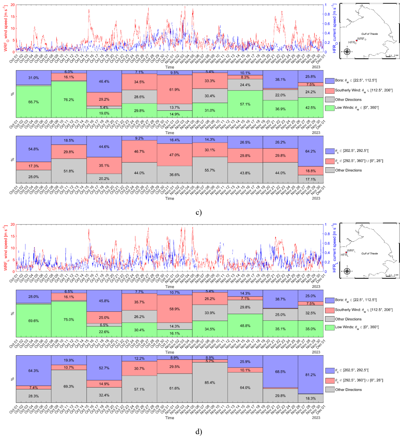
Figure 5: Comparison between the time series of surface current speed and wind speed for each of the four selected points in the GoT(a-d). Top panel: Time series of surface current velocity measured by HF radar (blue) and wind speed by WRF model (red). Middle panel: Weekly percentage distribution of wind kinds based on the WRF model (the direction refers to where the wind is
