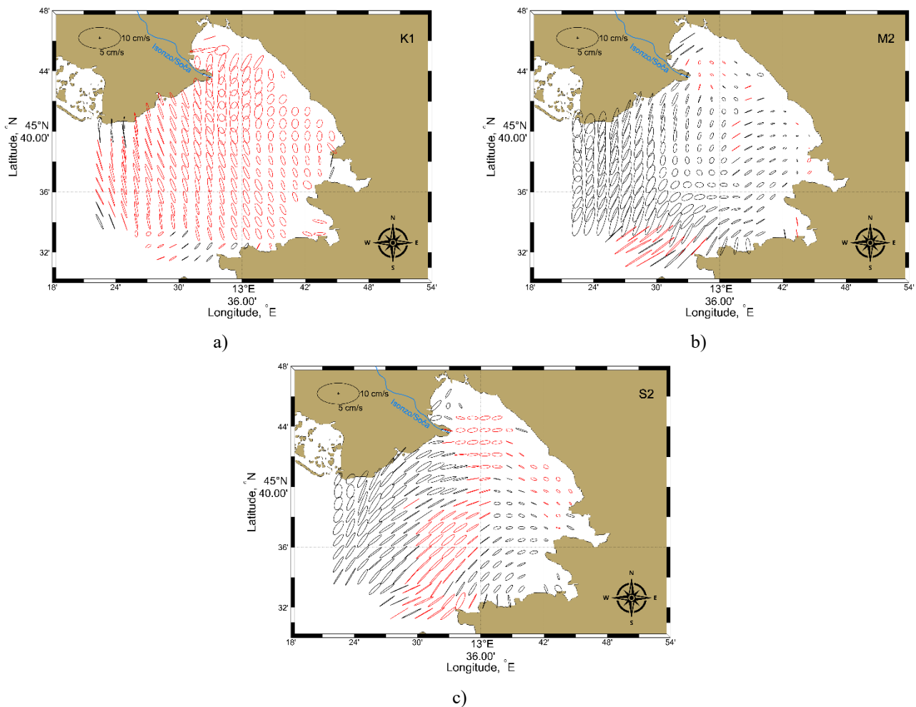
240 Figure 4: Tidal ellipses for the diurnal harmonic K_1 (a) and semidiurnal harmonics M_2 and S_2 (b and c). The black and red ellipses refer to a counterclockwise and clockwise rotation, respectively.
