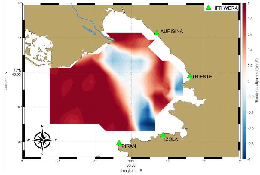
Figure S1: (a) Directional alignment ( \cos \theta ) map on 15th October 2023 19:00 UTC (Bora event). (b) Directional alignment ( \cos \theta ) map on 27th October 2023 05:00 UTC (Southerly wind event). (c) Directional alignment ( \cos \theta ) map on 28th October 2023 01:00 UTC (Southerly wind and strong river outflow event).
