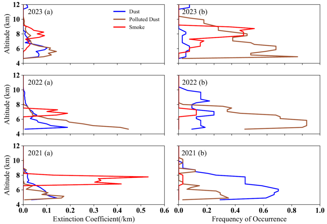
Figure 5. The vertical distribution of averaged aerosol extinction coefficient at 532 nm (a) and occurrence frequency profile of each aerosol type (b) during the peak of the fire season (March and April) from 2021 to 2023 over the southern of HTP (gray rectangle in Figure 1).
