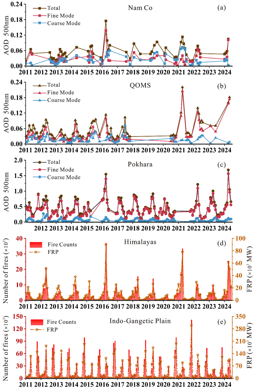
Figure 2. Temporal variations of monthly mean AERONET AOD at 500 nm, fine-mode AOD at 500 nm and coarse-mode at 500 nm at Nam Co (a), QOMS (b), and Pokhara (c); and time series of the monthly average number of fires and FRP from the MODIS Active Fire Product over the Himalayas (d) and Indo-Gangetic Plain (e).
