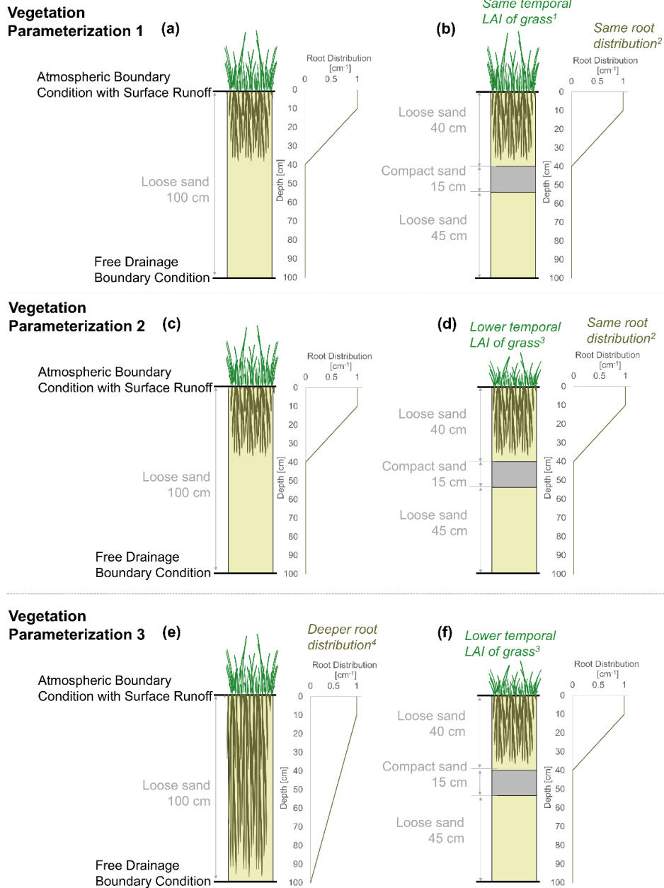
Figure 43. Schematic diagram of 1D soil water flow models for non-compacted and compacted cases under the three vegetation parameterizations.
