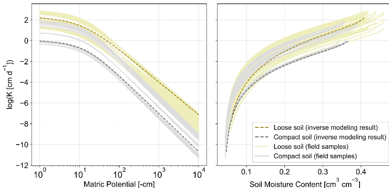
Figure A110. Conductivity curves ( \log K vs pF (left), \log K vs \theta (right)) for both loosened and compact sand layer based on optimization from inverse modeling and on field samples whose properties were inferred from ROSETTA and K_s measurements (falling head method)
