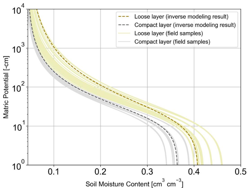
Figure A109. Water retention curves for loosened and compact sand layers based on optimization from inverse modeling and on field samples whose properties were inferred from ROSETTA.
