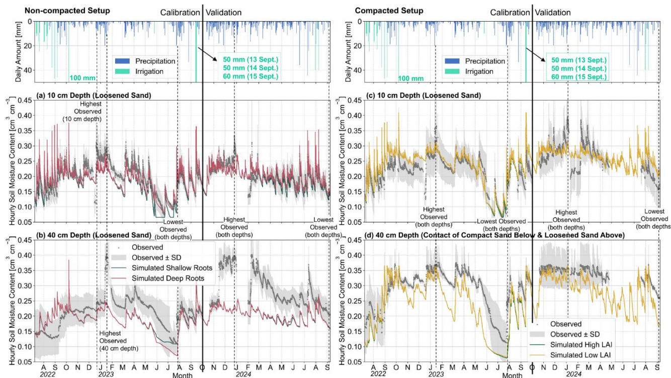
Figure 65. Observed soil moisture content ( \pm standard deviation (SD)) vs simulated soil moisture content time series at 10 and 40 cm depths under various vegetation parameterizations under calibration (08 July 2022–30 September 2023) and validation periods (01 October 2023–30 September 2024). Performance indicators are listed in Appendix B – Table B4B5.
