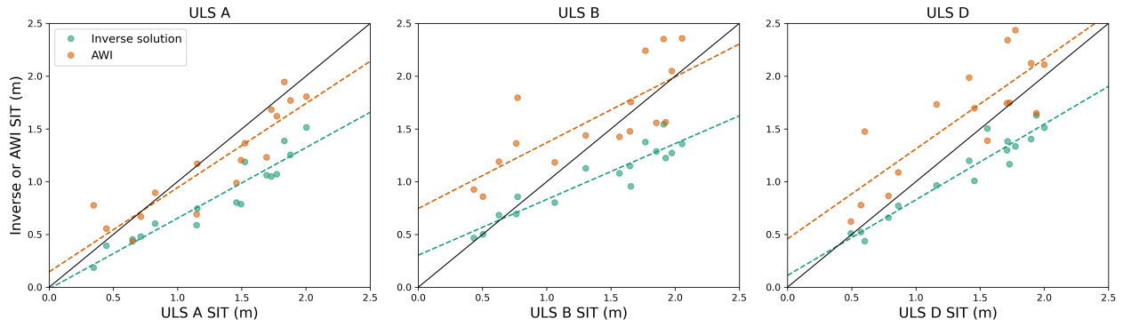
Figure 8. Validation of inverse SIT against BGEF moorings for the winter periods from 2018 to 2021. We also plot the results from AWI.
