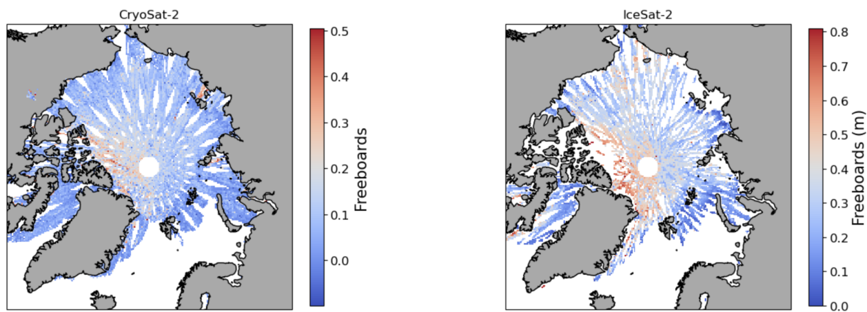
Figure S2. Example of input for April 2019 with the CS-IS satellite combination. The input is composed of daily along-track freeboard data binned on a 25 \text{ km}^2 EASE2 grid, for each satellite.
