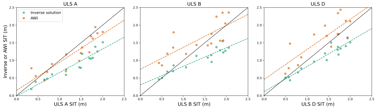
Figure 8. Validation of inverse SIT against BGEP moorings for the winter periods from 2018 to 2021. We also plot the results from AWI.
