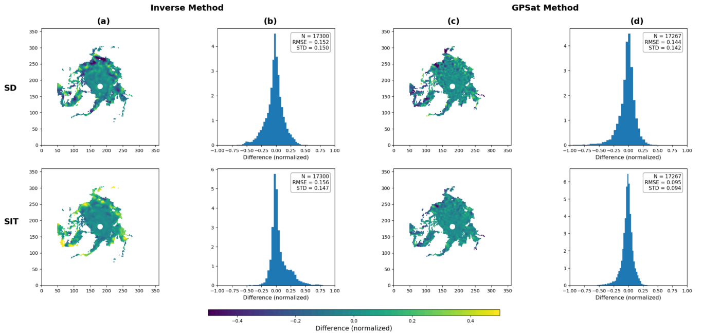
Figure 4. Quantitative analysis for the synthetic test. (a) Maps of the difference between Inverse SIT/SD and True SIT/SD, normalized by the maximum value of the SIT/SD ( \frac{\text{Inverse SIT/SD} - \text{True SIT/SD}}{\text{True SIT/SD}} ) (b) Histograms of the differences for the Inverse solution. The root mean squared error (RMSE) and the standard deviation (STD) are also computed (c) Maps of the difference between GPSat SIT/SD and True SIT/SD, normalized by the maximum value of the SIT/SD ( \frac{\text{GPSat SIT/SD} - \text{True SIT/SD}}{\text{True SIT/SD}} ) (d) Histograms of the differences for the GPSat solution.
