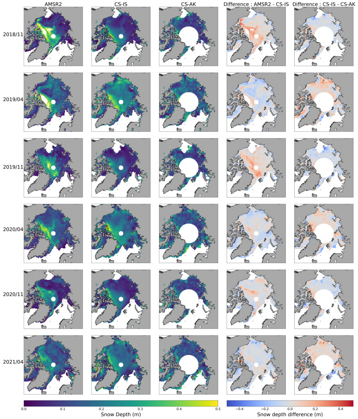
Figure 9. Comparison of our inversion for SD against AMSR2 product with \alpha_{cs} = 1 and \alpha_{ak} = 0 . We also compute the difference between AMSR2 and the CS-IS combination and the difference between the two combinations of satellites.
