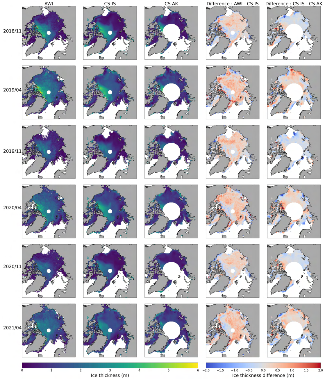
Figure 5. Results of the inversion for the SIT using CS-IS-2p and CS-AK-2p, with \alpha_{cs} = 1 , \alpha_{is} = 0 and \alpha_{ts} = \alpha_{ak} = 0 , \alpha_{ak} = 0 . The first column shows the AWI SIT product, for visual comparison. The second and third columns show the CS-IS and CS-AK results, respectively. The fourth column shows the difference between the AWI product and the CS-IS results. The fifth column shows the difference in inversion results between the two satellite combinations (CS-IS and CS-AK).
