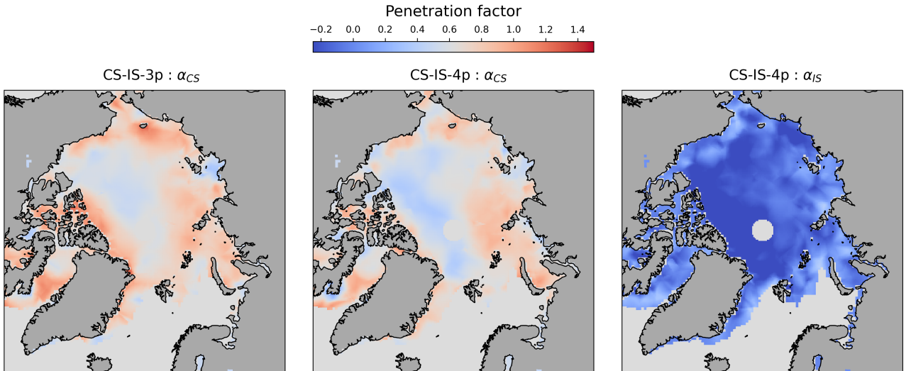
Figure 11. Result of the inversion with (a) CS-IS-3p (inversion for SD, SIT and \alpha_{cs} ) and (b) CS-IS-4p (inversion for SD, SIT, \alpha_{cs} and \alpha_{is} ) for April 2019 for the penetration-bias factors. The priors on the different physical parameters can be found in Section 3.
