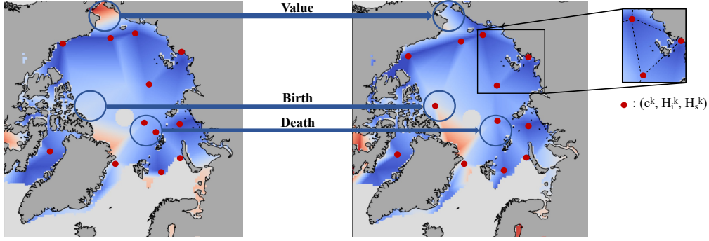
Figure 1. Schematic of 3 of the different perturbations than that can be applied at each iteration of the algorithm. We display a zoom on a Delaunay triangle with the different model parameters associated to a node (red point). The red dots are the triangle vertices to which the parameter are associated and the dashed lines are the sides of the triangles. The meaning of each change are Value : The value of a randomly chosen node of index k in the map is perturbed as well as its associated values H_i^k and H_s^k ; Birth : A new node is created with the associated values randomly drawn from the prior distribution defined previously. That is, a new node is created with position c_{H_i}^{n_H+1} and values H_i^{n_H+1} and H_s^{n_H+1} ; Death : A randomly chosen cell and the associated value of the physical parameter are deleted.
