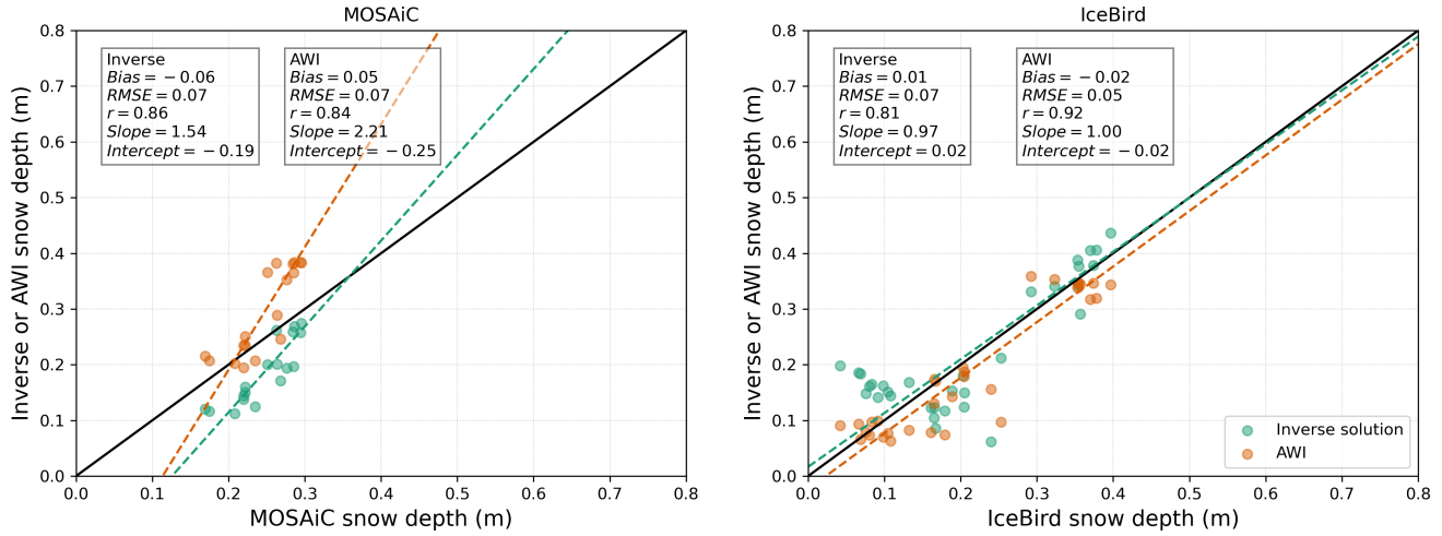
Figure 10. Evaluation of the results from the inversion using CS-IS-2p for SD. The validation is performed against MOSAïC (for Winter 2019-2020) and IceBird (for 2019/04).
