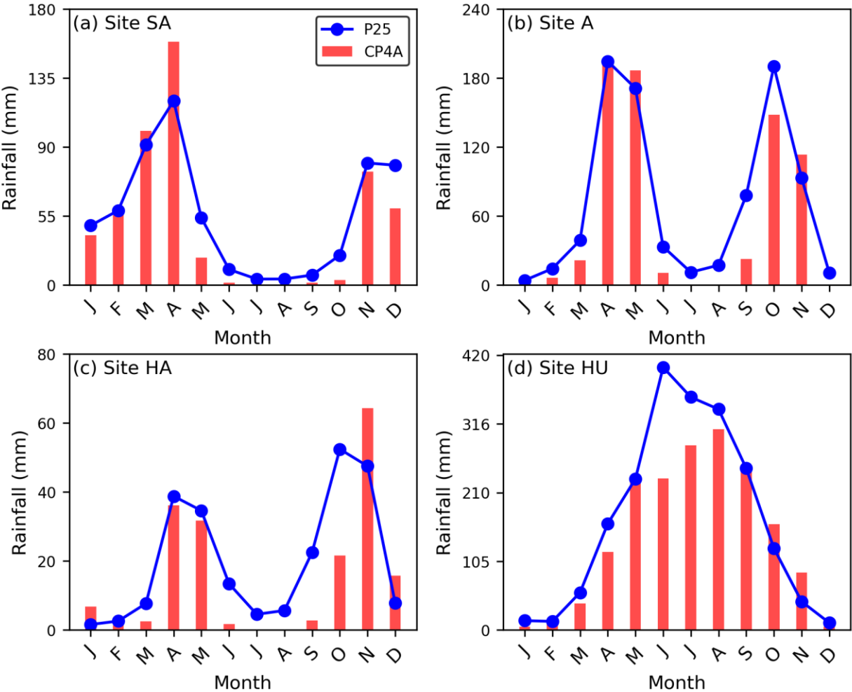
Figure B1 – Mean monthly rainfall at each of our four hydrological study sites using the CP4A/P25 ‘historical’ runs. These ‘historical’ CP4A/P25 simulations were designed to be statistically consistent with the observed climate between March 1997 and February 2007. The simulated seasonal cycles show good agreement with the observed seasonality (Cocking et al., 2024)
