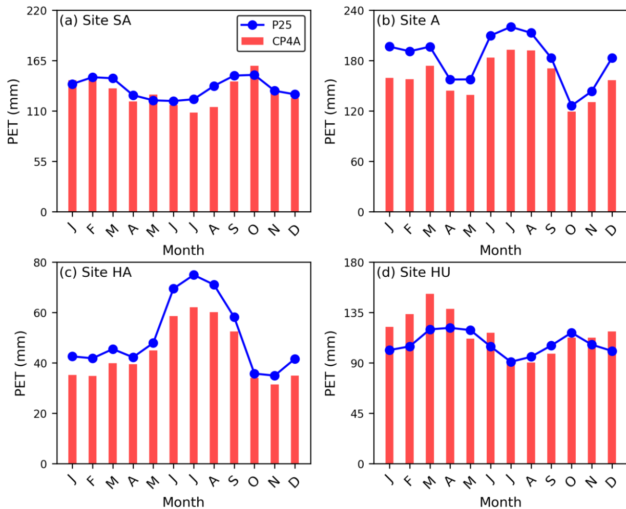
Figure B2 – Mean monthly PET at each of our four hydrological study sites, using the CP4A/P25 ‘historical’ runs. These ‘historical’ CP4A/P25 simulations were designed to be statistically consistent with the observed climate between March 1997 and February 2007. The simulated seasonal cycles of PET show good agreement with hPET (not shown).
