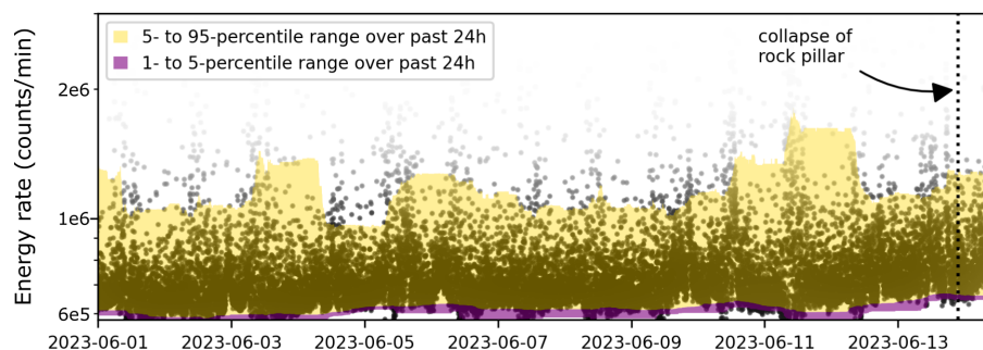
Figure 8. Evolution of seismic energy (logarithmic scale) prior to the collapse at the closest seismometer station (MH44; Fig. 1) - saturation of dots represents the kernel-density estimation based on Gaussian kernels: An increasing baseline of the energy level appears towards failure.
