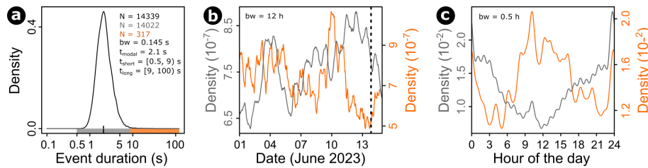
Figure 10. Temporal emergence patterns of seismically detected events, depicted as kernel density estimate plots. (a) Duration of STA-LTA-picked events with basic statistic characteristics, kernel bandwidth = bw, number of cases by color. The gray bar indicates “short events”, orange bar shows “long events”. (b) Event density curves for the studied time period. Colors as in (a), the gray dashed line indicates the time of collapse for the main rock pillar. (c) Occurrence of events at the diurnal scale. Colors as in (a).
