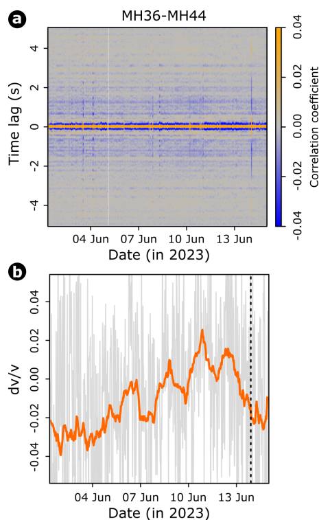
Figure 9. Seismic noise cross-correlation analysis. a) Correlogram of average cross-correlations across all seismic components for the station pair MH36–MH44. b) Raw 30 min resolved (gray lines) and 24-hour running average time series (orange line) of dv/v values. The black dashed line marks the occurrence of the rock pillar collapse.
