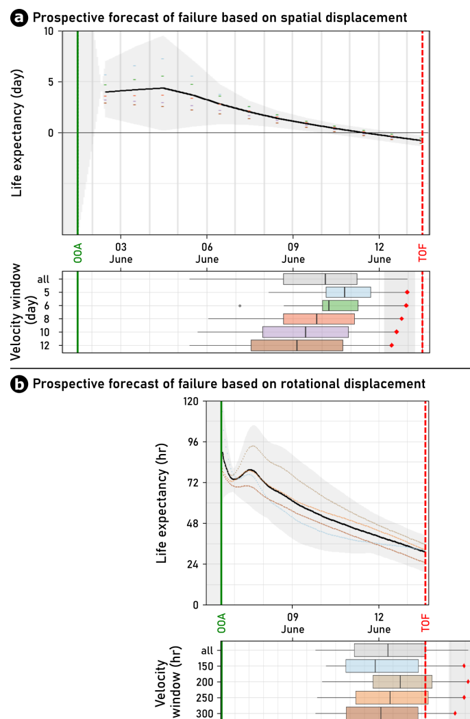
Figure 7. Prospective forecast of failure based on (a) spatial and (b) rotational displacement. The onset of acceleration (OOA; green solid line) is detected 12 and 7 days before failure. Colored points mark the life expectancy at the time when the forecast was calculated for each smoothing window length. The black line marks the mean forecast and the gray area the forecast uncertainty. The collapse of the rock pillar (time of failure TOF; red dashed line) is in between forecasts (a) and (b). Boxplots give information on all forecasts since the OOA per velocity window.
