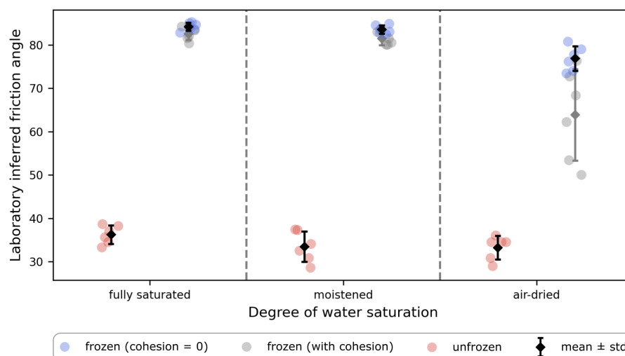
Figure 12. Laboratory-inferred friction angles grouped by degrees of saturation and temperature: While red refers to an unfrozen state ( +10^{\circ}\text{C} ) with assumed cohesion of 0\text{ kPa} , blue and gray refer to a frozen state ( -5^{\circ}\text{C} ) without cohesion ( 0\text{ kPa} ) and the cohesion value according to the Mohr-Coulomb failure criterion in Mamot et al. (2018), respectively. The influence of cohesion on the inferred friction angle is shown in the supplementary Figure S1.
