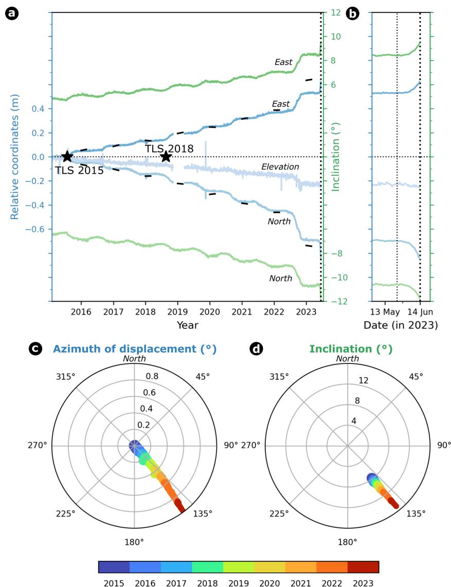
Figure 6. Spatial (azimuth; blue) and rotational (inclination; green) displacement time series for the (a) period 2015–2023 and (b) the last month before collapse, indicating a sudden acceleration starting ~10 days prior to failure. The black lines during the winter months show that the spatial displacements (North and East) can be fully explained by toppling with a tilt radius of 10m until a change in the kinematic process occurred in 2022. The polar visualization of the (c) spatial and (d) rotational displacements show a matching direction of movement or tilting.
