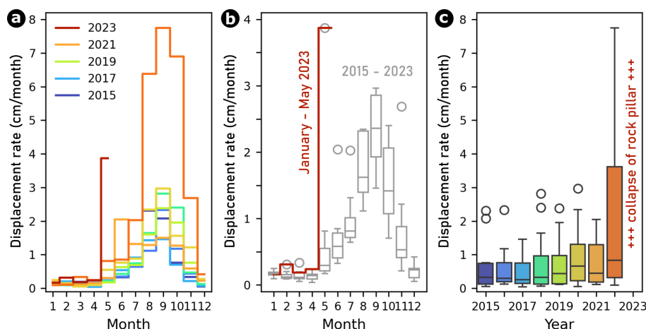
Figure 5. Monthly and annual spatial displacement rates of the rock pillar measured with a permanent GNSS station.
