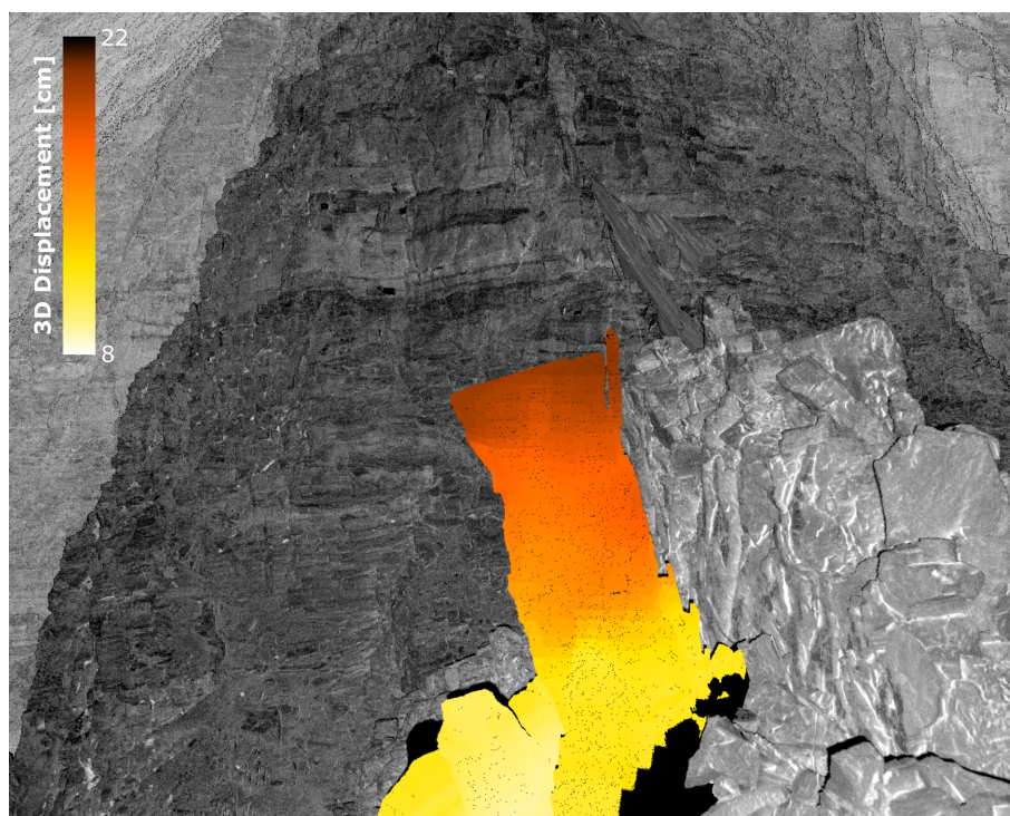
Figure 4. Isolated point cloud analysis showing the 3D displacement between the terrestrial laser scans on 27 July 2015 and 20 August 2018 (change in dip angle is shown in supplementary Fig. S5). During this period, the GNSS station (deployed at the upper right corner of the rock pillar) moved by 21 cm relative to the permanently installed TLS mounting plate.
