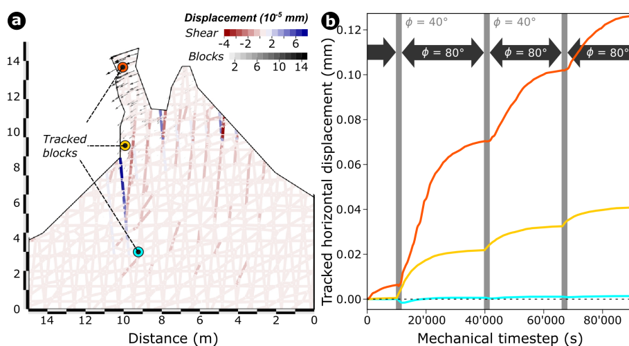
Figure 13. (a) Numerically calculated spatial distribution and magnitude of displacements of blocks and individual joints for the freestanding Matterhorn rock pillar after calculation of 90000 mechanical time steps. (b) Modeled effect of the seasonal but short-term drop in friction angles along fractures (between blocks) induced by temporary thawing due to percolating snowmelt water (gray bars).
