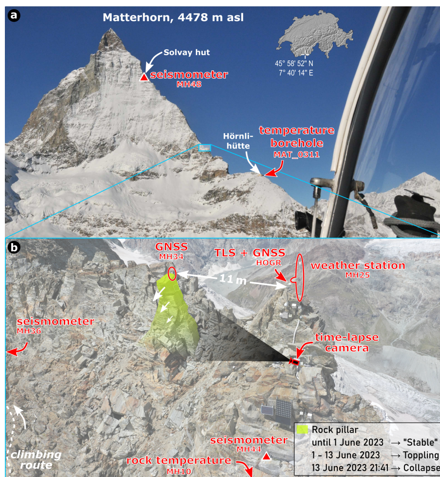
Figure 1. (a) The Matterhorn Hörnligrat Cryosphere Observatory is located along the northeastern ridge of the Matterhorn, with the main study site located between the Hörnli hut and Solvay hut. (b) A zoom to 3500 m asl highlights the freestanding rock pillar with a volume of approx. 20 \text{ m}^3 in yellow and labels the surrounding sensors in red. The white reference line between GNSS MH34 (rock pillar) and GNSS HOGR (mounting plate for terrestrial laser scanner) represents a distance of 11 meters. Rock samples for the laboratory experiments were collected behind the rock pillar on the North side. The white dashed line marks the climbing route in the flank just below the rock pillar, via which approximately 3000 climbers attempt to reach the summit each year, mostly between July and mid-September.
