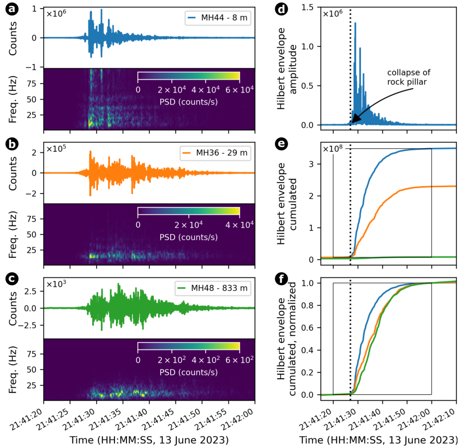
Figure 11. Seismic response to the impact of the collapsing rock pillar (black dotted line): (a)-(c) waveform and spectrogram as well as (d)-(f) energy estimate based on Hilbert envelope for the North component of the three seismometer stations MH44 (blue), MH36 (orange) and MH48 (green).
