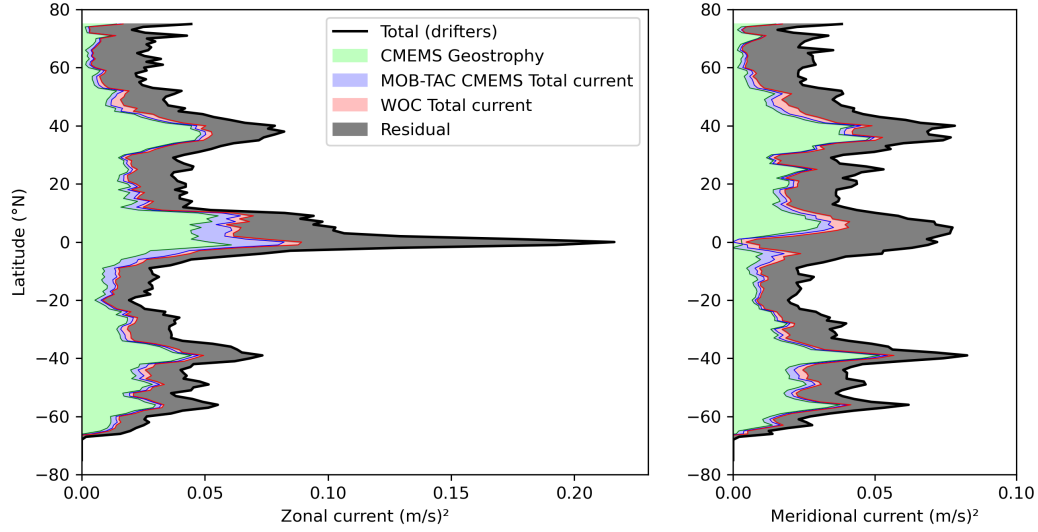
Figure 6. Variance of the Black lines : variance of the observed surface current (zonal component on the left, meridional on the right) as a function of latitude averaged globally for the drifter database between 2017 and 2020. The black line is for the total current derived from the drifters . The green, blue and red lines are the variance reduction after applying the Geostrophy from CMEMS represent the explained variance of the CMEMS geostrophy , the CMEMS MOB-TAC total current and the WOC total current. The explained variance is defined as the total variance (black) minus the variance reduction after applying the different current estimates. The filled colors indicate the relative amount of additional explained variance between successive products.
