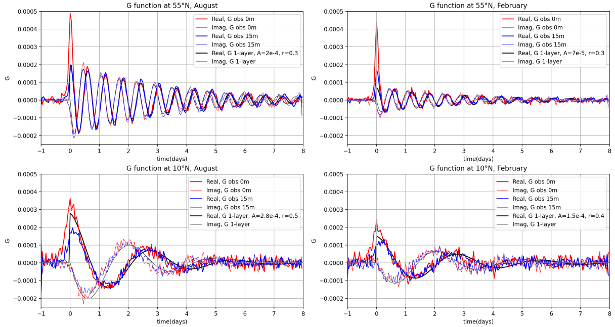
Figure 8. Upper panel-panels : G function from the first set of parameters in summer at latitude 50^{\circ} at latitude 55^{\circ} N and longitude -40^{\circ} E, represented as a function of the t' interval, for the real (plain line thick lines) and imaginary parts (dotted line). Lower-left panel : G function from the final parameters with the Fourier time-decomposition truncated at twice the Coriolis frequency. Lower-right panel : same function represented in the Real/Imaginary plane (thin lines). Upper-left panel in August and upper-right panel in February. Lower panels : same as upper panels, but at 10^{\circ} N.
