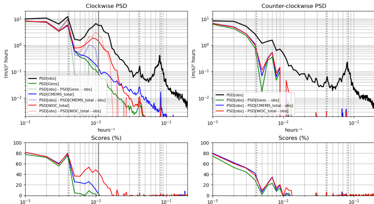
Figure 5. Same as Figure 4, averaged between 5°N and 10°N with vertical plain-solid line indicating the inertial frequency at 7.5°N
