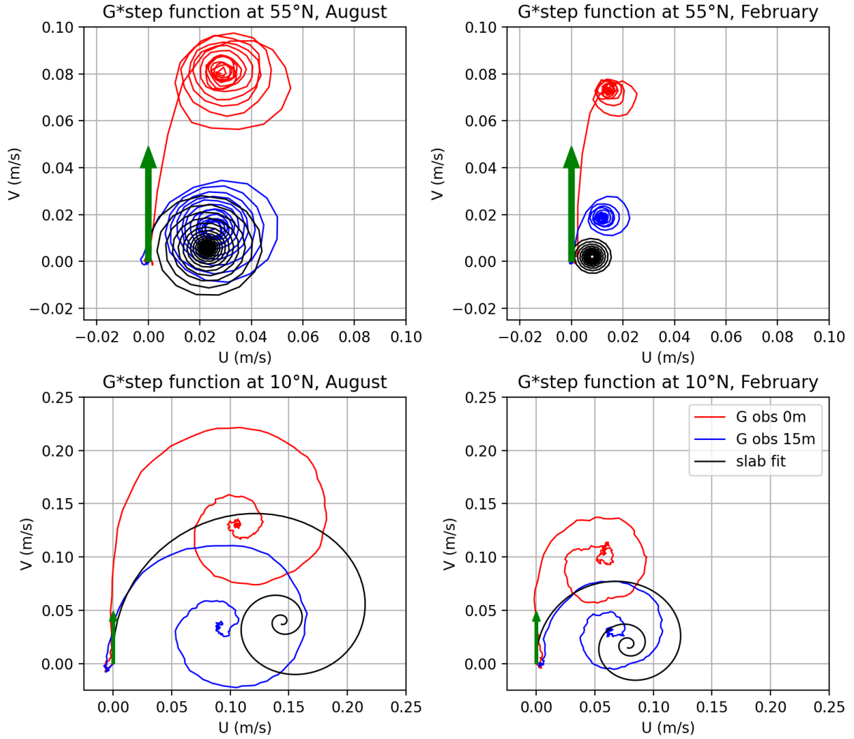
Figure 9. Integration of the response function with a unitary-step function of the wind represented by the green arrows. The result, called step-response functions, are represented in the (Real, Imaginary U, V ) plane by the red, blue and black lines for the undrogued drifters, drogued drifters and slab respectively. The four panels represent the different latitudes and seasons as in Figure 8
