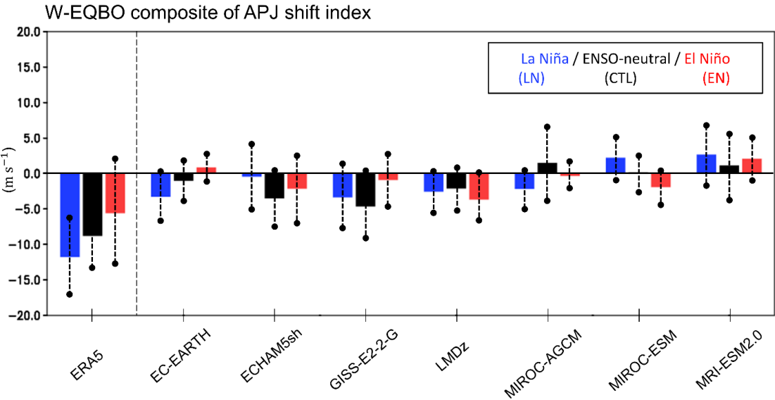
500 Figure 7: QBO-W minus QBO-E composite difference of the Asia-Pacific Jet (APJ) shift index. The APJ-shift index is defined as the difference of the 250-hPa zonal wind anomalies averaged over the Pacific sector (150° E–150° W) between the northern flank (40°–50° N) and the southern flank (20° N–30° N) of the climatological APJ core. The negative value indicates that the APJ moves toward the equator during the QBO-W phase. The composite differences are shown for the La Niña or LN experiment (blue), ENSO-neutral or CTL (black), and El Niño or EN experiment (red). The values are considered significant if the 5-95 % range of the bootstrap distribution (vertical dashed lines) does not encompass zero. 505
