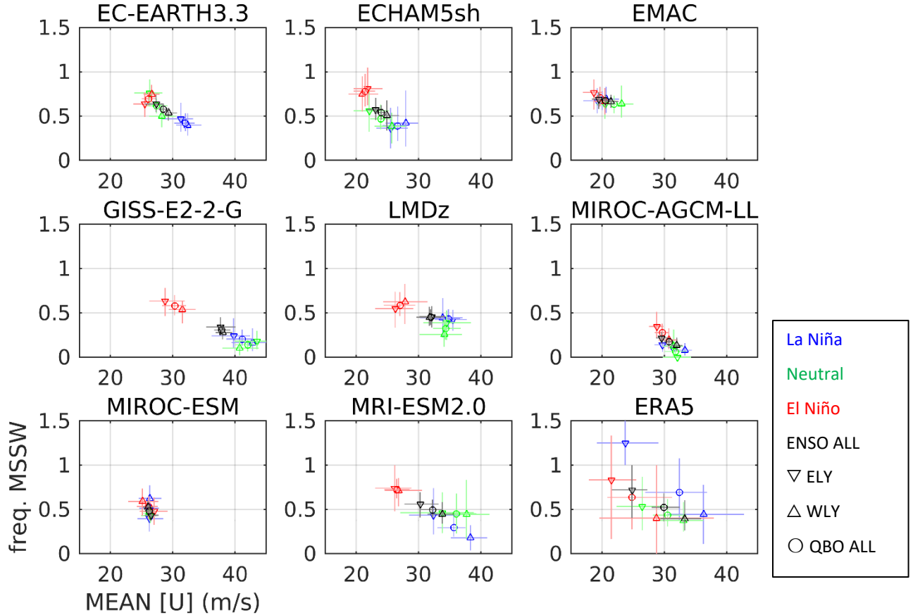
425 Figure 5: Scatter plots between mean vortex strength ( 60^\circ N, 10 hPa) and major SSW frequency during DJF for different QBO and ENSO conditions. Major SSWs are identified as a reversal of daily zonal-mean zonal wind at 60^\circ N and 10 hPa. QBO phases are classified using DJF-mean zonal-mean zonal wind anomalies at 50 hPa averaged over 5^\circ S– 5^\circ N using \geq 0 \text{ m s}^{-1} for QBO-W (WLY in panel) and < 0 \text{ m s}^{-1} for QBO-E (ELY). The anomalies are calculated for each ensemble member of each experiment for the simulation data; those ones are calculated using all years (1959–2021 seasons) for the ERA5 data. For ERA5, El Niño and La Niña winters are when all three DJF months have the El Niño and La Niña flag, respectively. Number of (QBO-W, QBO-E) categories for ERA5 are (24, 15) in ENSO-Neutral, (5, 6) in El Niño, and (9, 4) in La Niña winters. For each condition, each model, the data are randomly resampled 100 times with replacement, and then 95% ranges are obtained and plotted.
