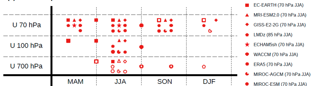
Figure 13: (a) Occurrence of a statistically significant zonal wind signal by models, season and altitude over the equatorial (10° S–10° N) 60° E–120° E band for the (a) CTL, (b) LN, and (c) EN experiments. The QBO-W minus QBO-E zonal wind signals are evaluated at three vertical levels and across four standard seasons. Symbols are placed between standard seasons when the strongest signal occurs in an intermediate period. Filled symbols represent westerly anomalies, while open symbols indicate easterly anomalies. The QBO definition for each model and experiment is provided in the legend.
