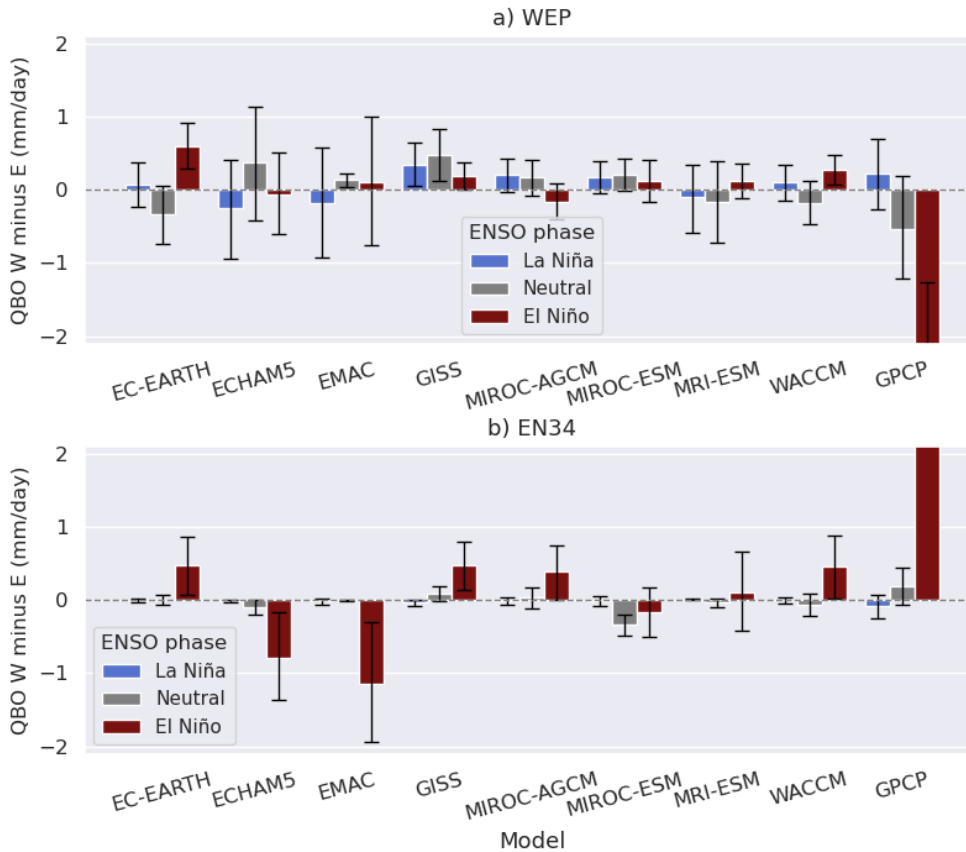
Figure 9: (a-b) Box plots of QBO-W minus QBO-E differences in DJF precipitation ( \text{mm day}^{-1} ) in (a) the western equatorial Pacific (WEP) and (b) EN3.4 region ( 5^{\circ}\text{ S} – 5^{\circ}\text{ N} , 170^{\circ} – 120^{\circ}\text{ W} ). Error bars represent the 95 % confidence interval. Note that the y-axis is fixed to make the plot clearer, but an alternative version where the y axis limits are set based on the GPCP bar is provided in supplementary Fig. S8.
