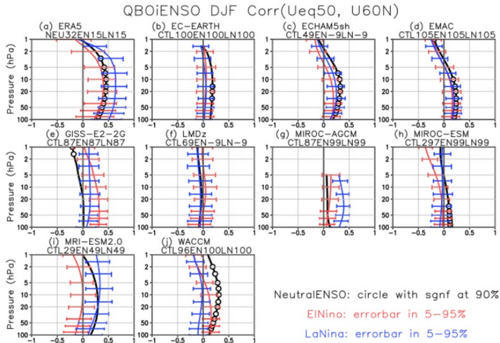
280 Figure 1: Vertical profiles of correlation coefficient between the QBO zonal wind at 50 hPa averaged over 5° S–5° N and the polar-vortex zonal wind at 55°–65° N in December-January-February (DJF) for QBOi models and ERA5. Circles represent statistical significance at the 90 % level. Red and blue bars represent 5–95 % confidence ranges using a bootstrap method repeating 1000 times in EN and LN experiments for the models as well as El Niño and La Niña winters for ERA5. Number of winters available for each model run for each experiment (ENSO phase) are displayed at the upper panel. For example, 'NEU32EN15LN15' in the ERA5 panel means there are 32 ENSO-neutral, 15 El Niño, and 15 La Niña winters, respectively.
