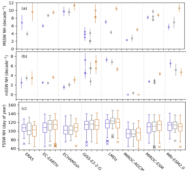
Figure 4: SSW statistics in NH in CTL, EN, and LN experiments for QBOi models including ENSO neutral, El Niño, and La Niña years for ERA5, based on their daily data. The order of triplets from left to right are La Nina (LN, purple), ENSO neutral winter experiment (CTL, grey), and El Nino (EN, brown). Frequency (number of events per decade) of (a) major SSWs (reversal of zonal-mean zonal wind at 10 hPa and 60° N; U60) and of (b) minor SSWs (reversal of 90°–60° N temperature gradient at 10 hPa without U60 reversal), occurring across full seasons. It is noted that multiple marker signs in the same experiment for a model indicate ensemble members (depending on data availability). Uncertainties are estimated at the 5–95% level based on bootstrapping of 10 years of winter months. (c) Boxplots of final SSW date (day of year), considering full seasons, i.e., from westerlies onset to their turn to easterly for ERA5 and QBOi models based on their daily data.
