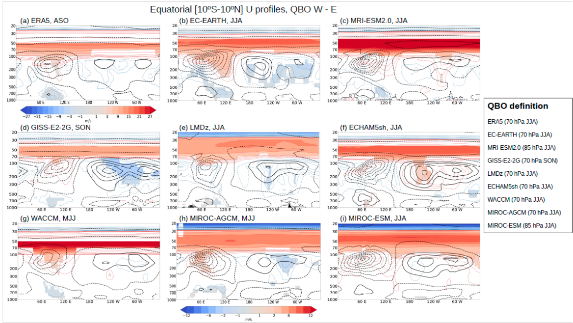
705 Figure 11: Climatology (black contours) and QBO Westerly (W) minus Easterly (E) differences (shading and colored contours) in equatorial zonal wind profiles, averaged over 10° S–10° N, from the LN experiment for the QBOi models. Black contours are drawn at 4 m s -1 intervals. Colored contours use the same intervals as the shading, with red contours indicating positive and blue indicating negative differences. The target season for each panel is indicated in the title, with the QBO definition provided in the legend. In ERA5, 15 La Niña events are identified using the NINO3 index during DJF, and they are classified into 10 QBO-W and 5 QBO-E categories by analyzing the zonal-mean zonal wind at 50 hPa in summer and autumn. Only statistically significant zonal wind differences at the 95 % confidence level are shaded. For models with a QBO definition other than 70 hPa during JJA, the Bonferroni correction is applied (see Section 2). Note that the color bar for ERA5 differs because of the larger QBO amplitude.
