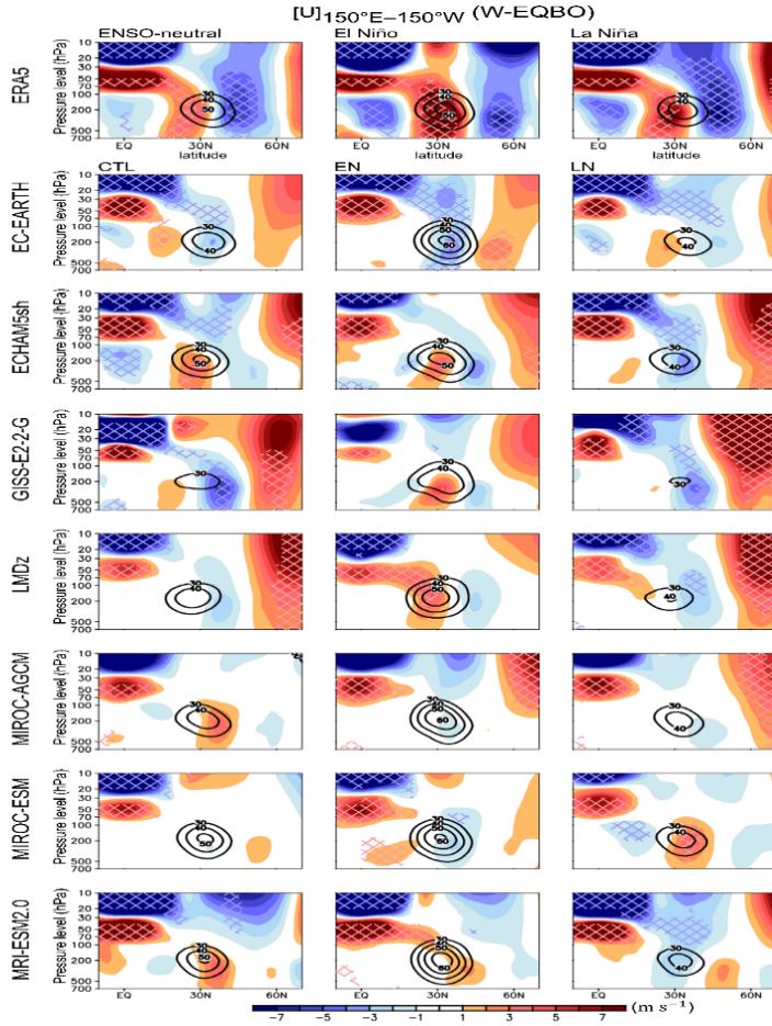
Figure 6: QBO-W minus QBO-E composite differences of zonal wind averaged over the Pacific sector ( 150^{\circ} E– 150^{\circ} W) for the ENSO-neutral (top-left), El Niño (top-middle), and La Niña (top-right) winters and those for the CTL, EN, and LN experiments (left to right columns). Values that are statistically significant at the 95% confidence level are cross-hatched. Contour denotes the climatological jet with zonal wind speed equal to or greater than 30 \text{ m s}^{-1} . QBO-W and QBO-E phases are defined as deseasonalized February–March zonal-mean zonal wind over 5^{\circ}\text{S} – 5^{\circ}\text{N} at 70 hPa being > 0.5 \sigma and < -0.5 \sigma , respectively. Numbers of (QBO-W, QBO-E) categories for ERA5 are (10, 9) in ENSO-Neutral, (6, 3) in El Niño, and (12, 7) in La Niña winters.
