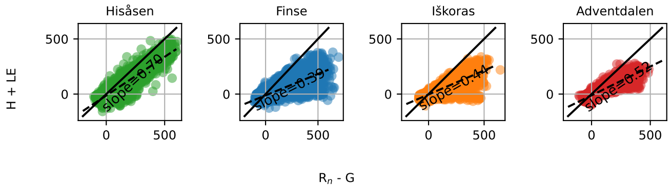
Figure F2. Energy balance closure (whole year) for Hisåsen (green), Finse (blue), Iškora (orange) and Adventdalen (red). The energy balance is estimated from the slope of the linear regression of the sum of latent and sensible heat on the y-axis against available energy (difference between net radiation and soil heat flux) on the x-axis.
