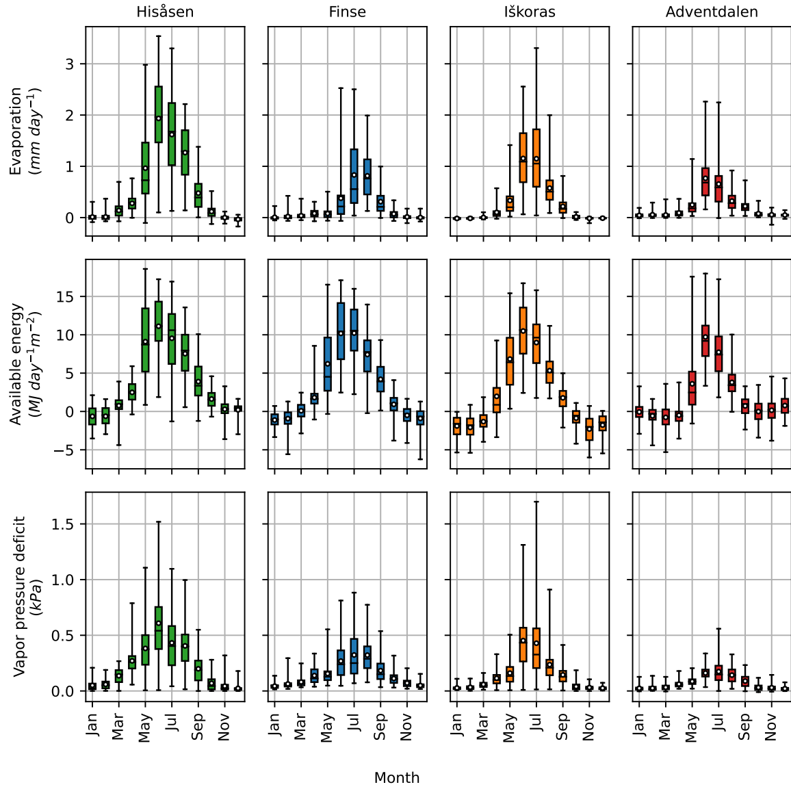
Figure 5. Daily evaporation in mm d -1 (upper row), available energy in MJ m -2 d -1 (middle row) and vapour pressure deficit in kPa (lower row) for each month at the four sites. For each month, the box plot represents median, 25- and 75 quantiles, and whiskers represent minimum and maximum values. The mean is represented by a white dot. Daily values are cumulative values of half-hourly values for evaporation and available energy, and daily mean for vapour pressure deficit.
