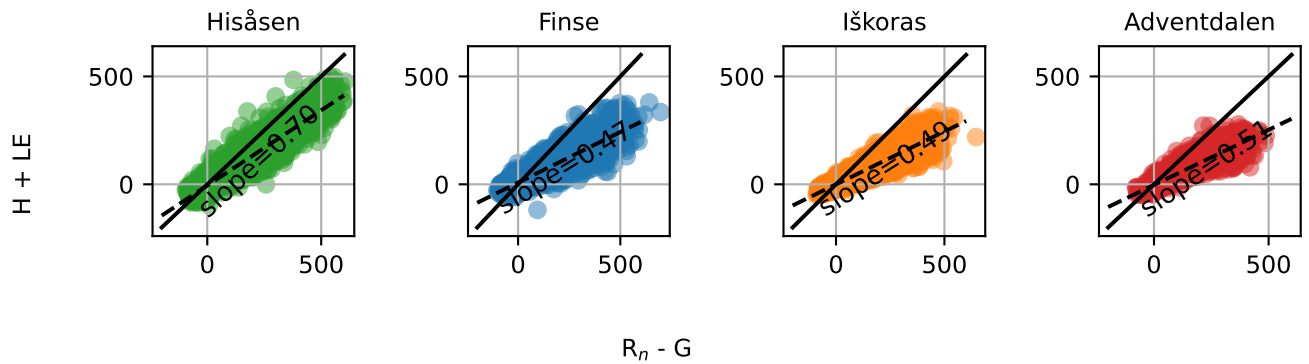
Figure F1. Energy balance closure in the snow-free season for Hisåsen (green), Finse (blue), Iškora (orange) and Adventdalen (red). The energy balance is estimated from the slope of the linear regression of the sum of latent and sensible heat on the y-axis against available energy (difference between net radiation and soil heat flux) on the x-axis.
