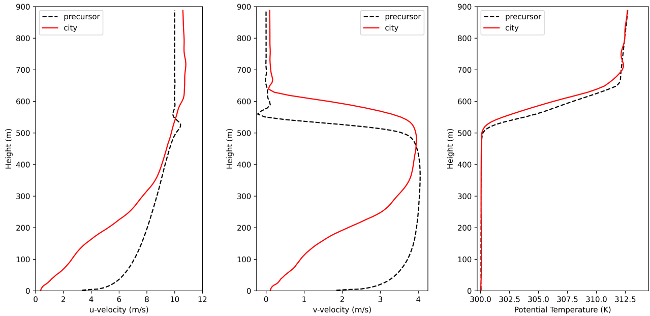
Figure 23. Plot of the time-average over t \in [8, 10]\text{hr} of u -velocity (left), v -velocity (middle), and potential temperature (right) averaged over the city domain in the horizontal for precursor simulation and the city simulation forced by the precursor.
