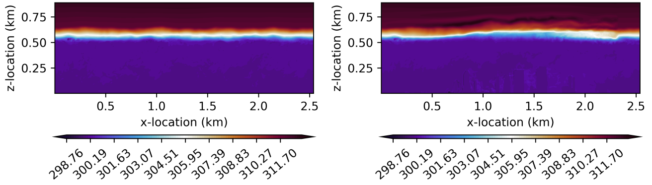
Figure 22. Plot of instantaneous potential temperature at t = 10\text{hr} for the concurrent turbulent precursor simulation (left) and the forced simulation with the city included (right) at y = 1,676\text{m} for the city forced by turbulent precursor simulation.
