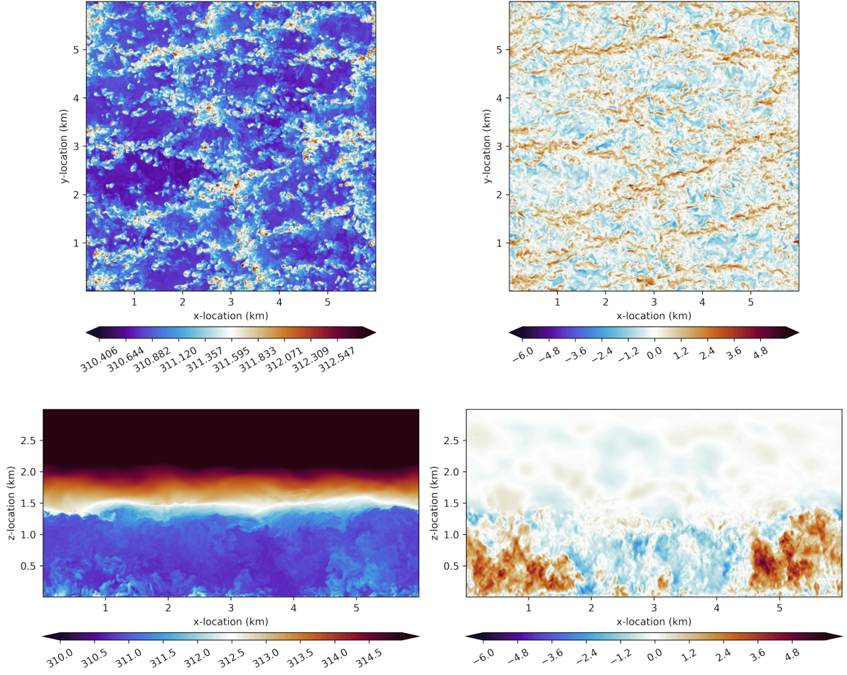
Figure 5. For the convective ABL test case, plots of potential temperature at z = 75 m (top left); vertical velocity at z = 75 m (top right); potential temperature at y = 3 km (bottom left); and vertical velocity at y = 3 km (bottom right) at t = 2 hr.
