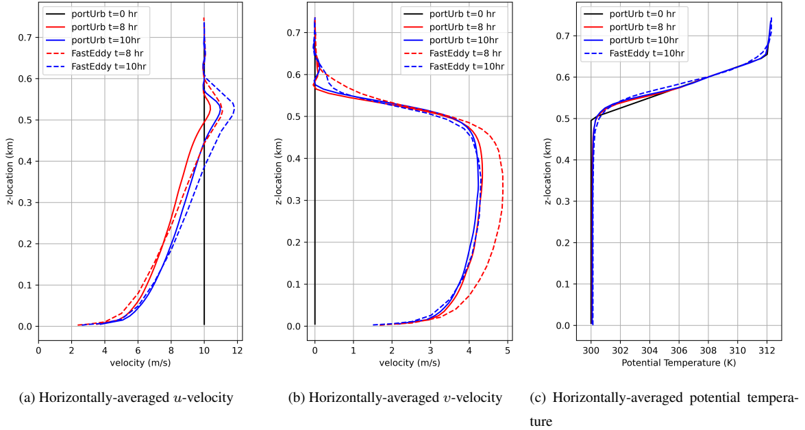
Figure 2. Plots for the neutral ABL test case of horizontally-averaged u -velocity, v -velocity, and potential temperature at different times.
