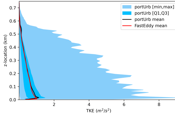
(c) Total TKE (resolved and unresolved)
