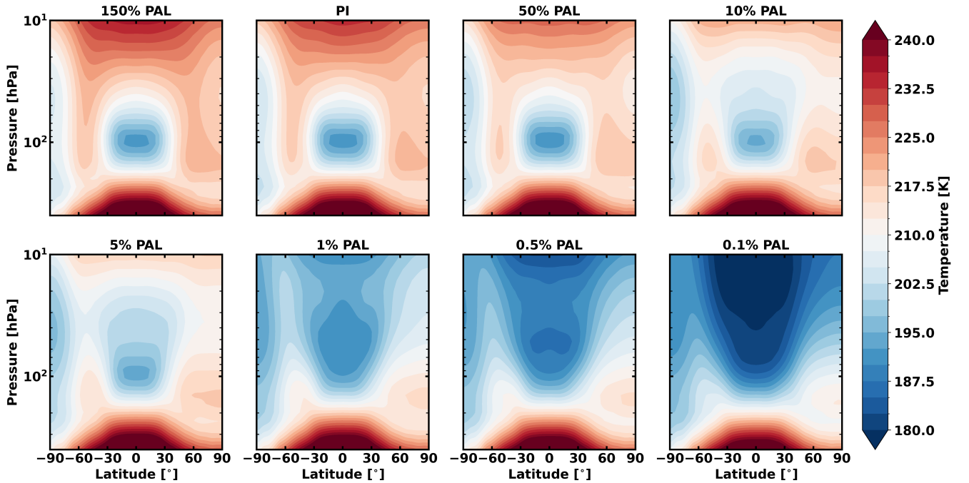
Figure 1. The zonal mean of atmospheric temperature (in K) is shown for simulations with \text{O}_2 mixing ratios between 150% PAL and 0.1% PAL, where \text{O}_2 decreases in abundance from the top left panel to the bottom right panel. The colour bar shows hotter temperatures in red and colder temperatures in blue. The TTL region is \pm 23.4^\circ from the equator and between 70–150 hPa in pressure.
