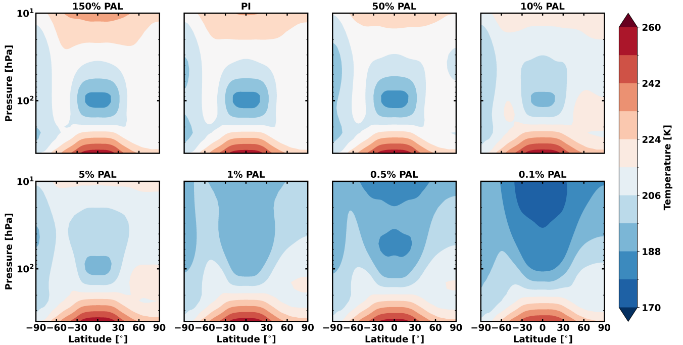
Figure 1. The zonal mean of temperature (in K) is shown for \text{O}_2 mixing ratios between 150% PAL and 0.1% PAL, where \text{O}_2 decreases in abundance from the top left panel to the bottom right panel. The colour bar shows hotter temperatures in red and colder temperatures in blue.
