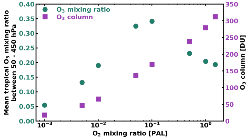
Figure 2. The mean tropical (defined at latitudes \pm 24^\circ from the equator) O_3 mixing ratio between 50–450 hPa is plotted on the left vertical axis in teal circles against the atmospheric mixing ratio of O_2 at the surface in terms of the present atmospheric level (PAL), which is 21% by volume. The total global ozone ( O_3 ) column density in Dobson Units (DU, where 1 \text{ DU} = 2.69 \times 10^{20} \text{ molecules m}^{-2} ) is also plotted in purple squares on the right vertical axis against the atmospheric mixing ratio of O_2 .
