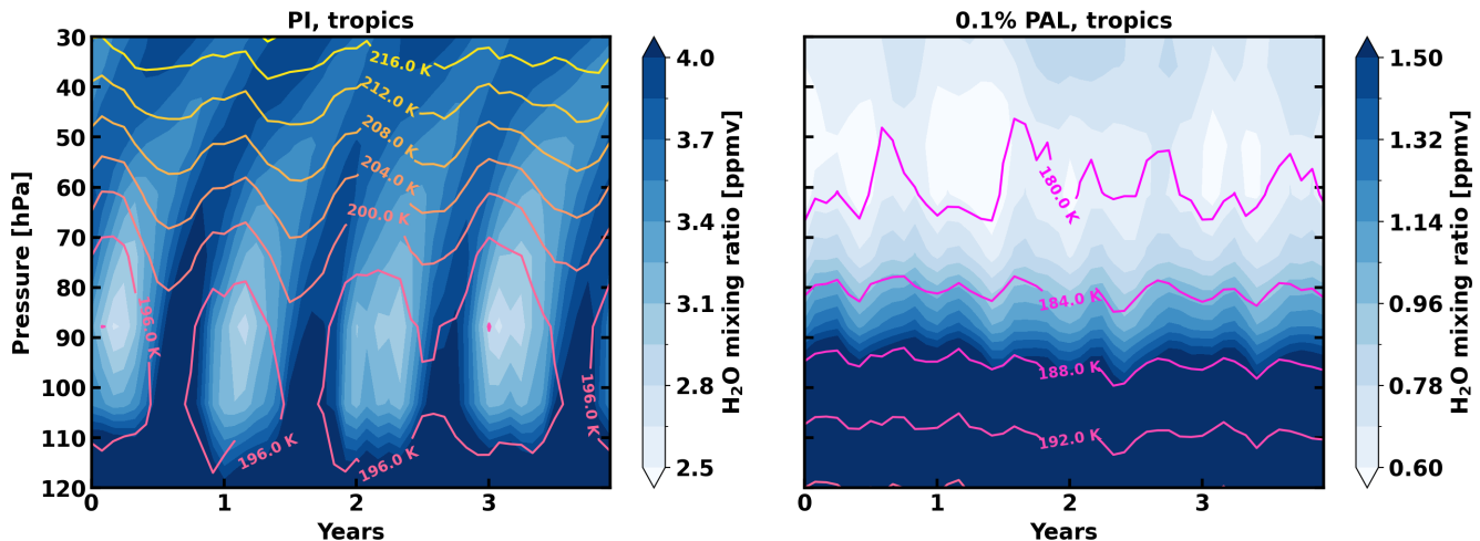
Figure 5. The water vapour mixing ratio in ppmv is shown for the PI scenario ( left ) and the 0.1% PAL scenario ( right ) between pressures of 120 – 30 hPa. Each panel shows four years in a row of each simulation, displaying the zonally averaged and latitudinally weighted H 2 O mixing ratio in the tropics between \pm 24^\circ . Whites show the lowest mixing ratios and darker blues show progressively larger mixing ratios. Note the different scales on each colour bar. The contours show the atmospheric temperature in kelvin, with yellow indicating higher temperatures and magenta indicating lower temperatures.
