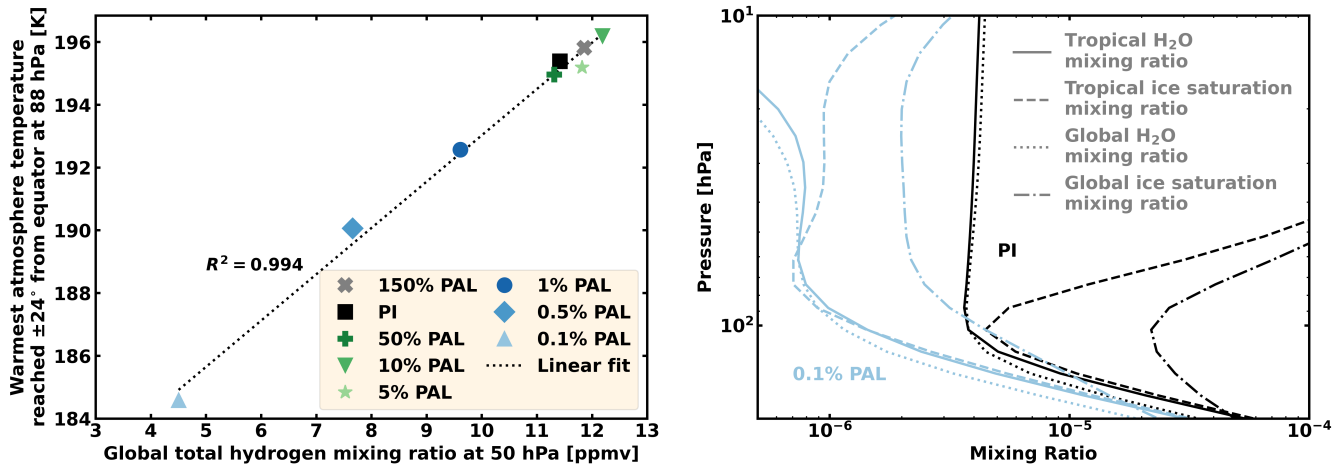
Figure 6. Left: The globally averaged total hydrogen mixing ratio ( f_T(H) ) at 50 hPa is plotted against the warmest temperature reached within \pm 24^\circ (tropical latitudes) from the equator at 88 hPa for each simulation. Linear regression gives a coefficient of determination ( R^2 ) of 0.994, which is showed by the dotted black line. The different O_2 mixing ratios are shown by various markers: 150% PAL (grey cross), PI (black square), 50% PAL (dark green plus), 10% PAL (green downward triangle), 5% PAL (light green star), 1% PAL (dark blue circle), 0.5% PAL (blue diamond), and 0.1% PAL (light blue upward triangle). Right: The H_2O mixing ratio is plotted against pressure for the PI (black) and 0.1% PAL (light blue) simulations, in terms of its tropical (unbroken line) and global (dotted line) average. Also shown is the ice saturation mixing ratio which depends on temperature and pressure and is shown for the tropical (dashed) and global (dash-dotted) average. The tropical average is for latitudes \pm 24^\circ from the equator.
