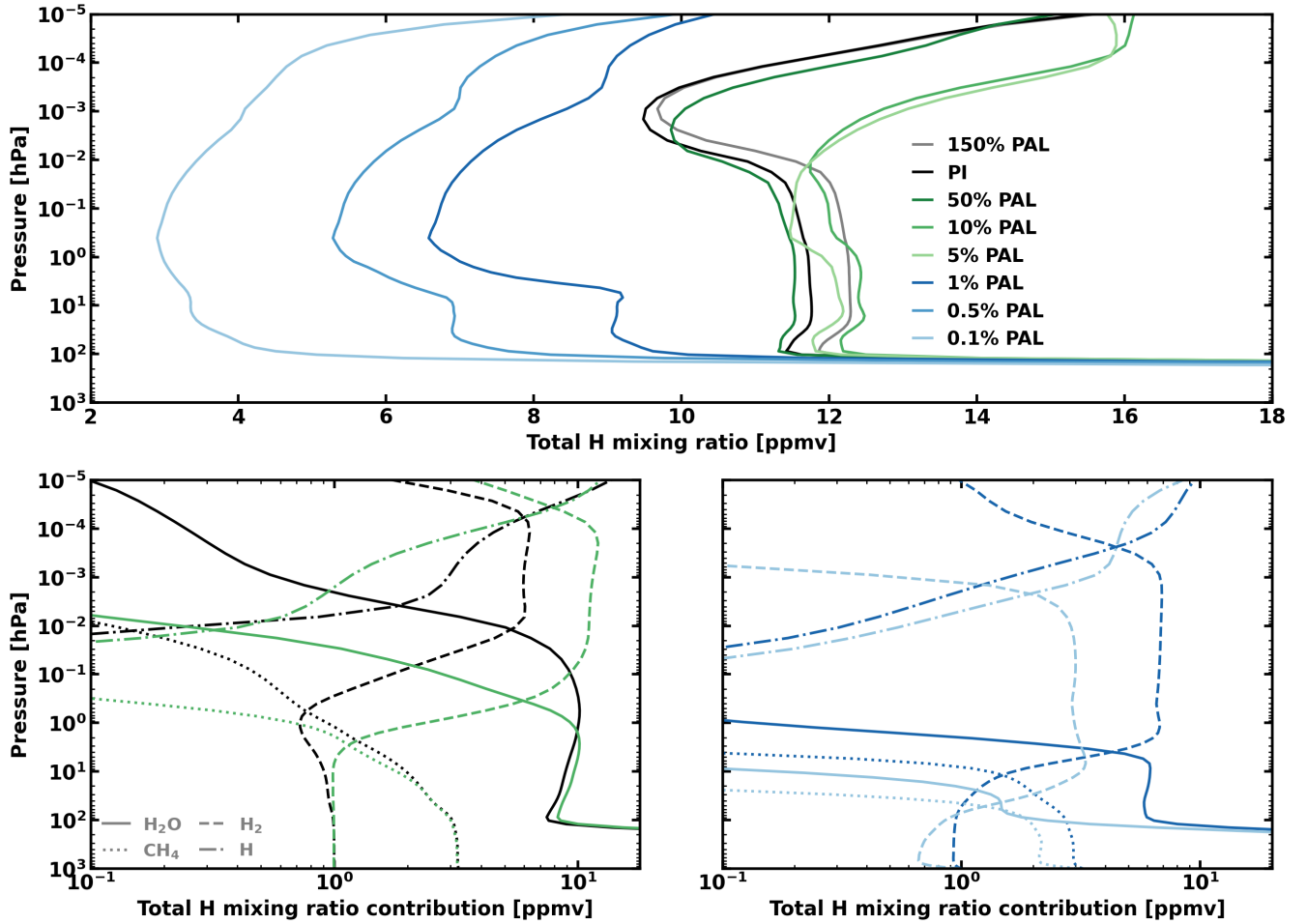
Figure 7. Top: f_T(H) , the total hydrogen mixing ratio is given in parts per million by volume (ppmv) and is shown against pressure for the 150% PAL (grey), PI (black), 50% PAL (dark green), 10% PAL (green), 5% PAL (light green), 1% PAL (dark blue), 0.5% PAL (blue), and 0.1% PAL (light blue) simulations. f_T(H) is calculated using Eq. (2). Hence, the mixing ratio contribution from H, H_2O , H_2 , and CH_4 is multiplied by a factor of 1, 2, 2, and 4, respectively. Bottom left: The total hydrogen mixing ratio contribution from H (dash dotted), H_2 (dashed), H_2O (unbroken), and CH_4 (dotted) is shown for the PI and 10% PAL simulations and bottom right: the 1% PAL and 0.1% PAL simulations.
