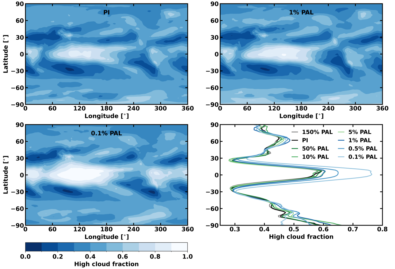
Figure 3. The top left , top right , and bottom left panels show the high cloud fraction as a function of longitude and latitude for the PI, 1% PAL, and 0.1% PAL scenarios, respectively. Bottom right: The high cloud fraction (high clouds are defined as clouds at pressures < 400 hPa) is averaged over longitude and shown as a function of latitude for all the WACCM6 simulations.
