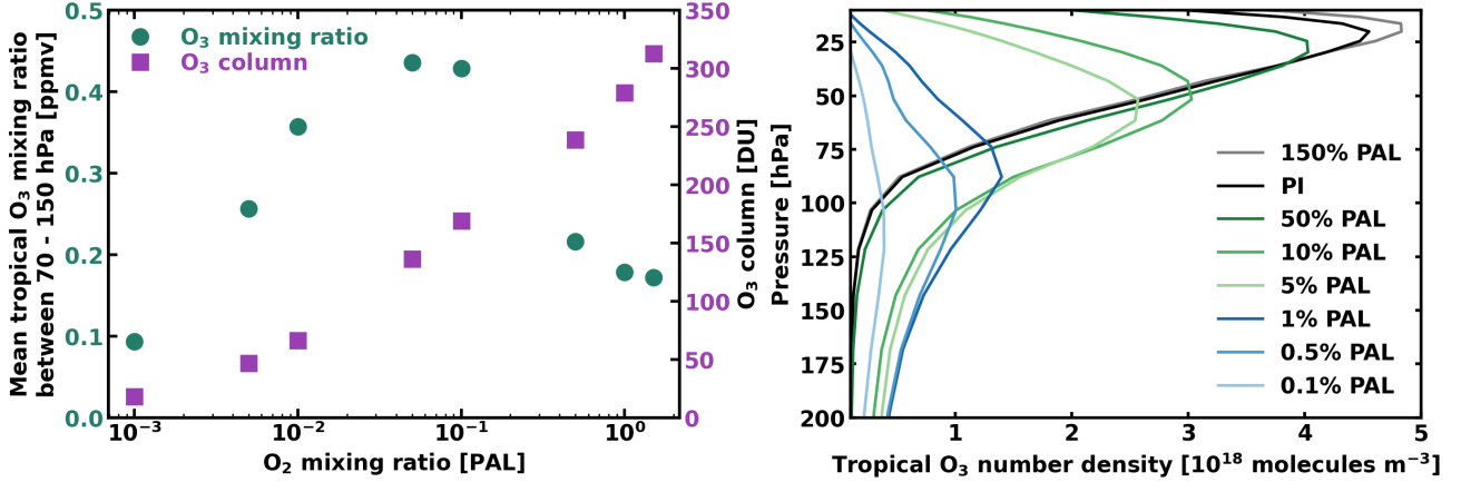
Figure 2. Left: The mean tropical (defined at latitudes \pm 24^\circ from the equator) \text{O}_3 mixing ratio between 70 – 150 hPa is plotted on the left vertical axis in teal circles against the atmospheric mixing ratio of \text{O}_2 at the surface in terms of the present atmospheric level (PAL), which is 21% by volume. The total global ozone ( \text{O}_3 ) column density in Dobson Units (DU, where 1 \text{ DU} = 2.69 \times 10^{20} \text{ molecules m}^{-2} ) is also plotted in purple squares on the right vertical axis against the atmospheric mixing ratio of \text{O}_2 . Right: The \text{O}_3 number density is shown for all eight simulations between 10 – 200 hPa on a linear scale (note the number density does not go to zero at pressures greater than 200 hPa, see Cooke et al., 2022).
