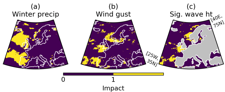
Figure 7: Coincident spatial signals for combined PC1 and PC2 in individual ETC hazards (a) winter total precipitation, (b) winter maximum 10m wind gust and (c) winter maximum significant wave height. Yellow denotes compound impact locations between PC1 and PC2 for each hazard, purple denotes no effect or no compound effect.
