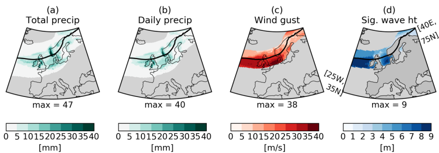
Figure 1: An example ETC footprint lifecycle for the four measures of ETC hazards: (a) cumulative precipitation over the cyclone lifecycle [mm], (b) maximum daily precipitation over lifecycle [mm], (c) local maximum 10m wind gust over lifecycle [m/s], and (d) local maximum significant wave height over lifecycle [m], for Storm Ciara in February 2020 (track shown by black line).
