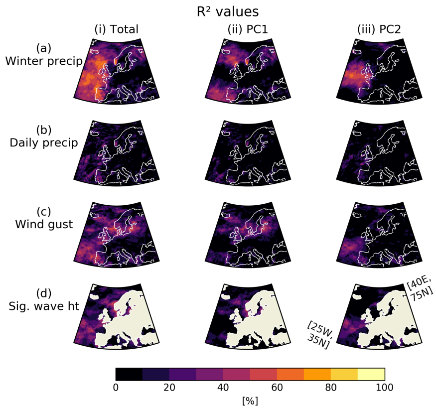
675 Figure 4: R^2 values [%] for the linear regression of ETC winter hazards (a) winter total precipitation, (b) winter daily maximum precipitation, (c) maximum 10m wind gust and (d) maximum significant wave height for (left) PC1+PC2, (middle) PC1 and (right) PC2.
