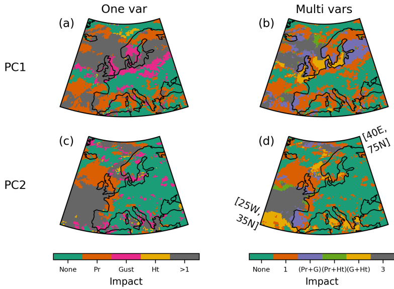
Figure 6: Compound ETC hazards for (a,b) PC1 and (c,d) PC2. (a,c) Regions affected by single hazards (Winter total precipitation, Pr, orange; Maximum 10m wind gust, Gust, Pink; Maximum significant wave height, Ht, yellow), no hazard (green) or >1 hazard (grey); (b,d) regions affected by compound hazards as labelled. Note the hazards may not occur on the same day.
