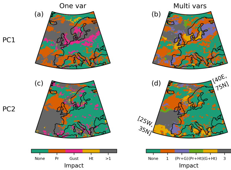
Figure 6: Compound ETC hazards for (a) PC1 and (b) PC2. (Left) Regions affected by single hazards (Winter total precipitation, Pr, orange; Maximum 10m wind gust, Gust, Pink; Maximum significant wave height, Ht, yellow), no hazard (green) or >1 hazard (grey); (right) regions affected by compound hazards as labelled. Note the hazards may not occur on the same day.
