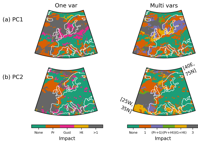
750 Figure 6: Compound ETC hazards for (a) PC1 and (b) PC2. (Left) Regions affected by single hazards (Winter total precipitation, Pr, orange; Maximum 10m wind gust, Gust, Pink; Maximum significant wave height, Ht, yellow), no hazard (green) or >1 hazard (grey); (right) regions affected by compound hazards as labelled. Note the hazards may not occur on the same day.
