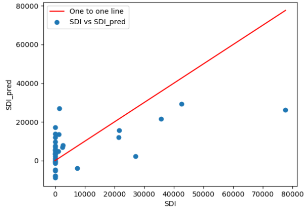
710 Figure 2: Winter cumulative SDI (x-axis) vs. predicted SDI based on the multiple linear regression between SDI and the PC1 and PC2 timeseries (y-axis) at grid box (1.875°W, 52.5°N). Red line shows 1:1 line. Note some of the predicted SDI values are negative when it is bounded at 0.
