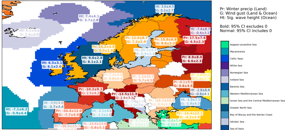
(a) Hazards for European Regions: PC1
