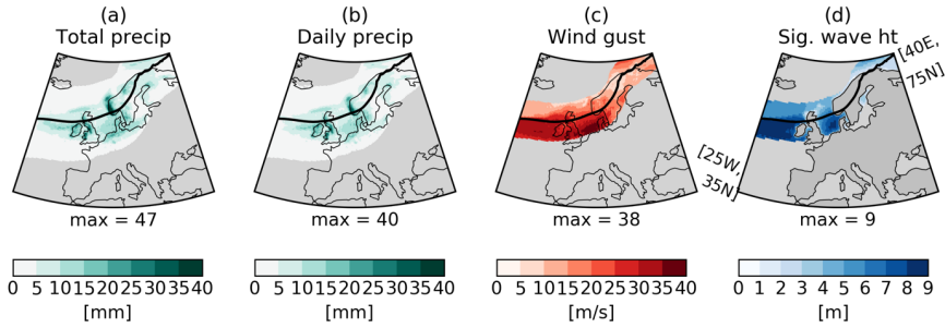
705 Figure 1: An example ETC footprint lifecycle for the four measures of ETC hazards (a) Cumulative precipitation over the cyclone lifetime , (b) maximum daily precipitation over lifetime , (c) local maximum 10m wind gust over lifetime , and (d) local maximum significant wave height over lifetime for Storm Ciara in February 2020 (track shown by black line).
