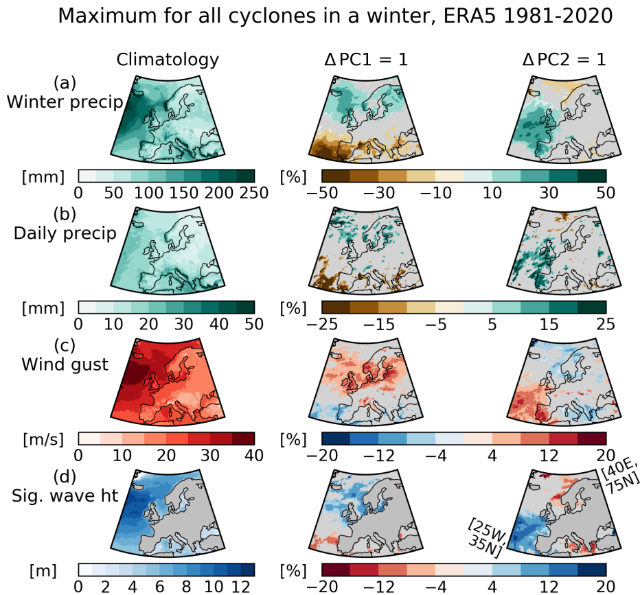
720 Figure 3: Maximum winter ETC hazards for (a) winter total precipitation [mm], (b) winter daily maximum precipitation [mm], (c) 10m wind gust [m/s] and (d) maximum significant wave height [m] for (left column) climatology, (middle column) regression onto PC1 and (right column) regression onto PC2 shown as percentage anomalies from the climatology. Note
