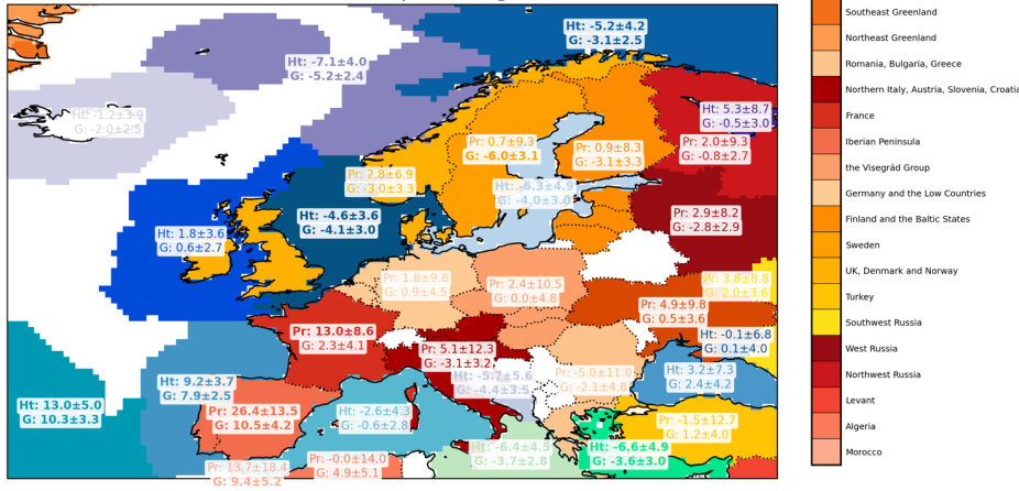
Figure 5: Regional percentage anomalies in winter ETC hazards for land and sea regions as labelled associated with (a) PC1 and (b) PC2. Hazards are winter total precipitation (Pr) and winter maximum wind gust (G) for land regions (red/yellow palette) and significant wave height for regional sea areas (Ht; green/purple/blue palette). Labels denote % anomalies
