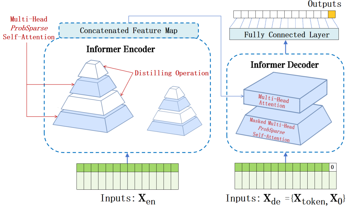
Figure 4. Framework diagram of Informer structure including encoder (Encoder) and decoder (Decoder).
