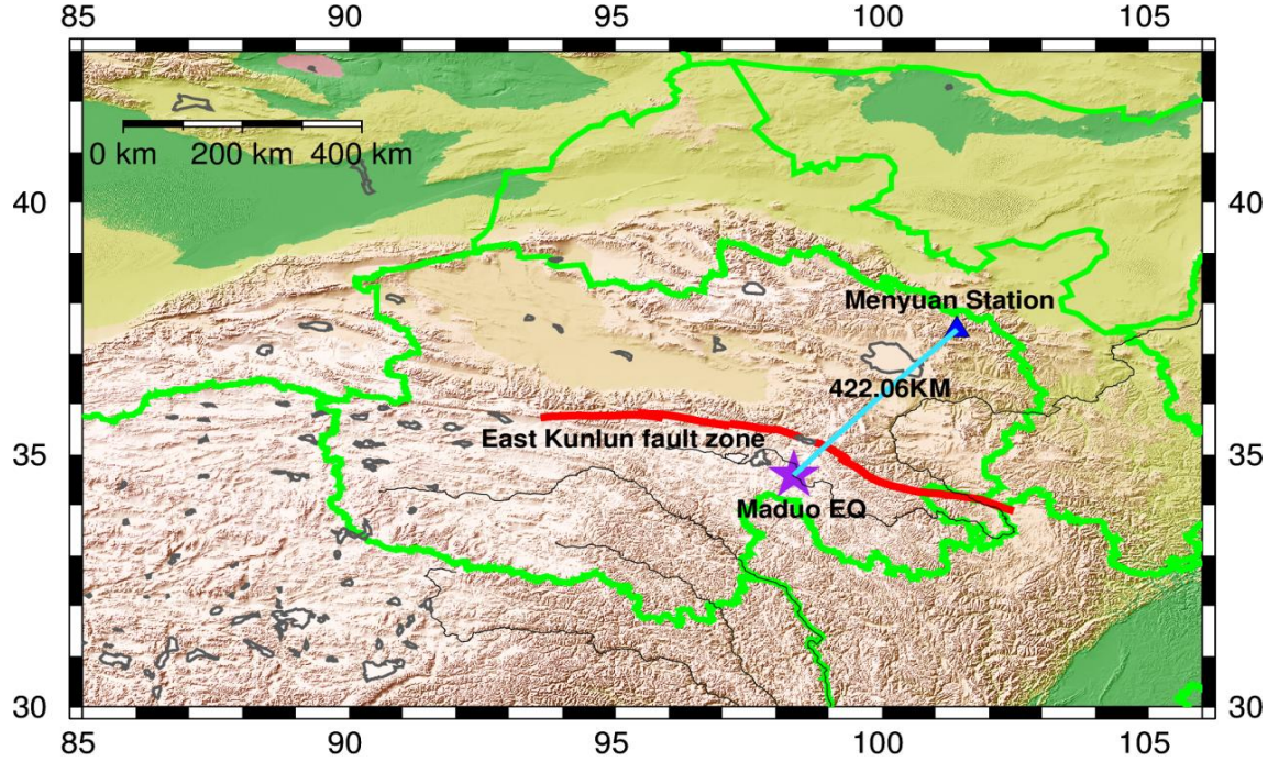
Figure 2. Location of the Mengyuan observatory relative to the epicenter of the Maduo earthquake. The blue triangle represents the location of the borehole strain observatory. The purple star represents the location of the epicenter of the Maduo earthquake, while the red line inscribes the East Kunlun Fault Zone. This map was generated by GMT software, v. 6.0.0rc5 ( https://gmt-china.org/ ).
