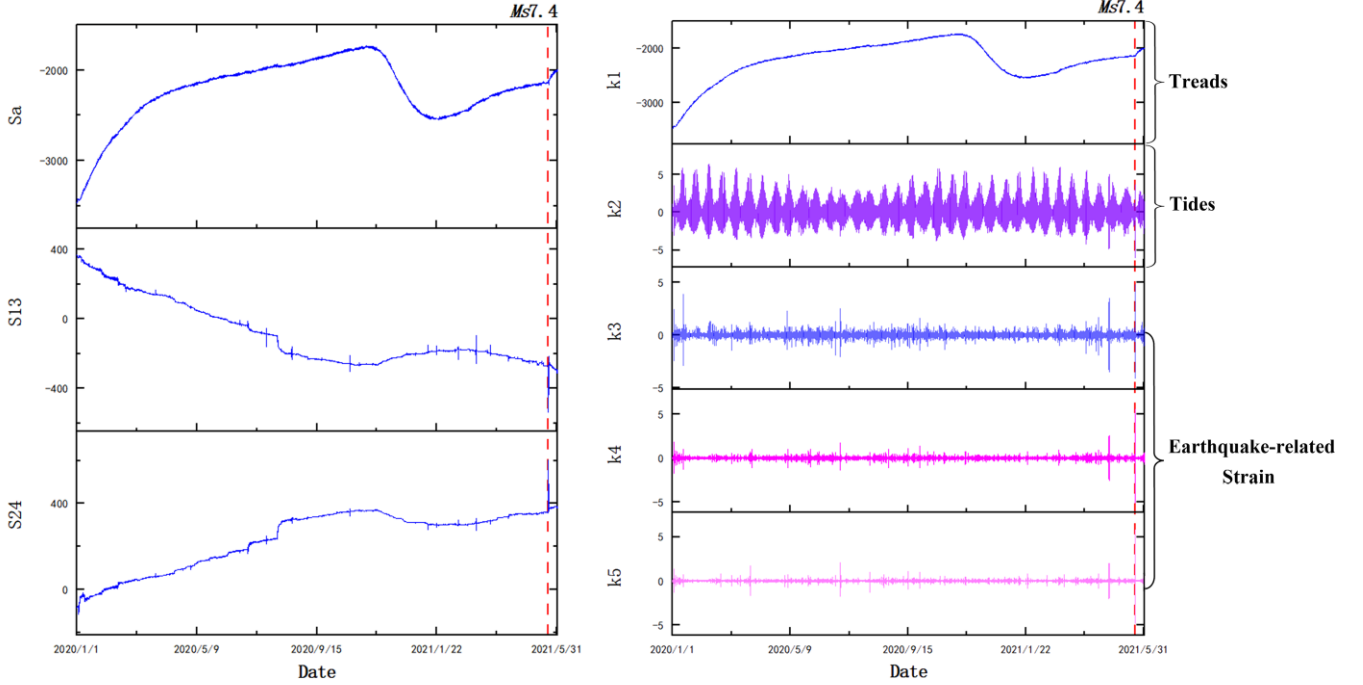
Figure 6. Data for S_a , S_{13} , S_{24} at the Mengyuan station and the results of the SVMD decomposition of S_a . k1 denotes the trend term, k2 denotes the earth tides, and k3, k4, and k5 denote the strains associated with the earthquakes. The red dashed line indicates the date of the earthquake.
