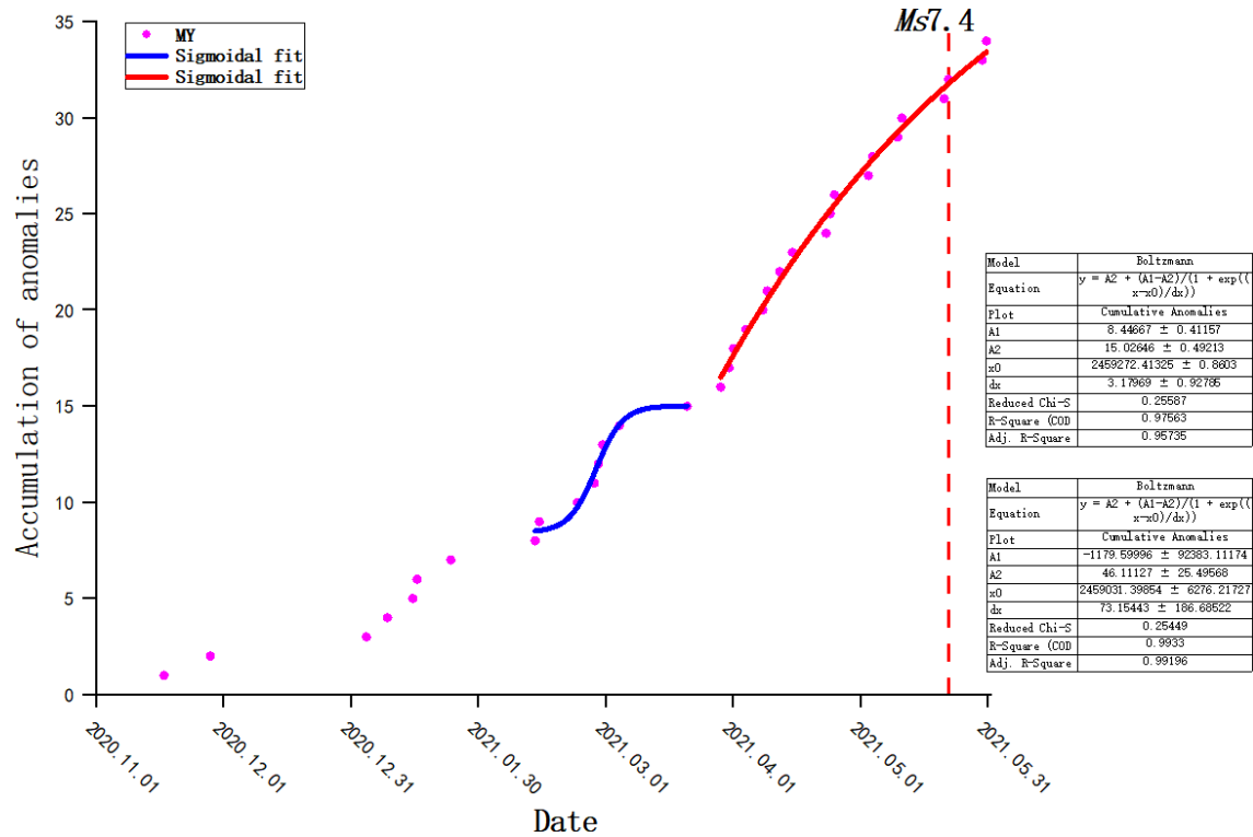
370 Figure 8. Cumulative results of anomalous days of borehole data at Mengyuan station (MY). The red dashed line indicates the date of the earthquake, and the blue and red curves indicate the results of the S-fit function for the first and second phases, respectively.
