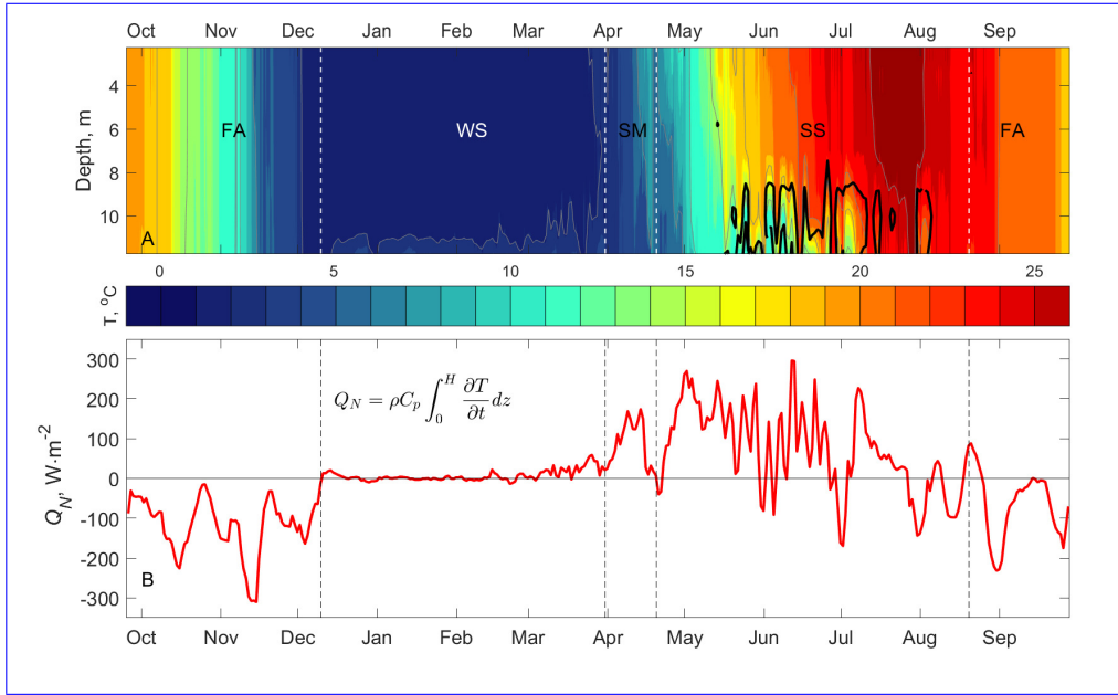
Figure 3. (A) Annual temperature cycle in the North Aral Sea in 2018-2019 . Thick black isoline is the boundary of the bottom stratified layer defined as N^2 > 2 \times 10^{-3} \text{ s}^{-2} . White vertical dashed lines mark the transitions of “lake seasons”: FA refers to fall (autumn) overturn , WS to winter stratification , SM to spring mixing and SS to summer stratification . (B) Rate of change of the lake heat content (Net heat flux into the lake Q_N )
