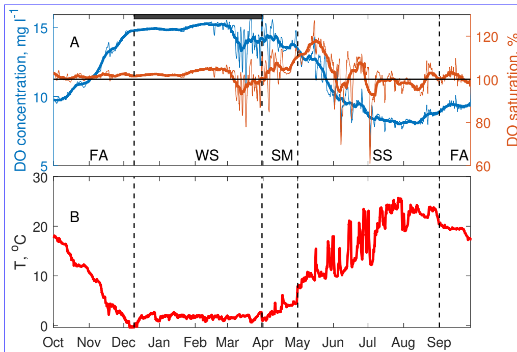
Figure 7. Annual cycle of (A) near-bottom dissolved oxygen at 12 m and (B) Near-bottom water depth temperature . Values of DO concentration in ppm-mg L -1 are shown with blue line, while values of DO saturation are shown with brown line. Black-Thick lines are 5-days running averages filtering out short-term DO oscillations. The gray bar indicates the ice-covered period and the black vertical dashed lines mark the transitions of “lake seasons” : FA refers to fall/autumn overturn, WS to winter stratification, SM to spring mixing and SS to summer stratification.
