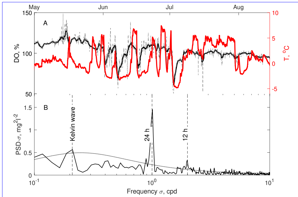
Figure 8. Summer dynamics of the DO content at the bottom slope: (A) Time series of the DO saturation (left axis, black lines) and the near-bottom temperature fluctuations around the summer mean value (right axis, red line). The thick black line is the DO saturation filtered with 24-hours moving average to remove daily primary production/respiration cycle. Thin dashed lines are the original DO saturation data. Coincident temperature and DO saturation drops indicate upwelling of hypoxic deep water at the mooring site. (B) Spectral density of near-bottom DO content oscillation in summer (June-Aug). Vertical dashed lines mark the periods of significant energy-containing oscillations. The Kelvin wave period corresponds to the energy-containing peak of temperature oscillations in Fig. 5. The dotted line shows the lower confidence boundary for the spectral peaks defined as the upper 95 % for the red noise signal (first order autoregressive process) containing the same variance as the observed time series (Gilman et al., 1963).
