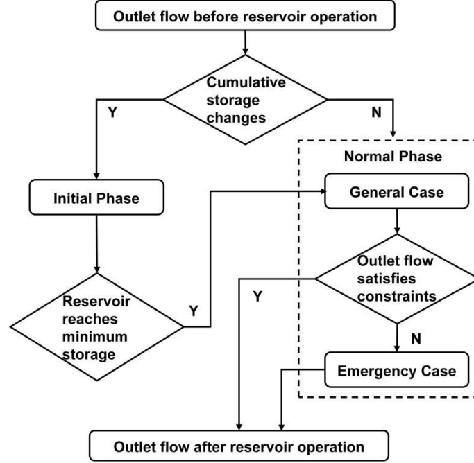
268 269 Figure 2: Flowchart of the constructed reservoir module.
