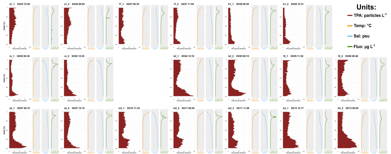
Figure A3. Total particles abundance, temperature, salinity, and fluorescence profiles.
