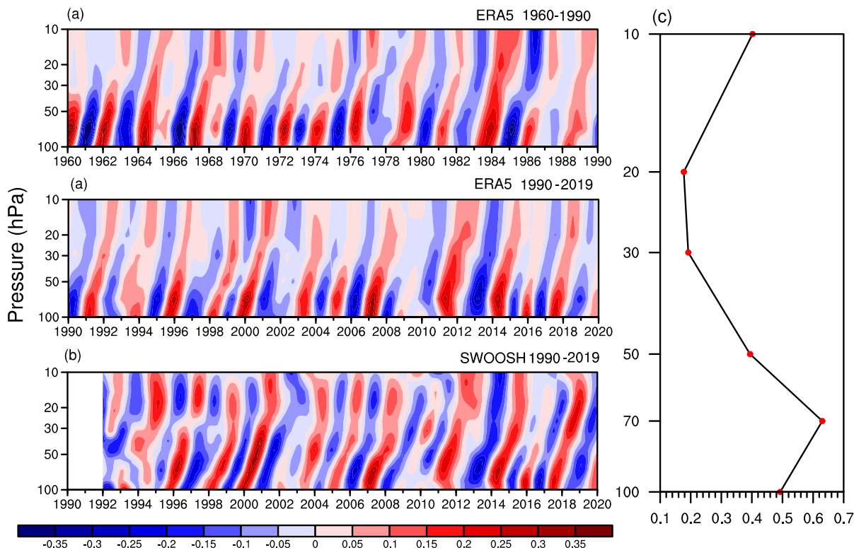
190 Figure 2. (a) Temporal variations of water vapor anomalies averaged over the equator (5°S–5°N) with removed linear trends in the tropical stratosphere from 1960–2019 for ERA5 reanalysis (mass mixing ratio, units: ppm). (b) Water vapor anomalies from 1992–2019 for SWOOSH data (mass mixing ratio, units: ppm). (c) Correlation between SWOOSH and ERA5 at each pressure level. The anomalies are filtered by applying a 15–60-month Butterworth bandpass filter.
