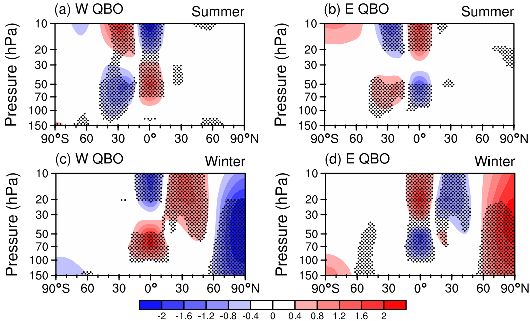
265 Figure 6. Zonal mean temperature anomalies under different QBO phases in northern winter and summer from 1959–2019 for ERA5 reanalysis (unit: K), respectively. (a) Temperature anomalies during the QBO westerly phase in the northern summer. (b) Temperature anomalies during the QBO easterly phase in the northern summer. (c, d) As in a, b but for temperature anomalies for the northern winter. Dots mark the composite anomalies at the 95% confidence level.
