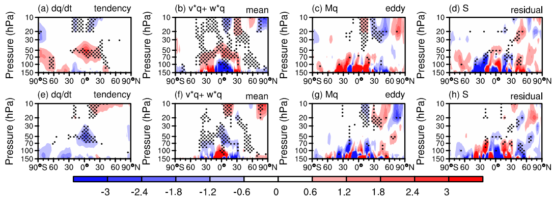
350 Figure 9. Diagnosis of the transformed Eulerian-Mean (TEM) tracer continuity equation in the northern winter from 1959–2019 for ERA5 reanalysis. (a) water vapor tendency during the QBO westerly phase (units: ppb day^{-1} ). (b) The mean advection of water vapor during the QBO westerly phase (ppb day^{-1} ). (c) The eddy transport of water vapor during the QBO westerly phase (ppb day^{-1} ). (d) The residual term of water vapor during the QBO westerly phase (ppb day^{-1} ). (e-h) The same as in a-d but for QBO easterly phase.
