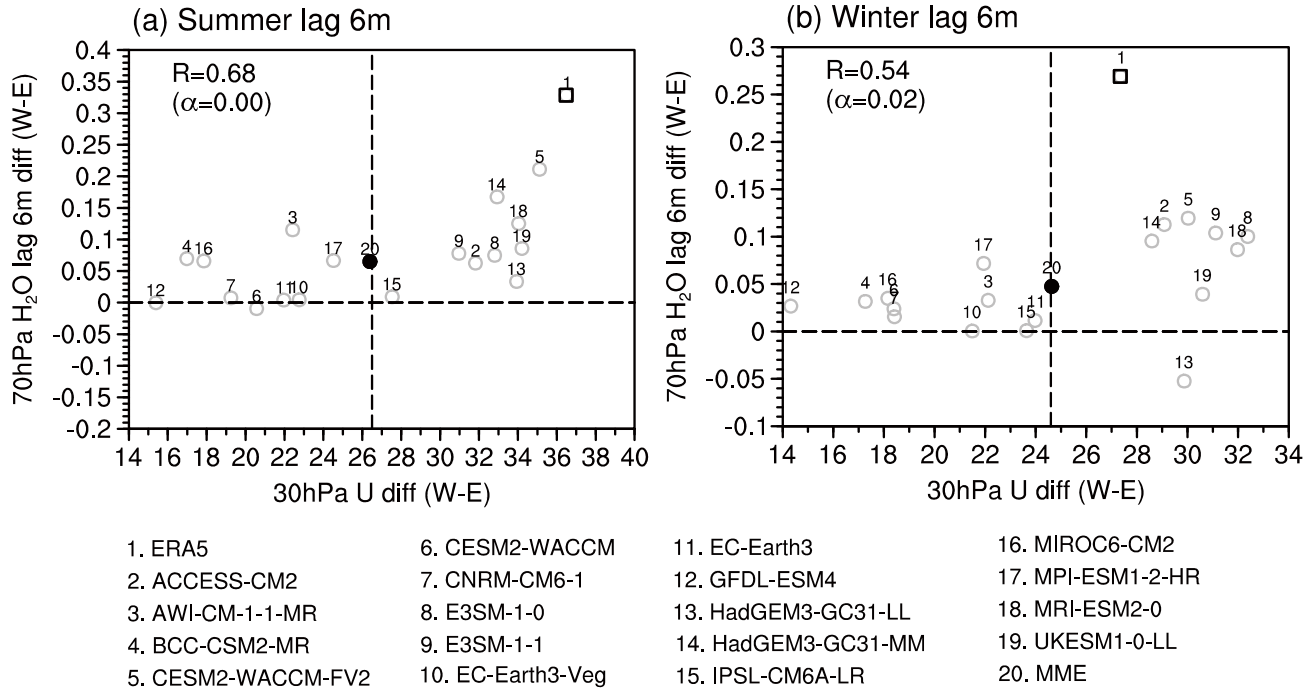
420 Figure 11. Scatter plots of QBO westerly phase minus easterly phase for 30 hPa zonal wind anomalies and 70 hPa water vapor anomalies with a lag of 6 months averaged between 5°S-5°N among 18 CMIP6 models and ERA5 for the northern summer and (b) the northern winter.
