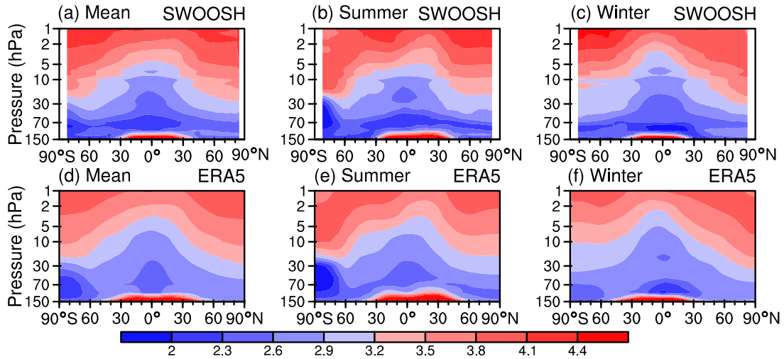
Figure 1. Comparison of stratospheric water vapor from SWOOSH satellite observations and ERA5 reanalysis (unit: ppm). Panels a-c in the first row shows stratospheric water vapor from SWOOSH observations from 1992 to 2019, while panels d-f in the second row display stratospheric water vapor derived from ERA5 reanalysis from 1992 to 2019. (a, d) Multi-year mean stratospheric water vapor mass mixing ratio. (b, e) Mean stratospheric water vapor mass mixing ratio in northern summer. (c, f) Mean stratospheric water vapor mass mixing ratio in northern winter.
