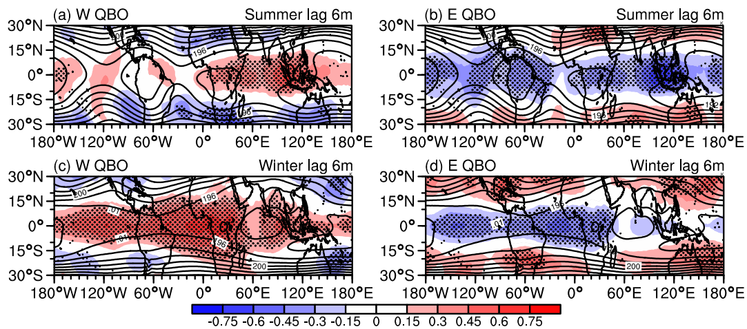
290 Figure 7. Temperature anomalies with a lag of 6 months at 100 hPa under different QBO phases in northern winter and summer from 1959–2019 for ERA5 reanalysis (shadings; unit: K), respectively. (a) Temperature anomalies during the QBO westerly phase in the northern summer. (b) Temperature anomalies during the QBO easterly phase in the northern summer. (c, d) As in a, b but for temperature anomalies following the QBO in the northern winter. Contours show the temperature climatology in winter and summer (contour interval: 2), and dots mark the composite anomalies at the 95% confidence level.
