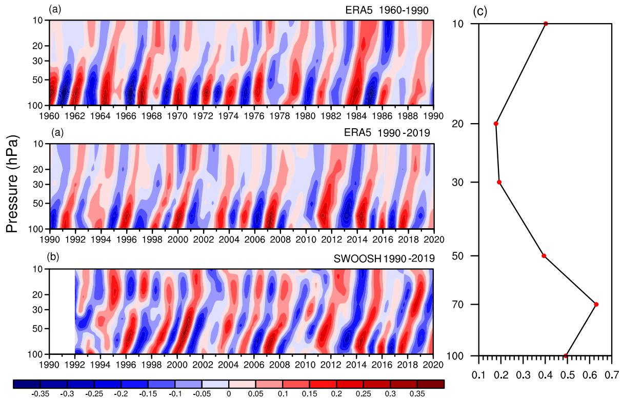
Figure 2. (a) Temporal variations of water vapor anomalies averaged over the equator (5°S–5°N) with removed linear trends in the tropical stratosphere from 1960–2019 for ERA5 reanalysis (mass mixing ratio, units: ppm). (b) Water vapor anomalies from 1990–2019 for SWOOSH data (mass mixing ratio, units: ppm). (c) The normalized standard deviation of the differences between SWOOSH and ERA5 at each pressure level. The anomalies are filtered by applying a 15–60-month Butterworth bandpass filter.
