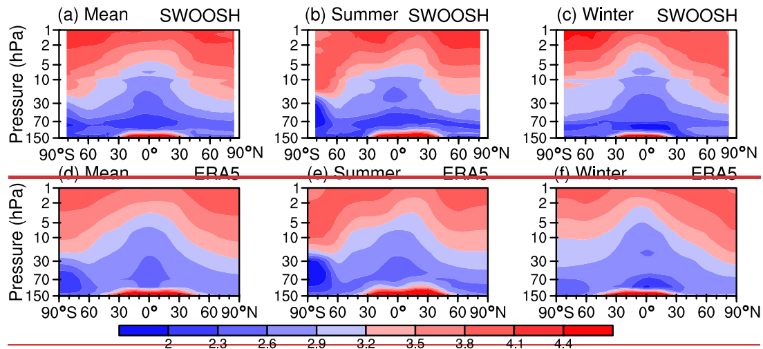
145 Figure 1. Comparative analysis of SWV from SWOOSH satellite observations and ERA5 reanalysis during 1992–2019 (unit: ppm). Panels a–c in the first row show SWV from SWOOSH observations, while panels d–f in the second row display SWV derived from ERA5 reanalysis. (a, d) Multi-year mean SWV mass mixing ratio. (b, e) Mean SWV mass mixing ratio in northern summer. (c, f) Mean SWV mass mixing ratio in northern winter.
