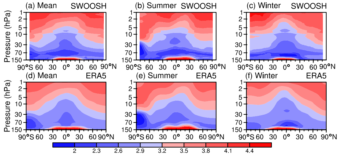
Figure 1. Comparison of stratospheric water vapor from SWOOSH satellite observations and ERA5 reanalysis data (unit: ppm). Panels a-c in the first row shows stratospheric water vapor from SWOOSH observations from 1992 to 2019, while panels d-f in the second row display stratospheric water vapor derived from ERA5 reanalysis from 1992 to 2019. (a, d) Multi-year mean stratospheric
