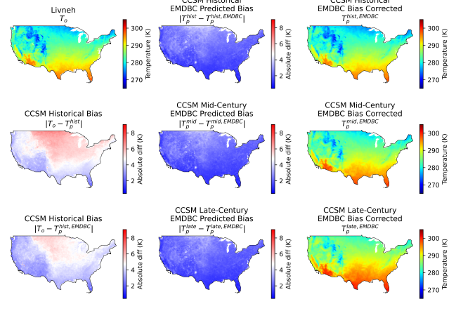
Figure 9. Temperature and temperature bias comparisons over CONUS before and after applying EMDBC. Left: Observed temperature (Livneh), WRF-CCSM average daily absolute bias, and EMDBC-corrected WRF-CCSM average daily absolute bias. Middle: Magnitude of EMDBC correction in historical, mid-century, and late-century timeframes. Right: EMDBC-corrected temperatures for WRF-CCSM historical, mid-century, and late-century periods.
