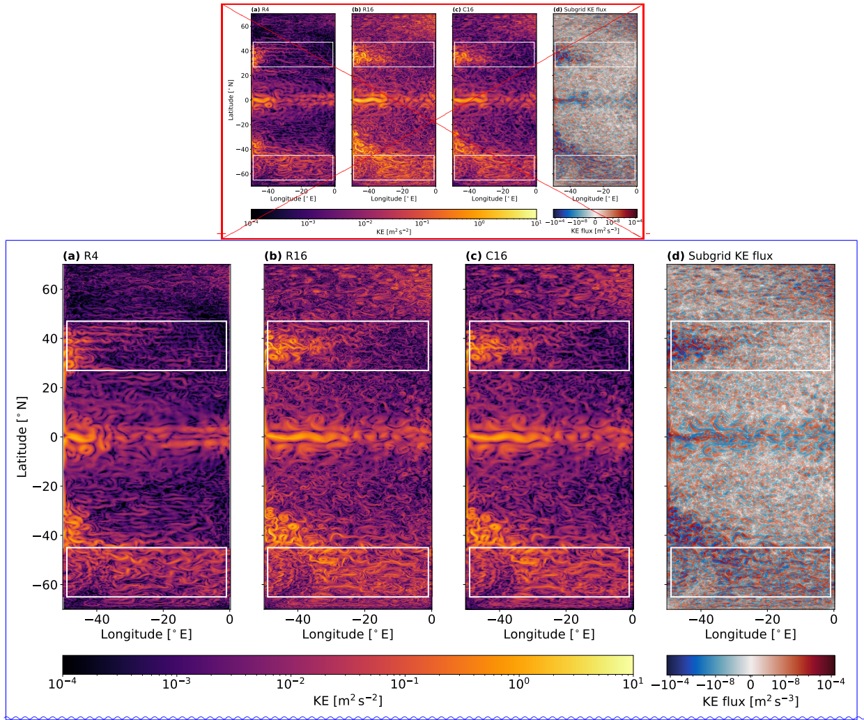
Figure 9. Surface kinetic energy snapshots for the (a) R4, (b) R16 and (c) C16 reference experiment. Panel (d) shows the KE tendency per unit mass due to the subfilter eddy source term of the C16 experiment. White boxes indicate the Gulf-Stream (top) and Southern Ocean (bottom) region. All snapshots are computed for the last time step after 23–30 years of simulation.
