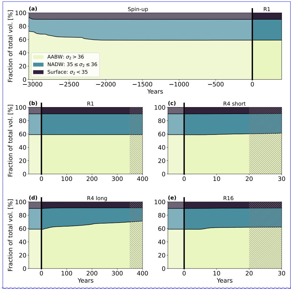
Figure E1. Time series of the water masses partition based on an idealized definition of Antarctic Bottom Water ( \sigma_2 > 36 \text{ kg m}^{-3} ), North Atlantic Deep Water ( 35 \text{ kg m}^{-3} < \sigma_2 < 36 \text{ kg m}^{-3} ) and surface water ( \sigma_2 < 35 \text{ kg m}^{-3} ). Values are given as percentages of the total water volume. The 3000 years of spin-up at 1^\circ horizontal resolution (panel (a)) is continued as experiment R1 for 400 years (panel (b)). R4 (panel (c)) and R16 (panel (e)) are initialized from the same stratification field as R1, indicated by the thick black line. The R4 experiment is continued for 400 years (panel (d)). Hatched areas indicate the period of data-collection for each experiment, corresponding to the gray boxes in Fig. 3.
