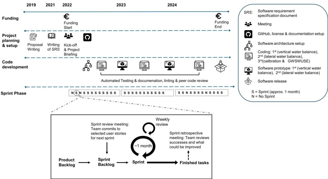
185 Figure 1: Timeline and agile project management setup for reprogramming of WaterGAP in the ReWaterGAP project.
