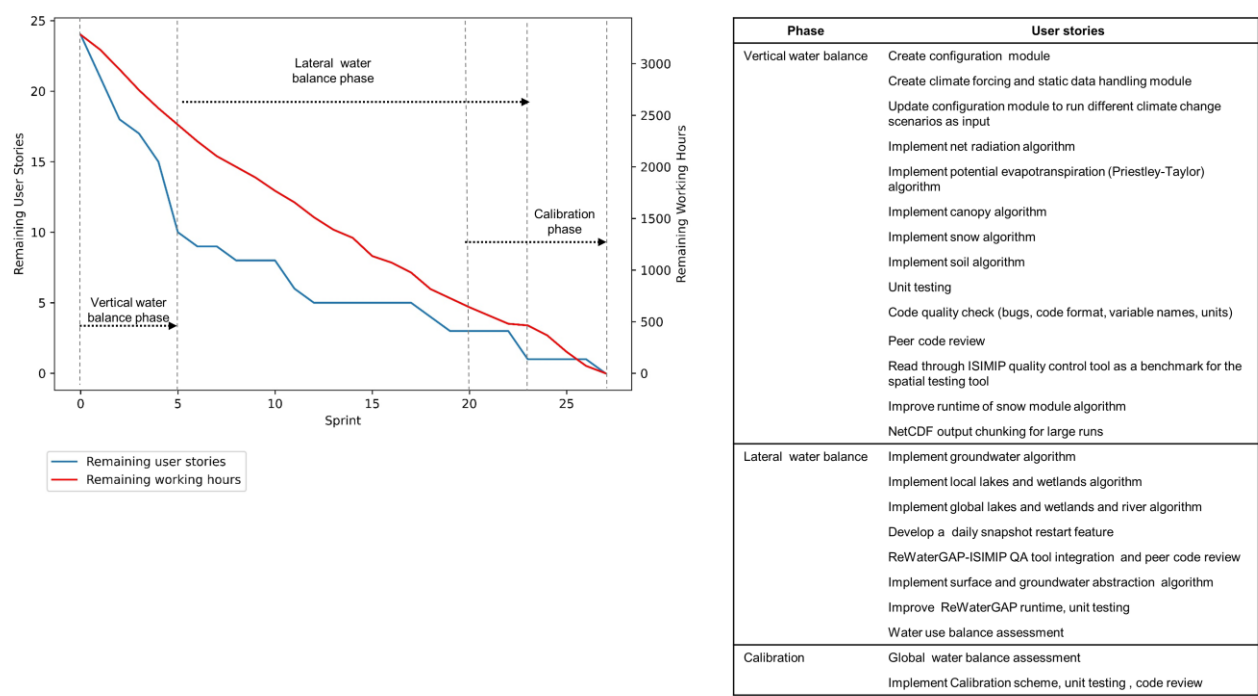
Figure 2: Cumulative plot of remaining user stories and corresponding working hours over 27 sprints (left), and a table of 24 major user stories (right, also see progress_taking.xlsx in supplement), grouped by their corresponding phases: vertical water balance, lateral water balance, and calibration.
