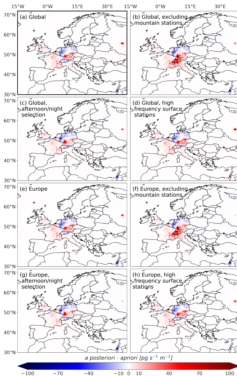
Figure E2. Inversions increments (a posteriori - a priori) averaged over the study period (2005-2021), shown for different observation datasets: (a) the full global dataset, (b) the global dataset excluding mountain stations, (c) the global dataset selecting night/afternoon observations, (d) the global dataset using exclusively high-frequency surface observations, (e) the European dataset, a subset of the global dataset focused on observations in and around Europe, (f) the European dataset excluding mountain stations, (g) the European dataset selecting night/afternoon observations (h) the European dataset using exclusively high-frequency surface observations.
