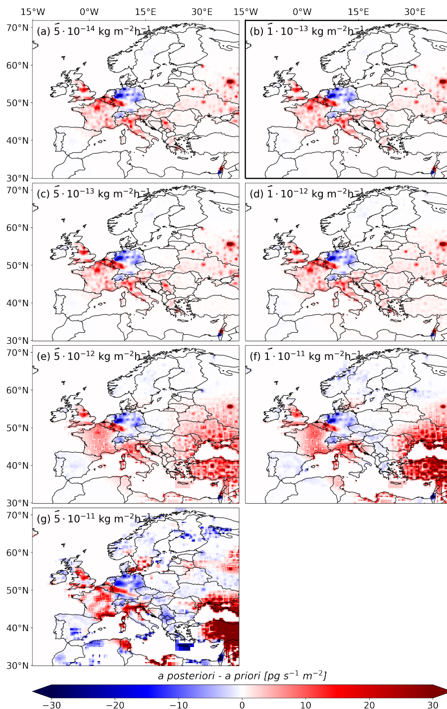
Figure C4. Inversions increments (a posteriori - a priori) for the year 2012, shown for different tested minimal a priori emission uncertainty values (a) 5 \times 10^{-14} \text{ kg m}^{-2} \text{h}^{-1} , (b) 1 \times 10^{-13} \text{ kg m}^{-2} \text{h}^{-1} , (c) 5 \times 10^{-13} \text{ kg m}^{-2} \text{h}^{-1} , (d) 1 \times 10^{-12} \text{ kg m}^{-2} \text{h}^{-1} , (e) 5 \times 10^{-12} \text{ kg m}^{-2} \text{h}^{-1} , (f) 1 \times 10^{-11} \text{ kg m}^{-2} \text{h}^{-1} , and (g) 5 \times 10^{-11} \text{ kg m}^{-2} \text{h}^{-1} .
