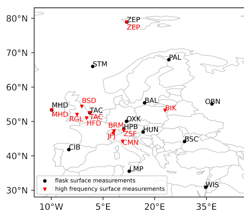
Figure 1. Locations of the observation stations in and around Europe. Stations with continuous surface measurements (BIK, BSD, BRM, CMN, HFD, JFJ, MHD, RGL, TAC, ZEP, ZSF) are represented with red triangles, while surface flask measurements (BAL, BSC, CIB, HPB, HUN, LMP, OBN, OXK, MHD, PAL, STM, TAC, WIS, ZEP) are shown with black dots.
