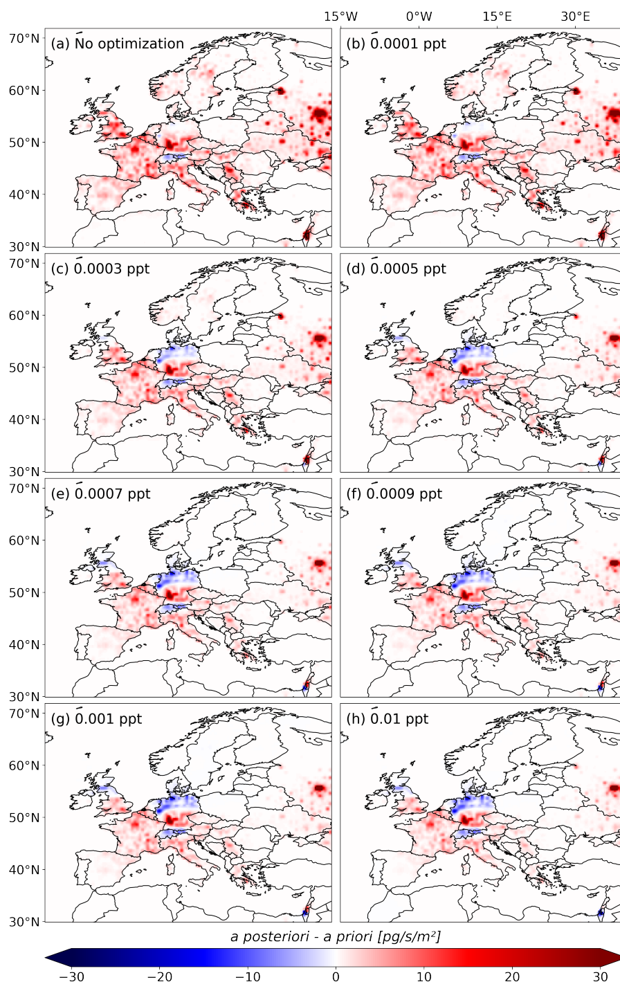
Figure G5. Inversions increments (a posteriori - a priori) averaged over the study period (2005-2021), shown for various baseline uncertainty values: (a) no optimization, (b) 0.0001 ppt (c) 0.0003 ppt, and (d) 0.0005 ppt, (e) 0.0007 ppt, (f) 0.0009 ppt, (g) 0.001 ppt, (h) 0.01 ppt
