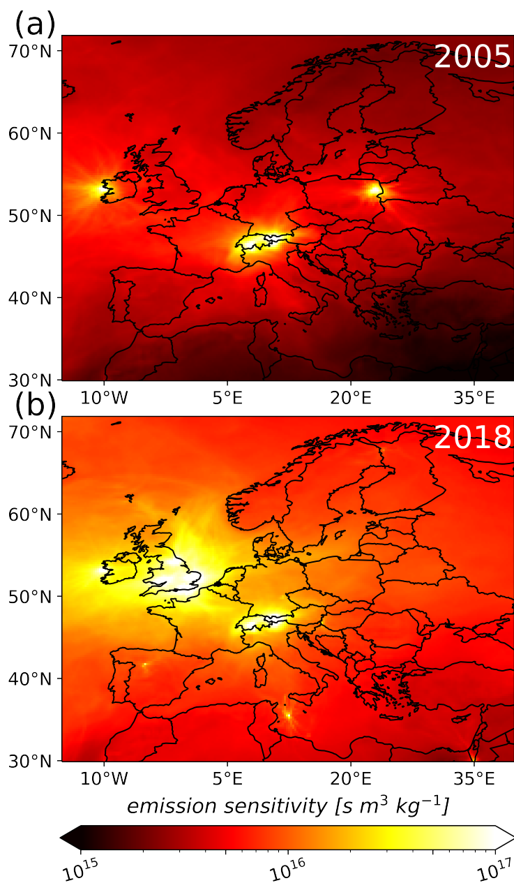
Figure 2. Simulated emission sensitivities for the years 2005 and 2018 in Europe. The displayed values represent the annual sum of FLEX-PART calculations. As a result, sites with frequent online observations carry more weight than those relying on flask measurements or observations from mobile platforms.
