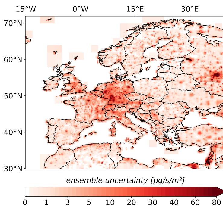
Figure A1. Ensemble uncertainty, presented as the 2\sigma uncertainty across all a posteriori emissions of the Monte Carlo ensemble at each grid cell
