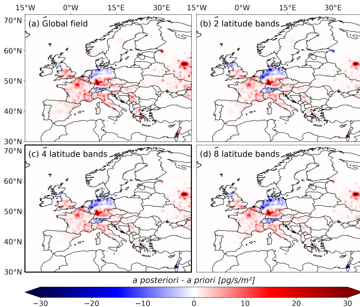
Figure G2. Inversions increments (a posteriori - a priori) averaged over the study period (2005-2021), shown for various spatial resolutions of aggregated baseline contributions for the baseline optimization: (a) the whole field, (b) 2 latitudinal bands, (c) 4 latitudinal bands, and (d) 8 latitudinal bands
