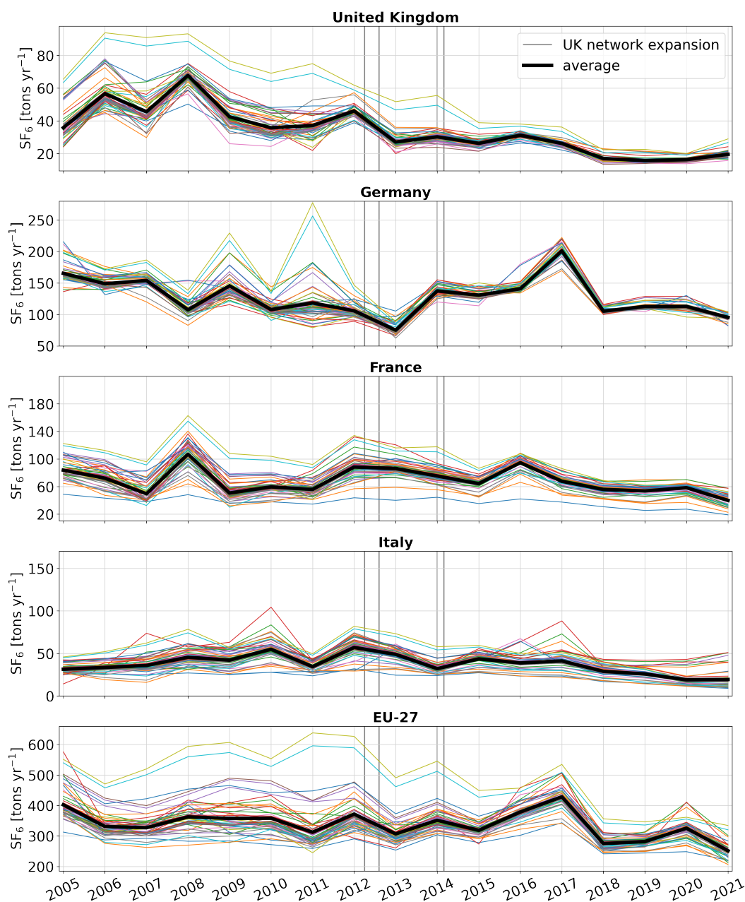
Figure 11. Annual emission time series for (a) the United Kingdom, (b) Germany, (c) France, (d) Italy, and (e) the EU-27. The colored lines represent the inversion results of all sensitivity tests and the solid black lines represent the average a posteriori emissions across all performed tests. The vertical grey lines indicate the times when additional observational data from the expansion of the UK network became available. The vertical grey lines indicate the times when additional observational data from the expansion of the UK network became available.
