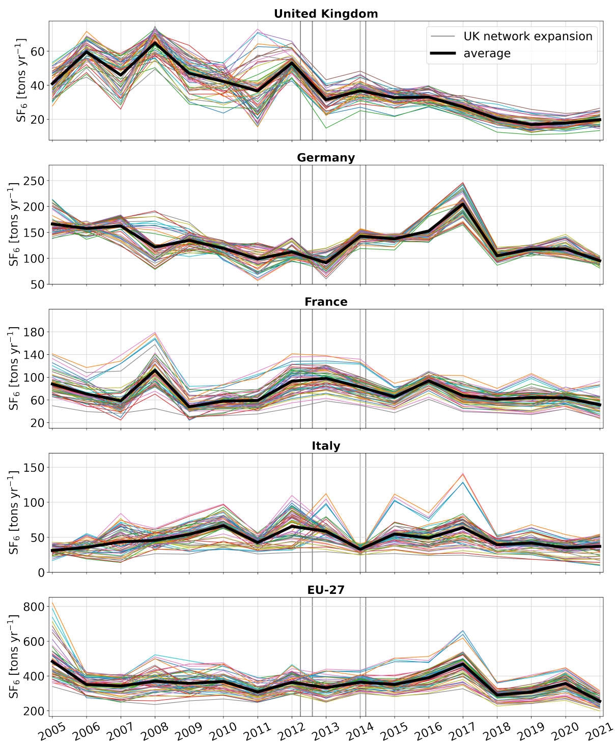
Figure A2. Annual emission time series for (a) the United Kingdom, (b) Germany, (c) France, (d) Italy, and (e) the EU-27. The colored lines represent all inversion results using the Monte Carlo-based settings. The solid black lines represent the average a posteriori emissions across all performed inversions,
