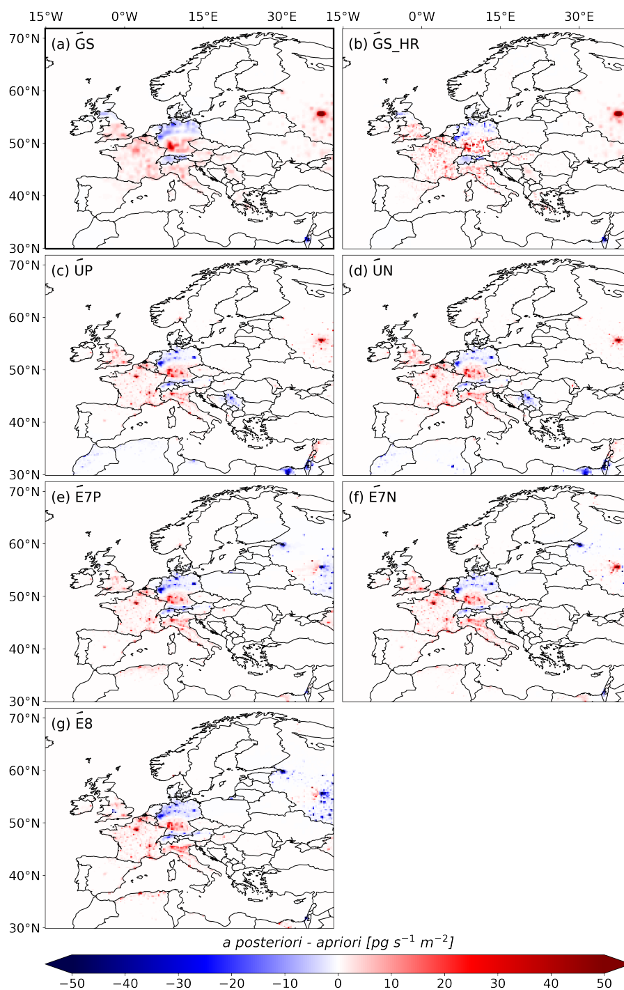
Figure B1. Inversions increments (a posteriori - a priori) averaged over the entire study period (2005-2021), shown for different a priori emission inventories: (a) GS, (b) GS_HR, (c) UP, (d) UN, (e) E7P, (f) E7N, (g) E8.
