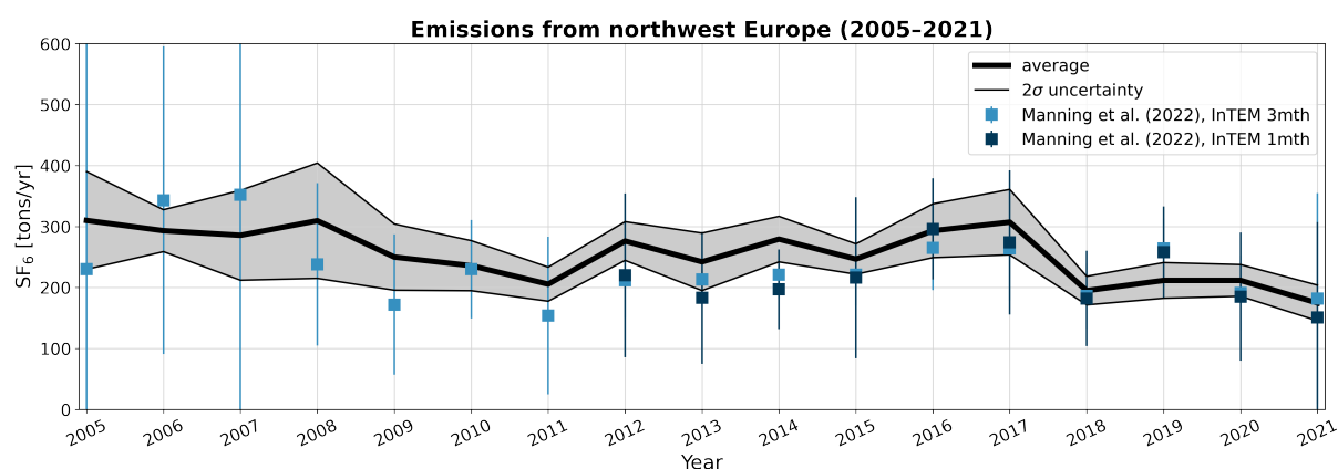
Figure A3. Annual emission time series for northwest Europe. The solid black lines represent the average a posteriori emissions across all performed inversions, with with a 2- \sigma uncertainty range for each year for each year. The blue and black squares represent the results from Manning et al. (2022) using the InTEM model with inversion time frames set to 3- and 1-months, respectively
