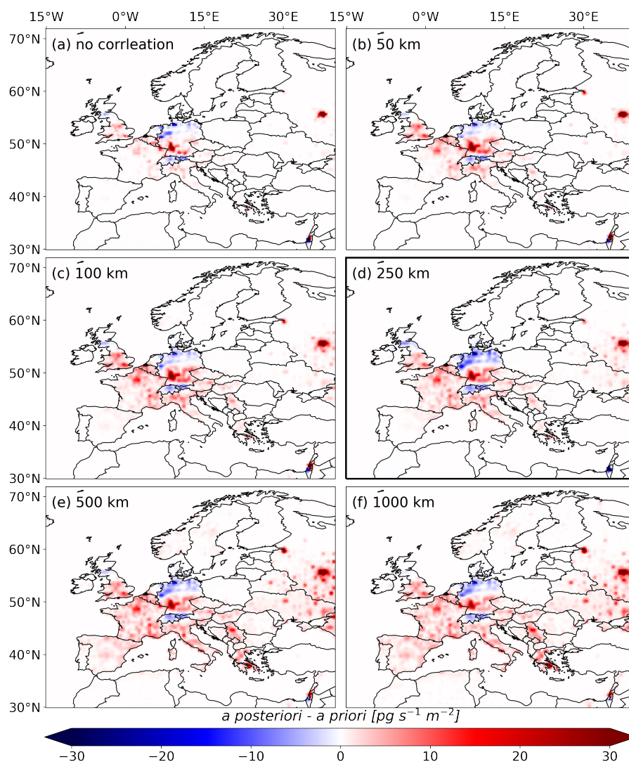
Figure D2. Inversions increments (a posteriori - a priori) averaged over the study period (2005-2021), shown for different spatial scale lengths for the a priori emission uncertainty correlation: (a) no correlation, (b) 50 km, (c) 100 km, (d) 250 km, (e) 500 km, and (f) 1000 km
