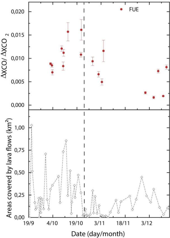
1115 1116 Figure D1: Comparison between the time series of \Delta XCO/\Delta XCO_2 ratios obtained over the whole eruptive period at 1117 FUE and the daily covered area by the lava flows derived from the daily Copernicus EMSR546 mapping 1118 (COPERNICUS EMERGENCY MANAGEMENT SERVICE | Copernicus EMS - Mapping).
