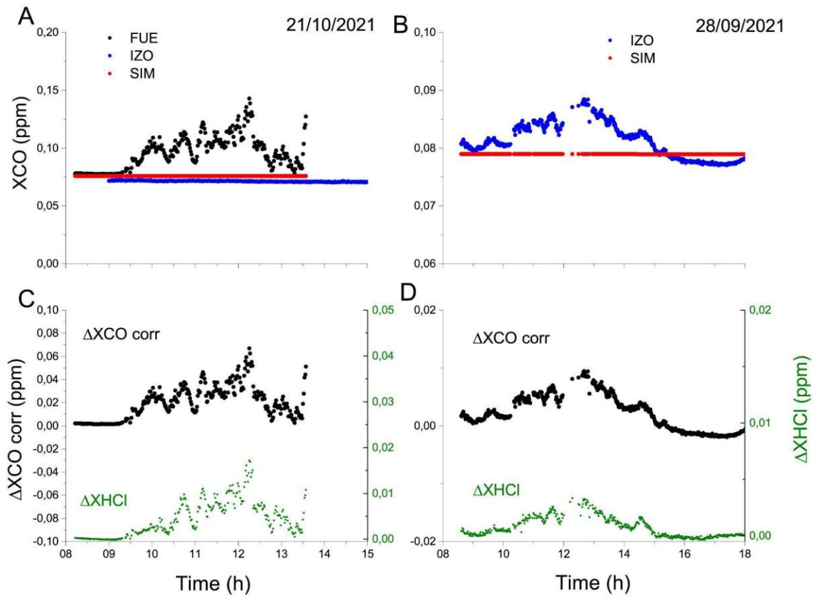
1053 1054 Figure A4: Same as A3 for CO. For CO the procedure only consisted in removing the long-term trend, estimated 1055 from the long-term IZO daily average time series.
