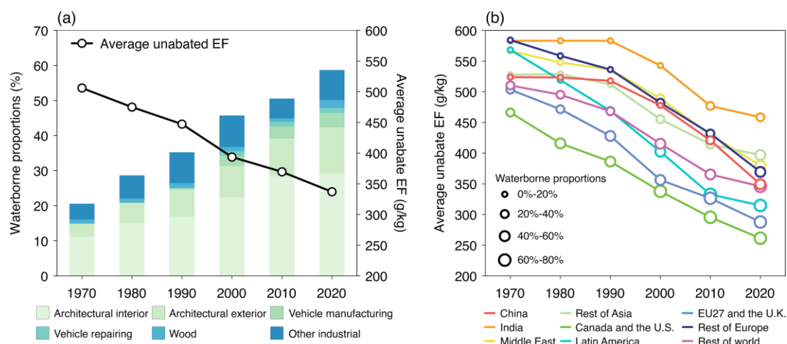
Figure 4. (a) Waterborne proportions of global paint use accumulated by application purpose (colored bars) and changes in global average unabated emission factors (black line with circles). (b) Changes in regional average unabated emission factors. The sizes of the circles represent regional waterborne proportions.
