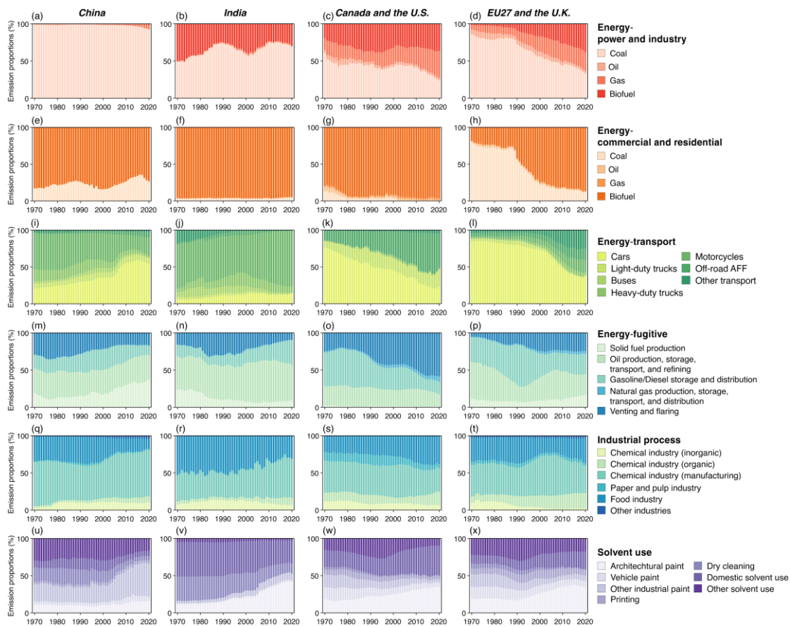
505 Figure 8. The distributions of regional NMVOC emissions by detailed fuel type or sector for (a-d) energy-power and industry, (e-h) energy-commercial and residential, (i-l) energy-transport, (m-p) energy-fugitive emissions, (q-t) industrial process, and (u-x) solvent use in China, India, Canada and the U.S., and EU27 and the U.K. from 1970 to 2020.
