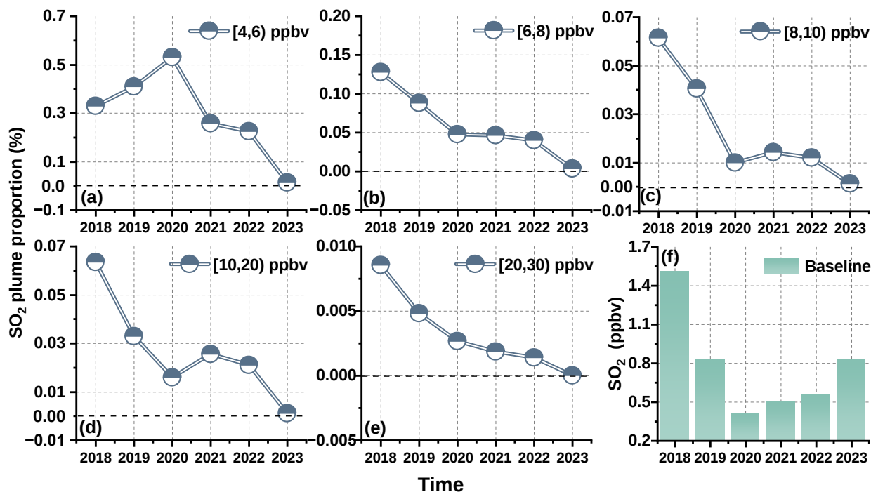
Figure 6: Yearly variation in SO 2 plume proportions and baseline level from 2018 to 2023. (a-e) Number of SO 2 -rich plumes within different concentration ranges divided by the total valid spectra for each year. (f) Annual baseline concentrations of SO 2 obtained through the BEADs algorithm.
