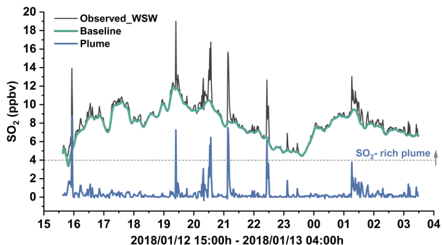
235 Figure 5: Time series of baseline trends and SO 2 -rich plume signals separated from Observed_WSW using the BEADs algorithm. The black line represents the DOAS observed SO 2 concentrations, the green line indicates the baseline, and the blue line corresponds to plumes sequence extracted using the BEADs algorithm. The dashed line marks the threshold for identifying SO 2 -rich plumes.
