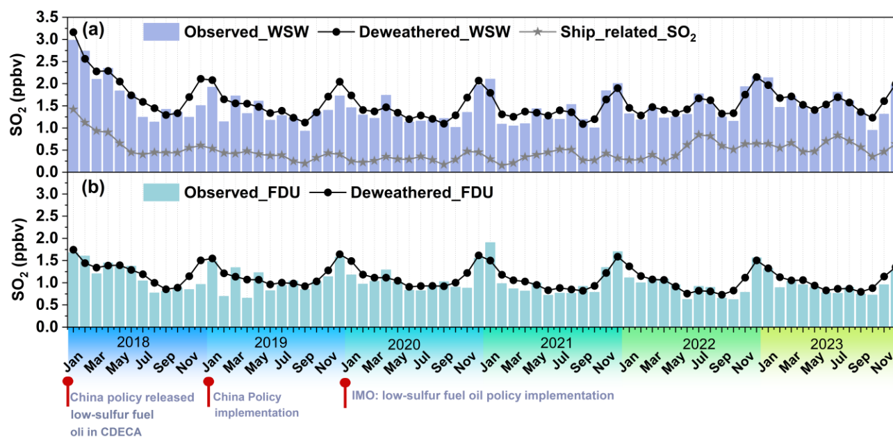
Figure 4: Monthly observed SO 2 concentrations based on DOAS and deweathered SO 2 after weather normalization in WSW and FDU, and ship_related_SO 2 contributions during 2018-2023. (a) The light purple bars represent the monthly average observed SO 2 concentration at WSW; The solid black circles represent the deweathered SO 2 concentration at WSW after removing meteorological influences. The gray star symbols indicate the monthly average contribution of ship_related_SO 2 . (b) The light blue bars represent the monthly average observed SO 2 concentration at FDU; The solid black circles represent the deweathered SO 2 concentration at FDU removing meteorological influences.
