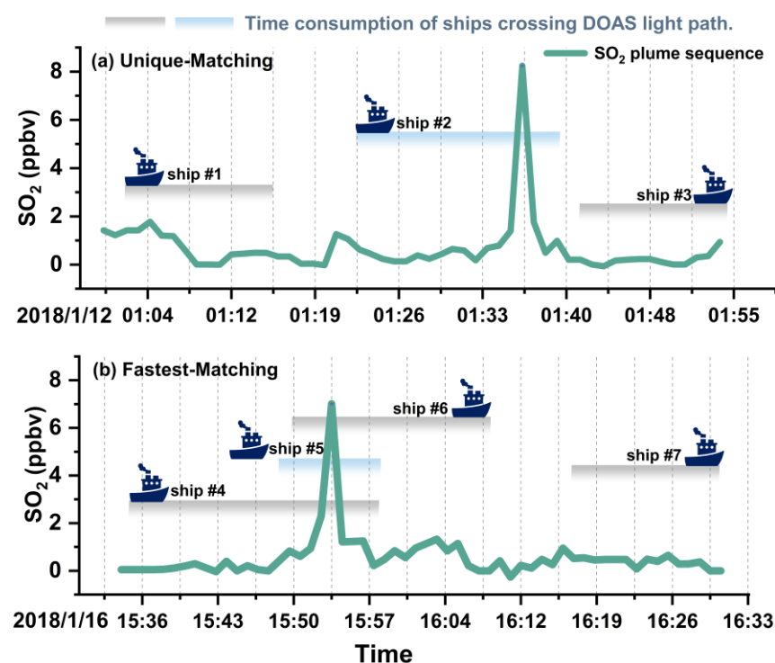
285 Figure 7: Illustration of two Matching-datasets for associating SO 2 -rich plumes with AIS ship activities. (a) Unique-Matching, where only plumes observed during the passage of a single ship (ship #2) near the DOAS light path are considered; and (b) Fastest-Matching, where plumes are matched to the ship (ship #5) with the shortest crossing time.
