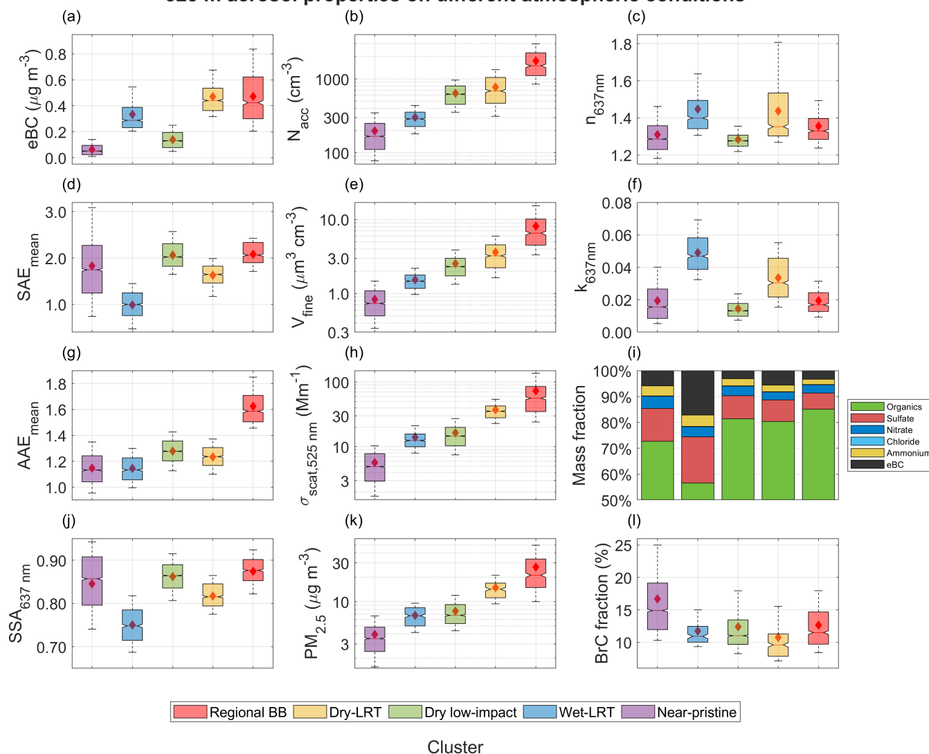
Figure 3. Box plots for the measured variables at the 325 m height when separated by the identified clusters, ordered from 1 to 5. The whiskers extend to the 10 th and 90 th percentiles, and the mean values are indicated with a red diamond. In (a) the eBC concentration, in (d) the SAE, and in (g) the AAE are the clustering seed variables. In (b) the accumulation mode particles, in (e) the fine mode volume, in (h) the scattering coefficient, and in (k) the \text{PM}_{2.5} mass are the extensive variables. In (c) and (f), the real and imaginary parts of the refractive index, respectively, in (i) the chemical composition, in (j) the SSA, and in (l) the BrC fraction are the other intensive properties. Note that the chemical composition fractions are shown from 50 to 100% to facilitate the visualization of more minor differences due to the strong organic aerosol dominance.
