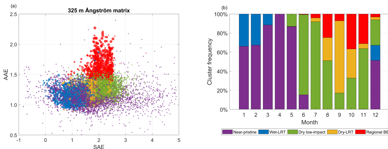
Figure 2. Results for the clustering analysis of the aerosol optical properties at 325 m, using the k-means algorithm with 5 clusters and the binary season separation. In panel (a), the Ångström matrix shows the distribution of clusters, with the point size indicating the equivalent black carbon concentration. Panel (b) shows the annual cycle of the cluster frequencies.
