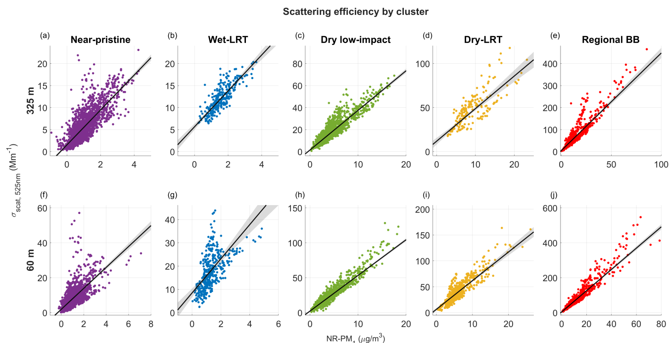
Figure 6. Scatter plots of non-refractive PM_1 mass and scattering coefficient at 525 nm measured at 325 m (a-e) and 60 m (f-j) for each cluster, with linear fit. The shaded areas indicate the 95% confidence interval.
